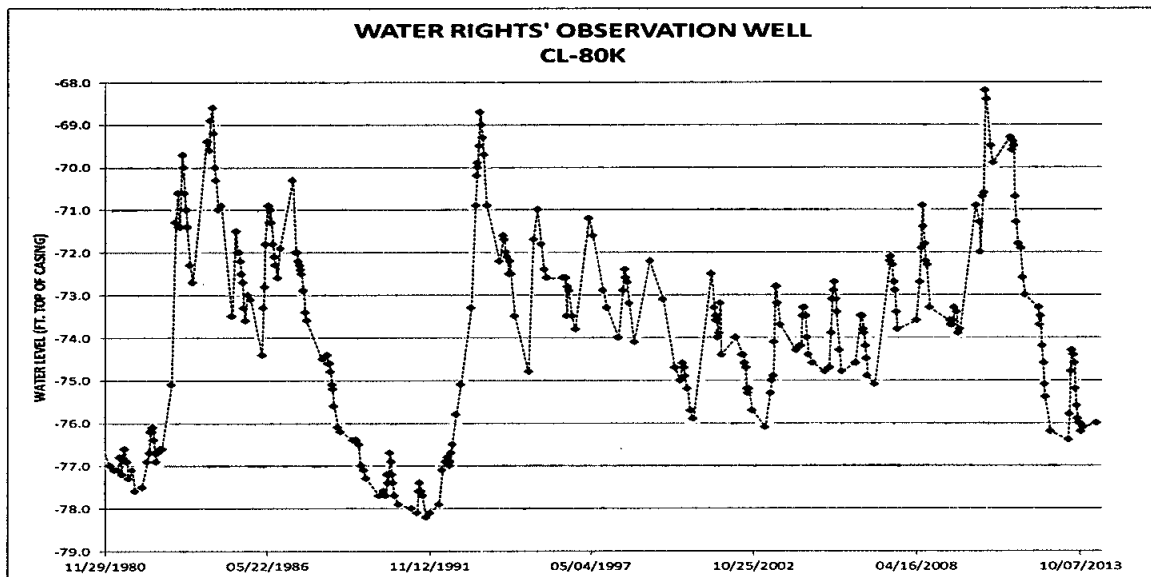
Figure 2- Hydrograph for observation well CL-80K (Water Rights, 2014a)
