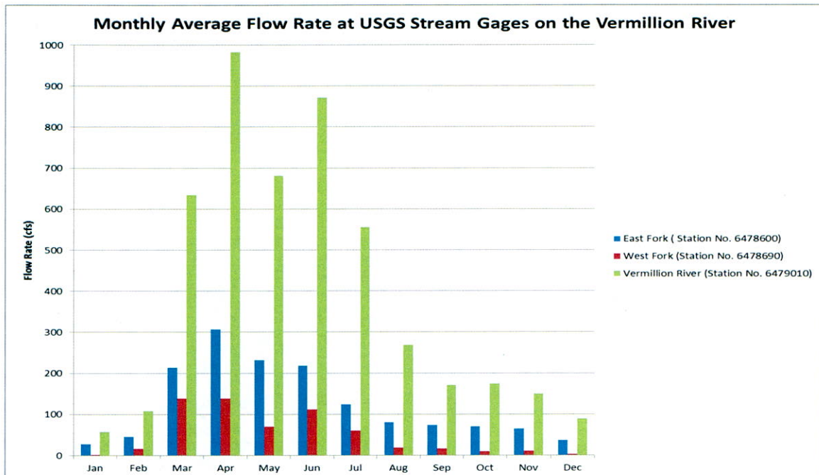
Figure 4- Monthly average flow rate at USGS stream gages on the Vermillion River (USGS, 2014)
