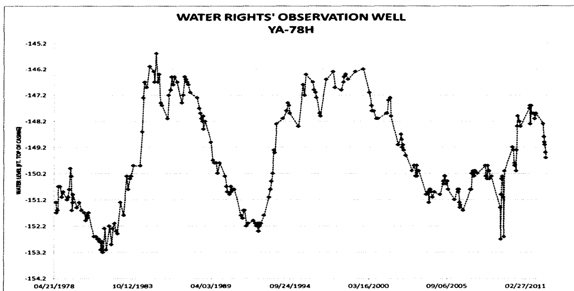
Figure 1- Hydrograph of DENR-Water Rights' observation well YA-78H, located approximately 0.42 miles northeast of the proposed well location (Water Rights, 2012a)
