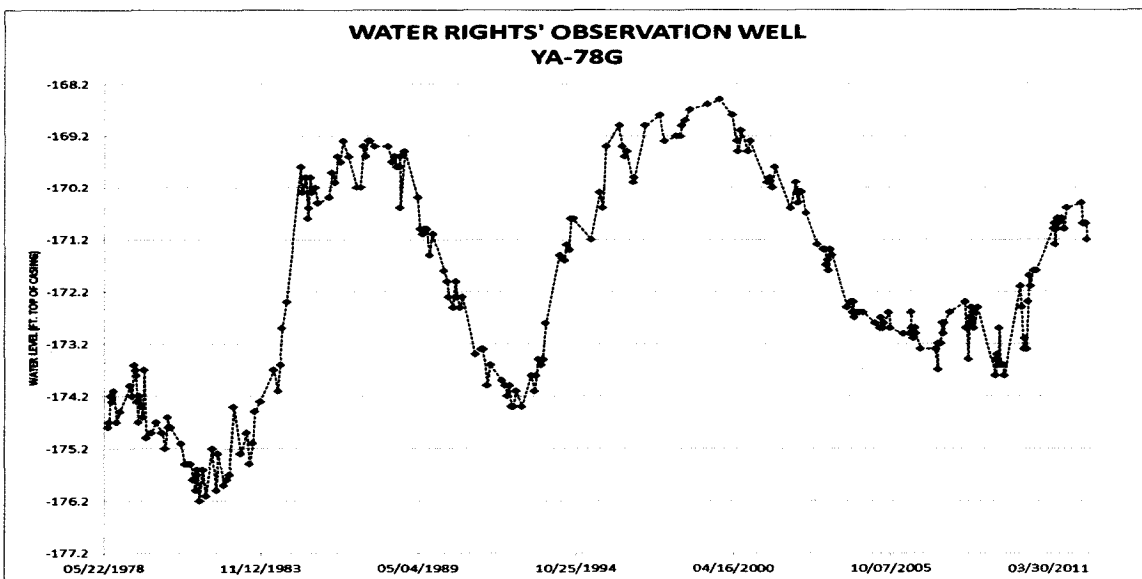
Figure 3- Hydrograph of DENR-Water Rights' observation well YA-78G, located approximately 1.56 miles west-northwest of the proposed well location (Water Rights, 2012a)
