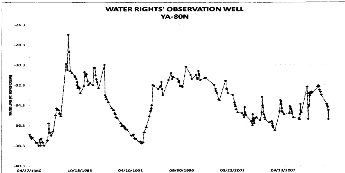
Figure 2- Hydrograph of DENR-Water Rights' observation well YA-80N, located approximately 1.47 miles north-northeast of the proposed well location (Water Rights, 2012a)
