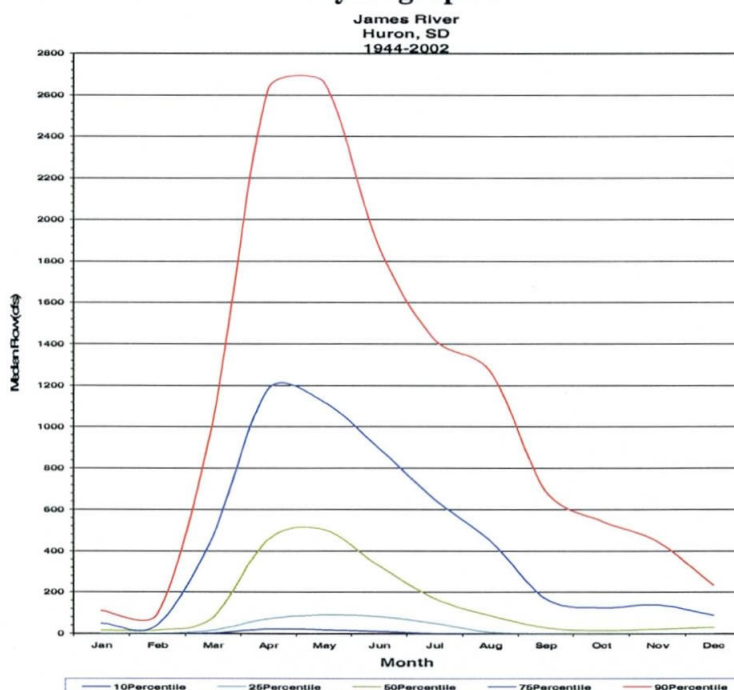
Hydrograph 2
