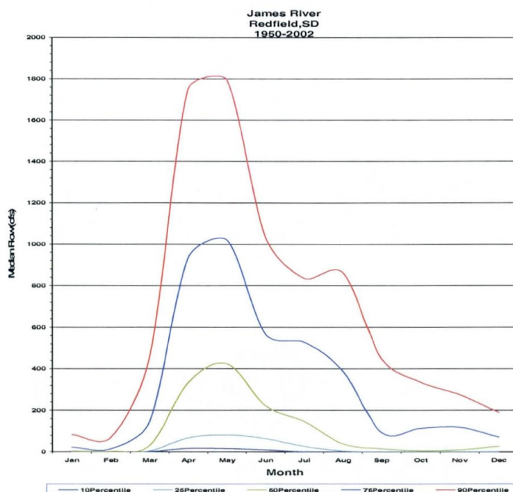
Hydrograph 1
