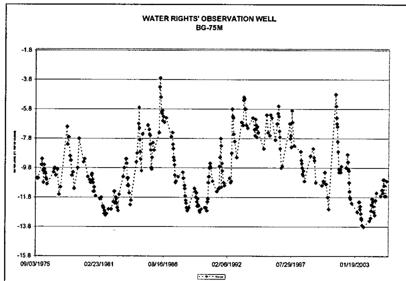
Figure 1. Hydrograph of observation well BG-75M.
