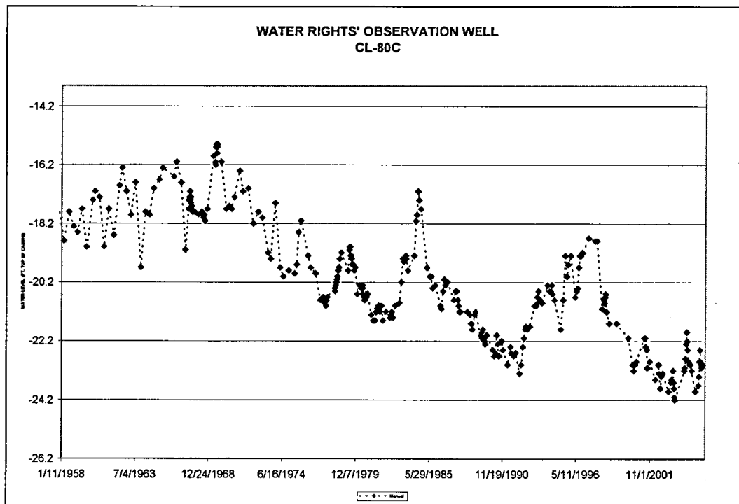
Figure 1. Hydrograph of observation well CL-80C.
