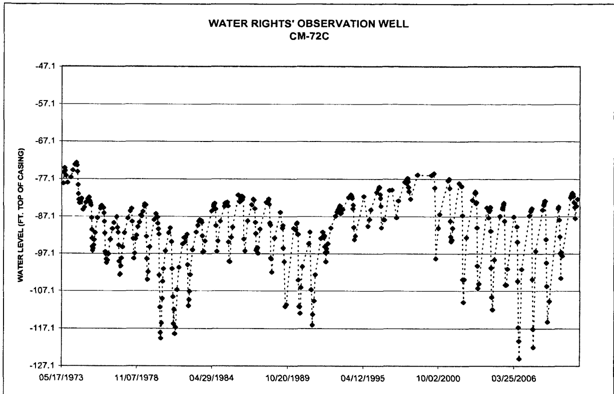
Figure 1. Hydrograph for Water Rights Observation Well CM-72C, completed into the Choteau:West Aquifer within two miles of 6599A-3
