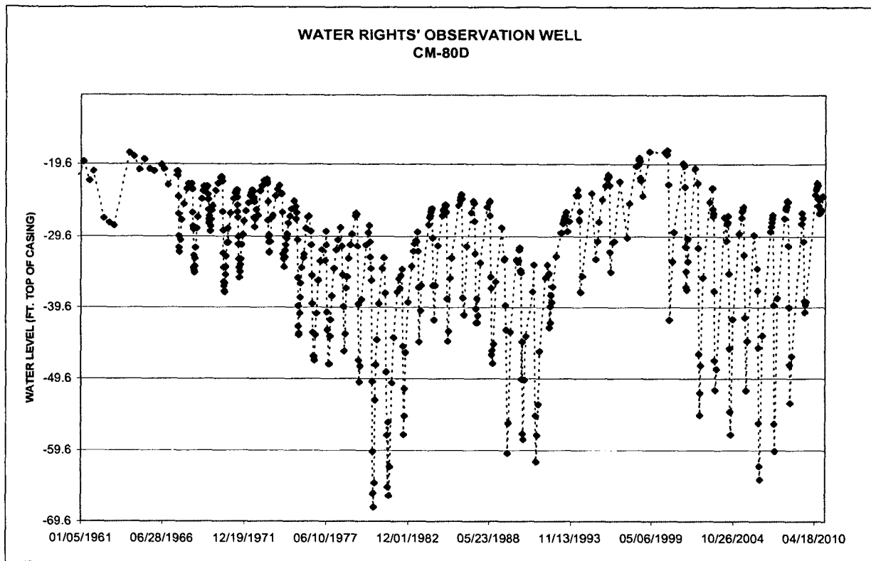
Figure 3. Hydrograph for Water Rights Observation Well CM-80D, completed into the Choteau:West Aquifer just over a mile west of 6599A-3
