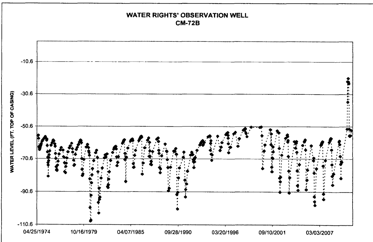
Figure 2. Hydrograph for Water Rights Observation Well CM-72B, completed into the Choteau:West Aquifer within two miles of 6599A-3
