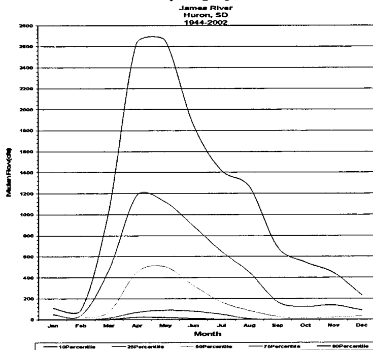
Hydrograph 2
