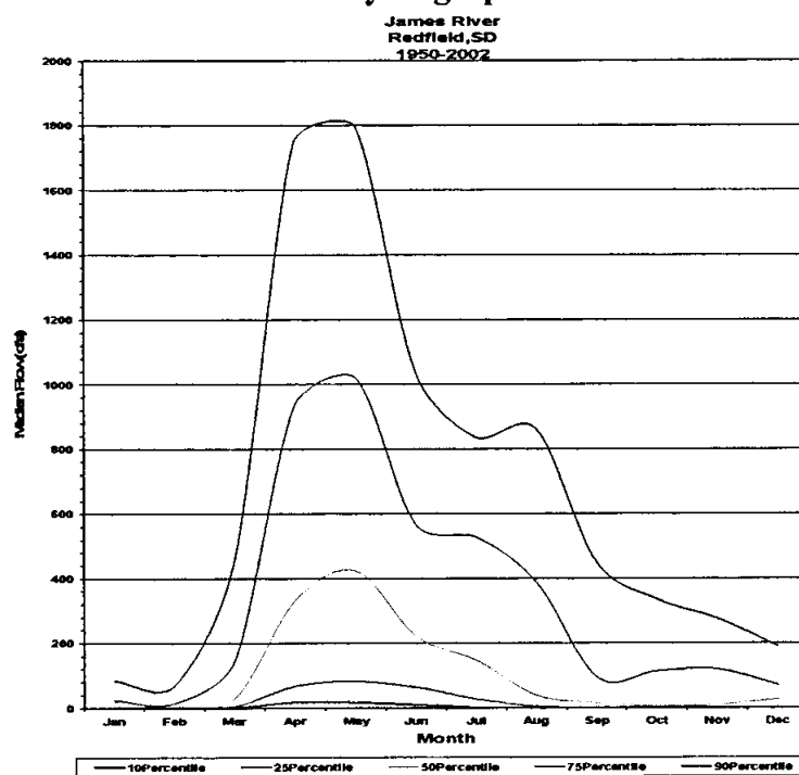
Hydrograph 1
