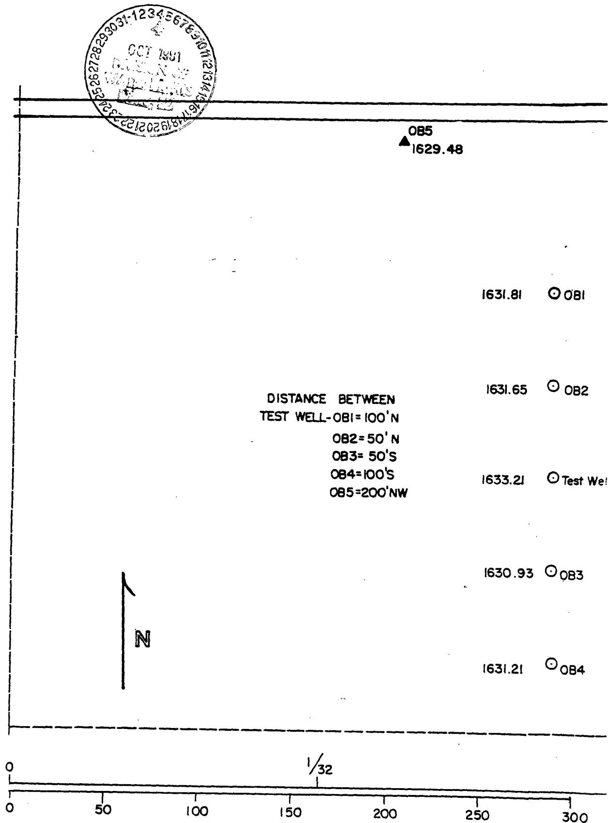
FIGURE 3-- Well configuration and elevations at the Brookings-Deuel rural water system test site, NE \frac{1}{4} , NE \frac{1}{4} , NE \frac{1}{4} , NE \frac{1}{4} , SEC. 25, T. 112N; R. 51 W; Brookings county, South Dakota.
