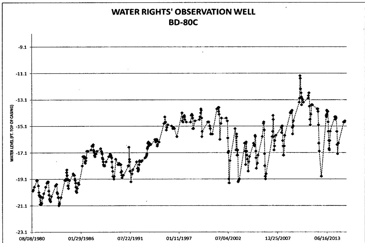
Figure 2. Hydrograph for DENR-Water Rights' observation well completed into the Tulare: Western Spink/Hitchcock aquifer approximately one-half of a mile northwest of the wells that supply water for Water Right No. 3317A-3.
