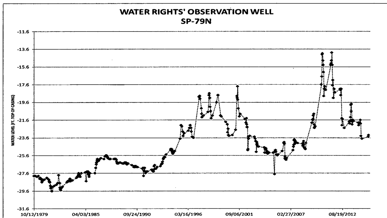
Figure 2. Hydrograph for DENR-Water Rights' observation well completed into the Tulare: Western Spink/Hitchcock aquifer approximately three-fourths of a mile northeast of the wells that supply water for Water Right No. 4794-3.
