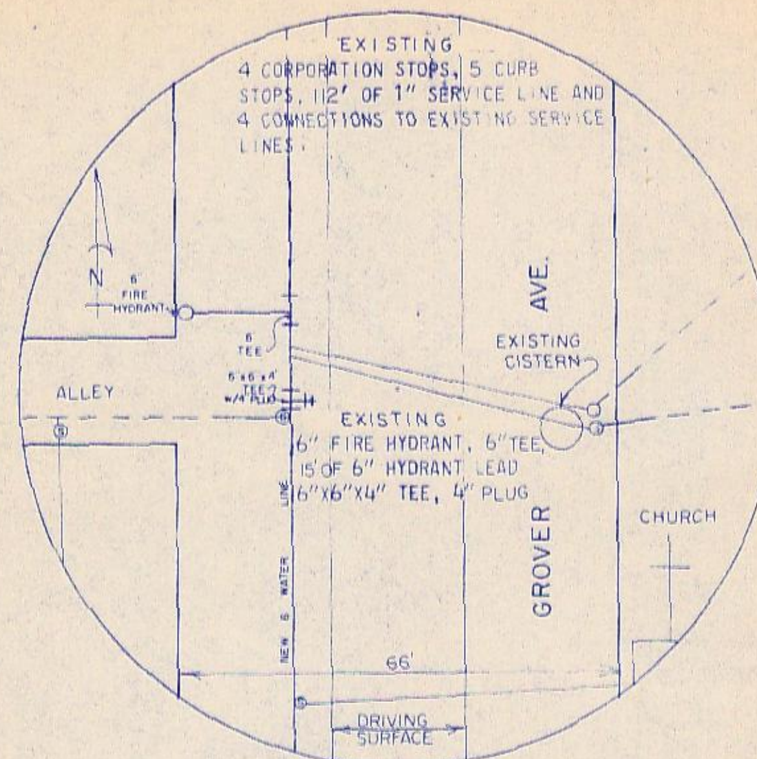
DETAIL FOR AREA 2
