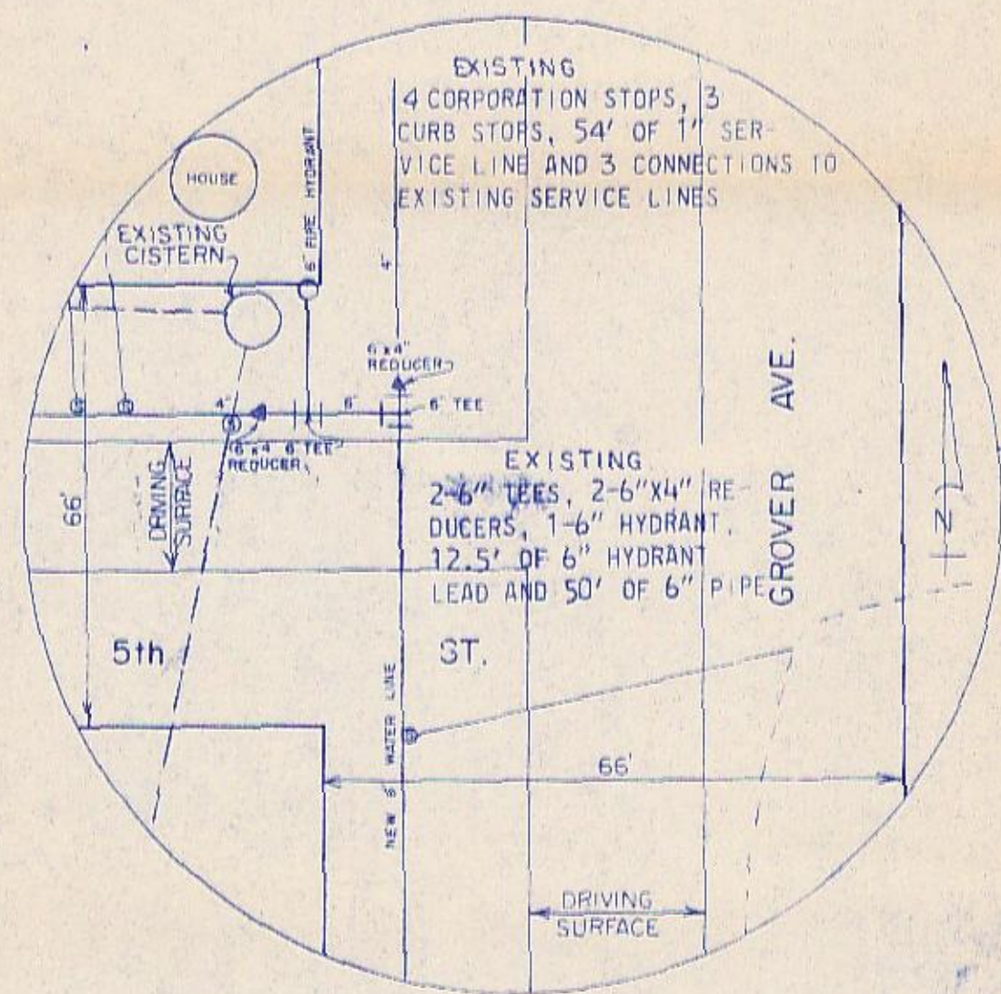
DETAIL FOR AREA 3
