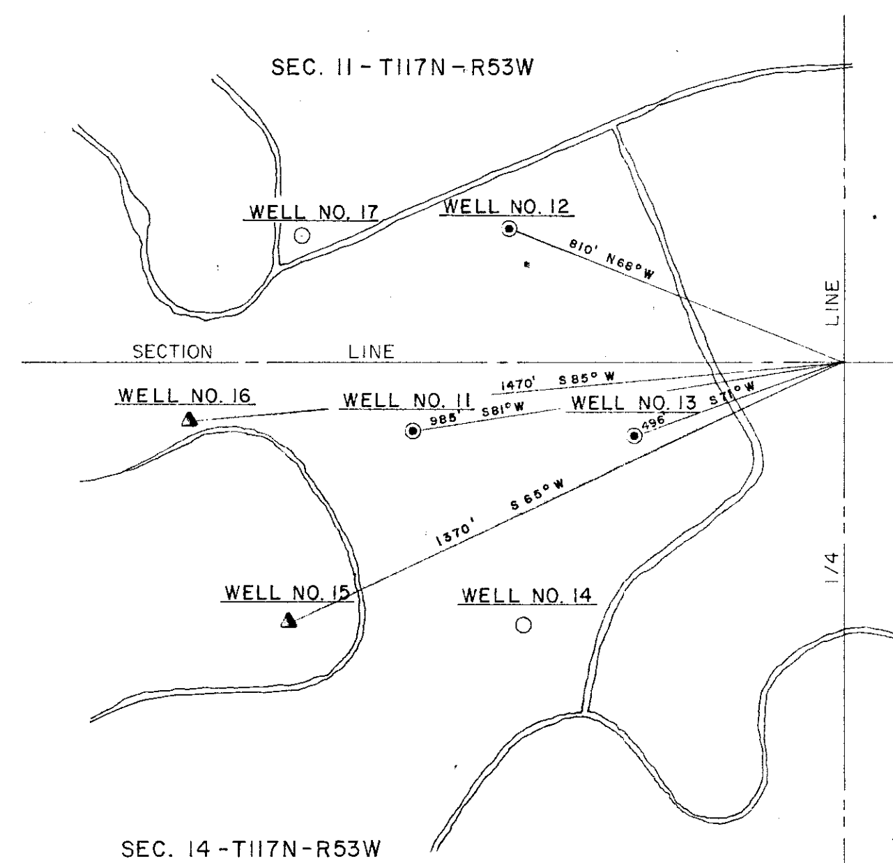
DETAIL "A" SCALE 1" = 300'
