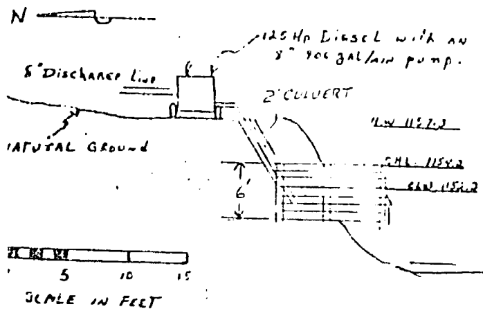
Elevation View
