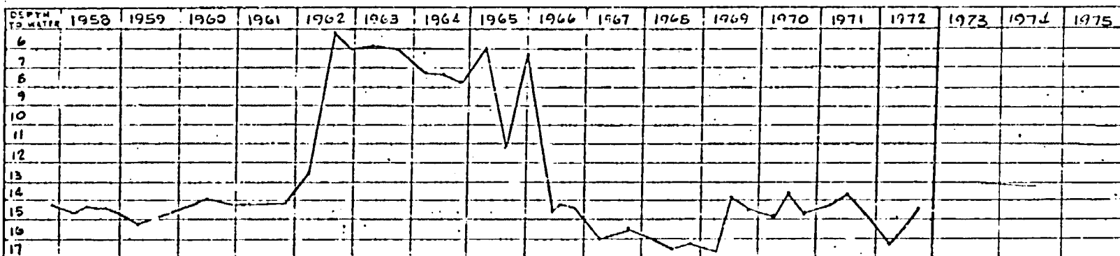
Observation Well C1. Graph Of Annual Water Level Measurements
