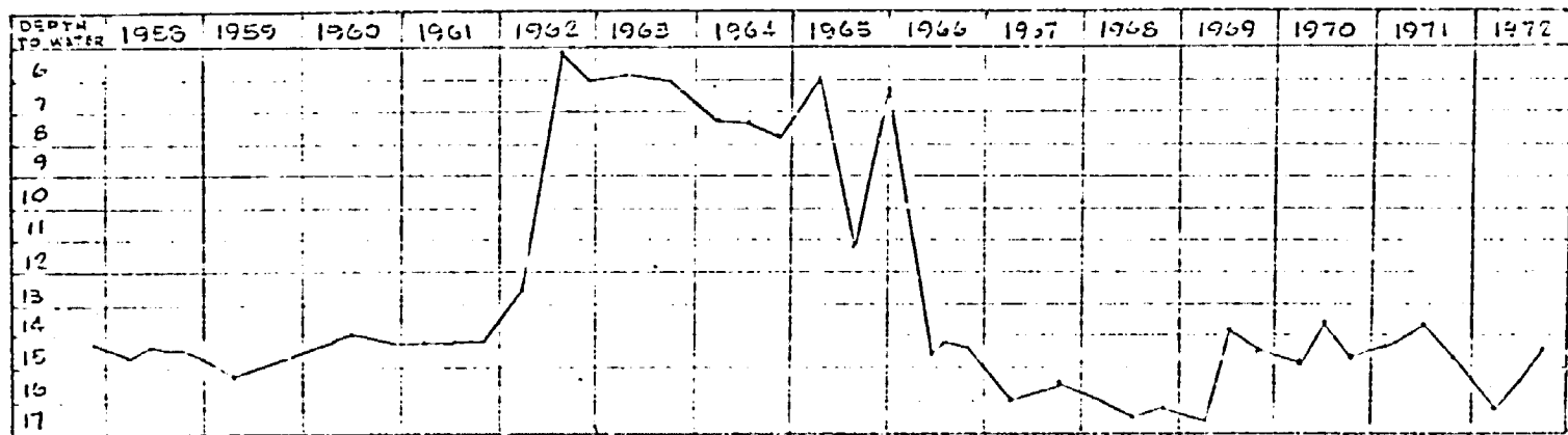
Observation Well C1. Graph Of Annual Water Level Measurements
