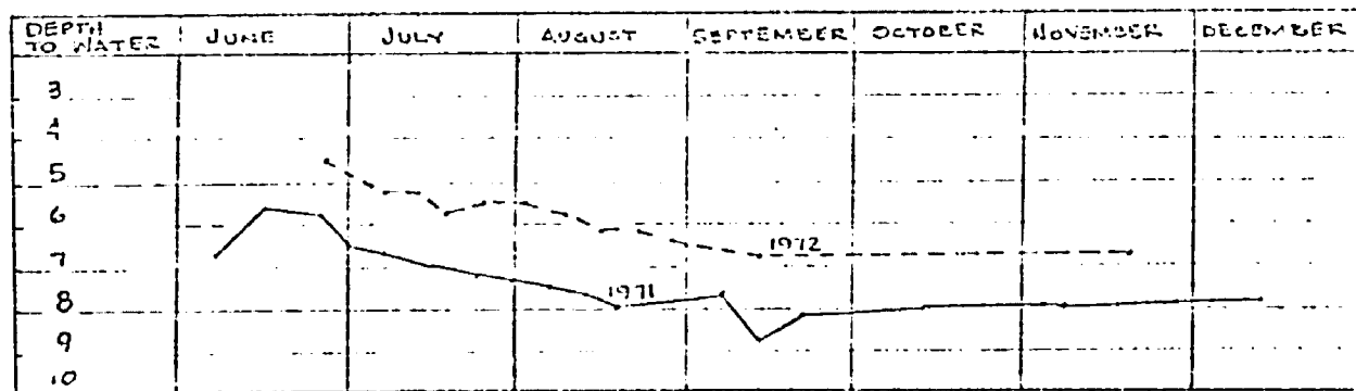
Observation Well JS. Graph of 1971 & 72 Water Level Measurements During Irrigation Season
