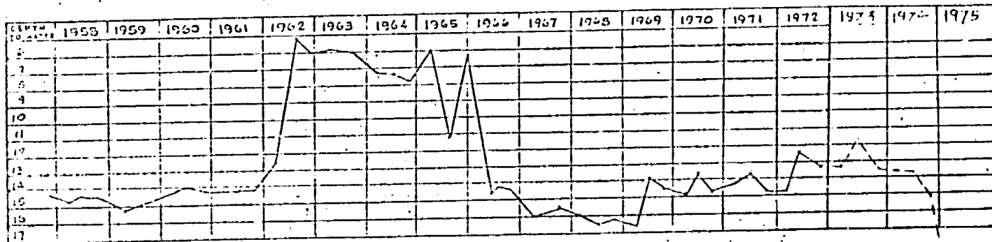
Observation Well C1. Graph Of Annual Water Level Measurements
