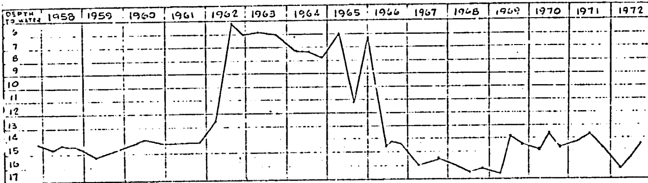
Observation Well C1. Graph Of Annual Water Level Measurements
