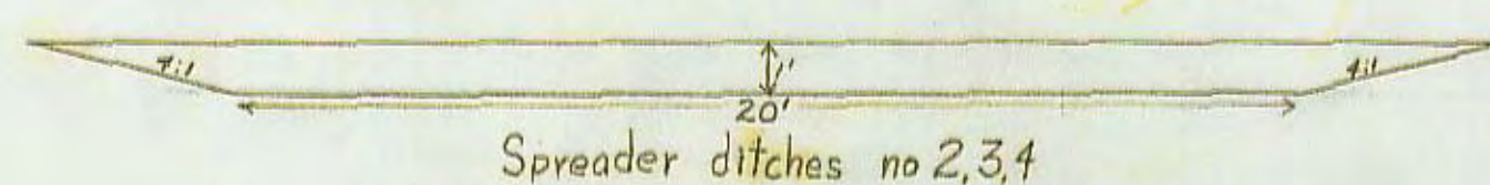
TYPICAL X-SECTIONS OF DIKES AND DITCHES SCALE: 1" = 4'
