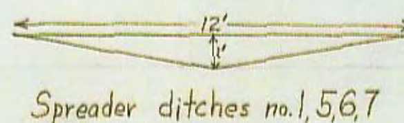
TYPICAL X-SECTIONS OF DIKES AND DITCHES SCALE: 1" = 4'
