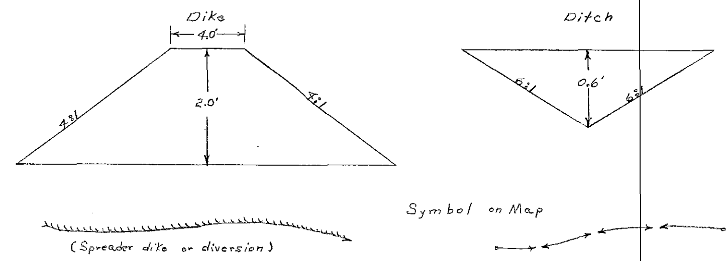
TYPICAL CROSS-SECTIONS
