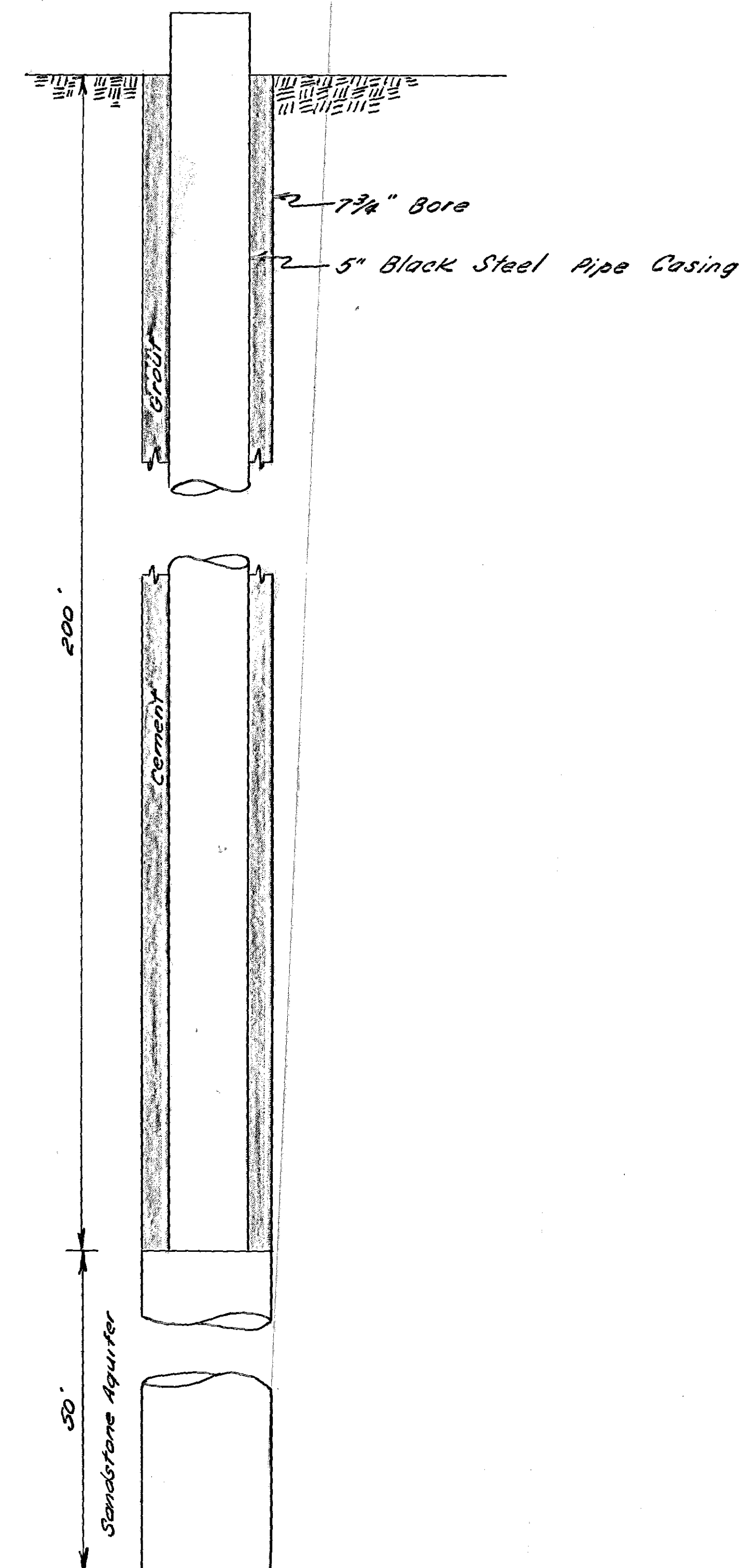
TYPICAL WELL DETAILS No Scale
