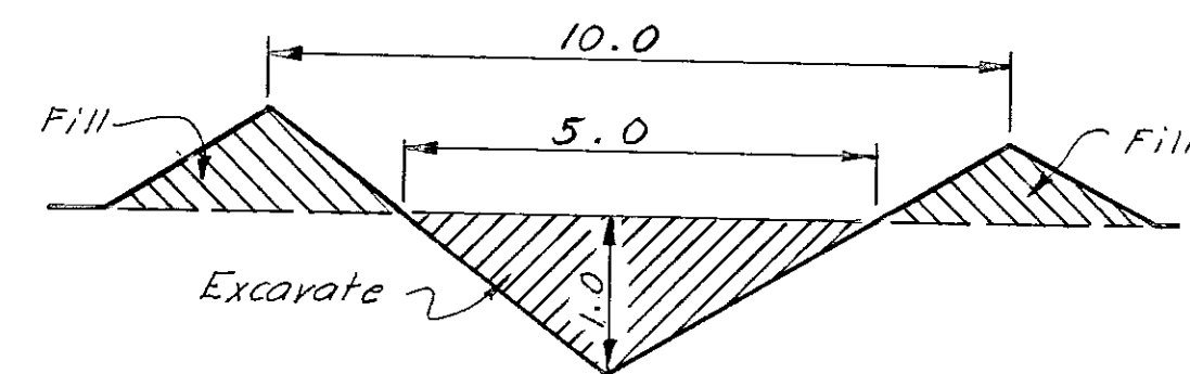
TYPICAL DITCH SECTION
