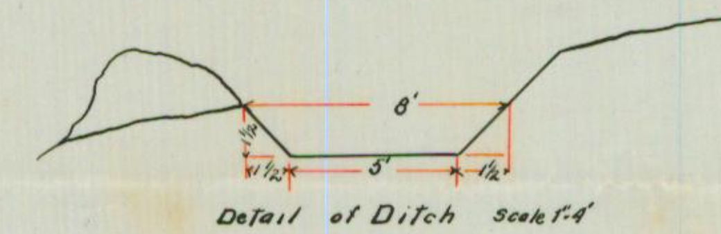
Detail of Ditch Scale 1"=4'
