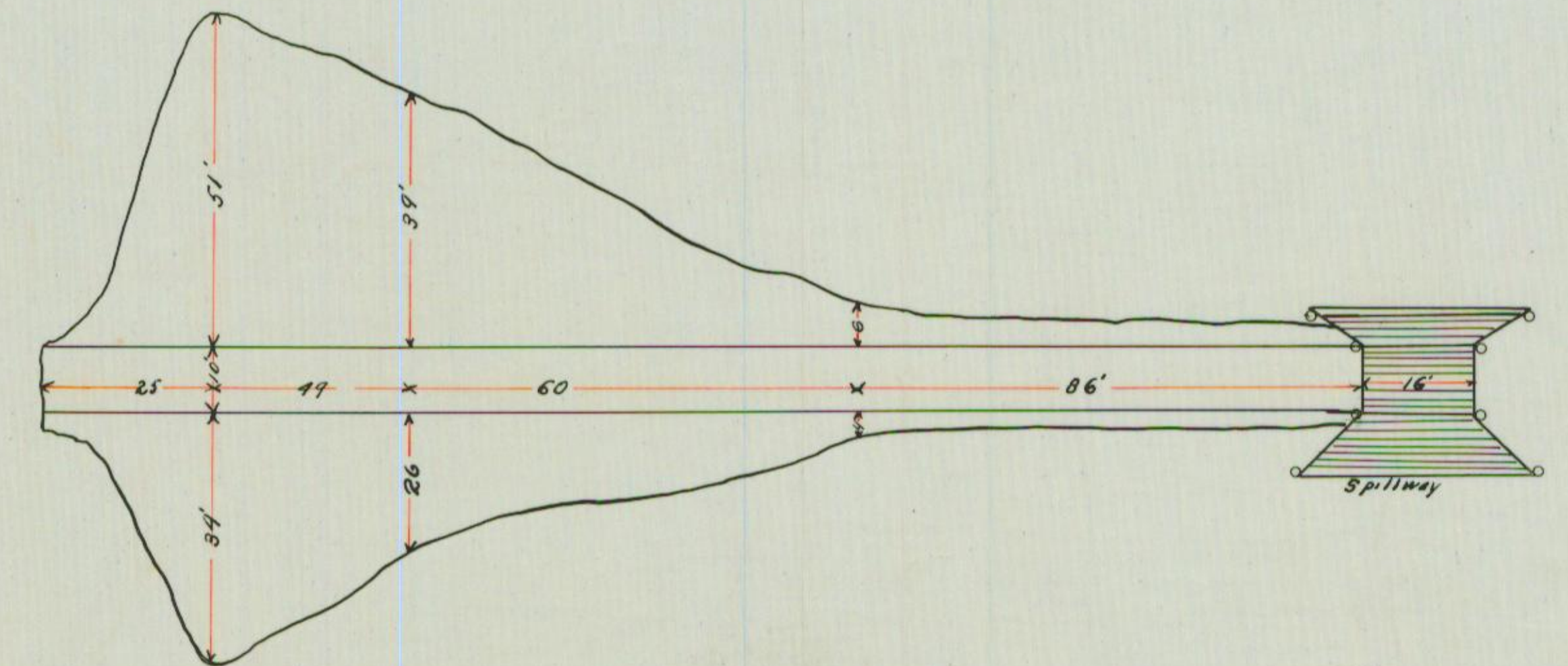
Plan of Dam Scale 1"=20'
