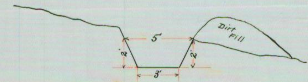
Section of Ditch Scale 1" = 4'
