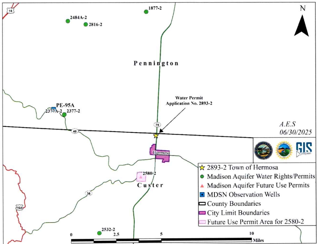
Figure 4. Approximate location of the proposed diversion for Application No. 2893-2, and the nearby Madison aquifer observation wells, water rights/permits, and future use permits (Water Rights, 2025b and 2025c)
