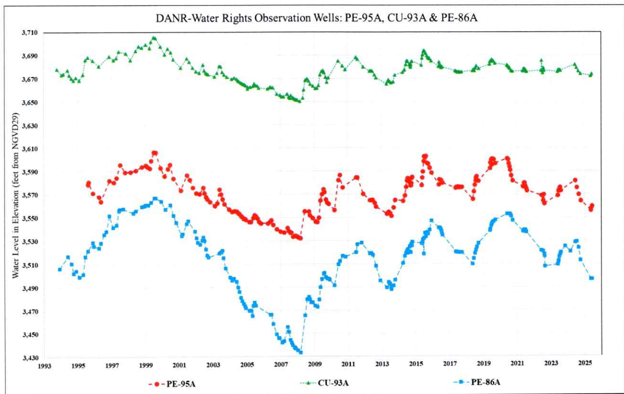
Figure 3. A graph showing the elevation of water levels for observation wells: PE-95A, CU-93A & PE-86A (Water Rights, 2025b)
