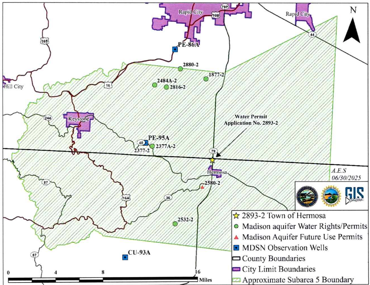
Figure 2. Subarea 5 used for the Madison and Minnelusa aquifers localized hydrologic budgets (modified from Carter et al., 2001b), the location of the proposed diversion point for Water Permit Application No. 2893-2, the Madison aquifer water rights/permits, and observation wells within Subarea 5 (Water Rights, 2025b and 2025c)
