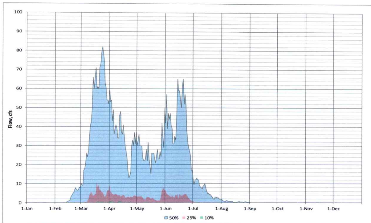
Figure 1. Percentile streamflow hydrograph for the stream gaging station USGS No. 06441500, Bad River near Ft Pierre; 1928-2022 (USGS. 2023).
