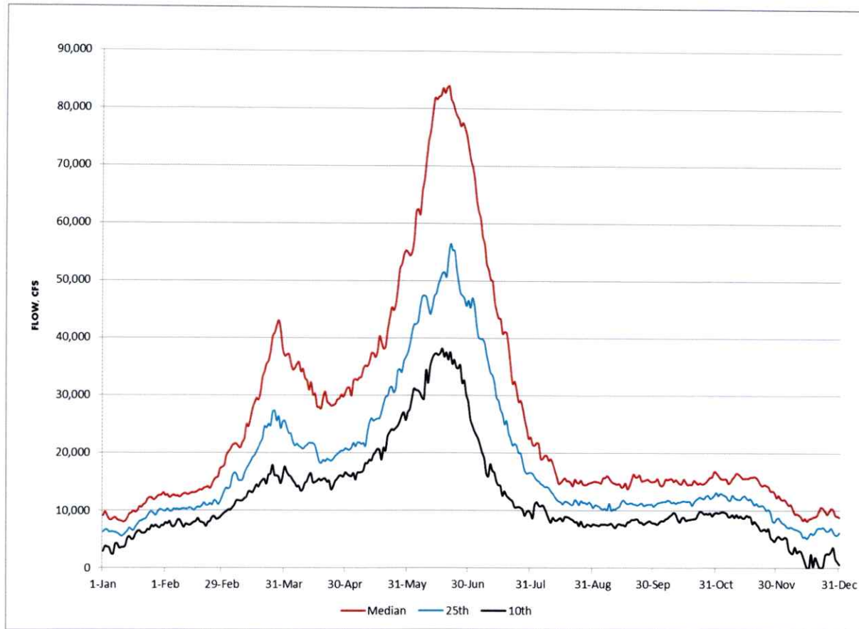
Figure 2. Natural flow hydrograph for the Missouri River at Oahe Dam (Jacobson, 2001).
