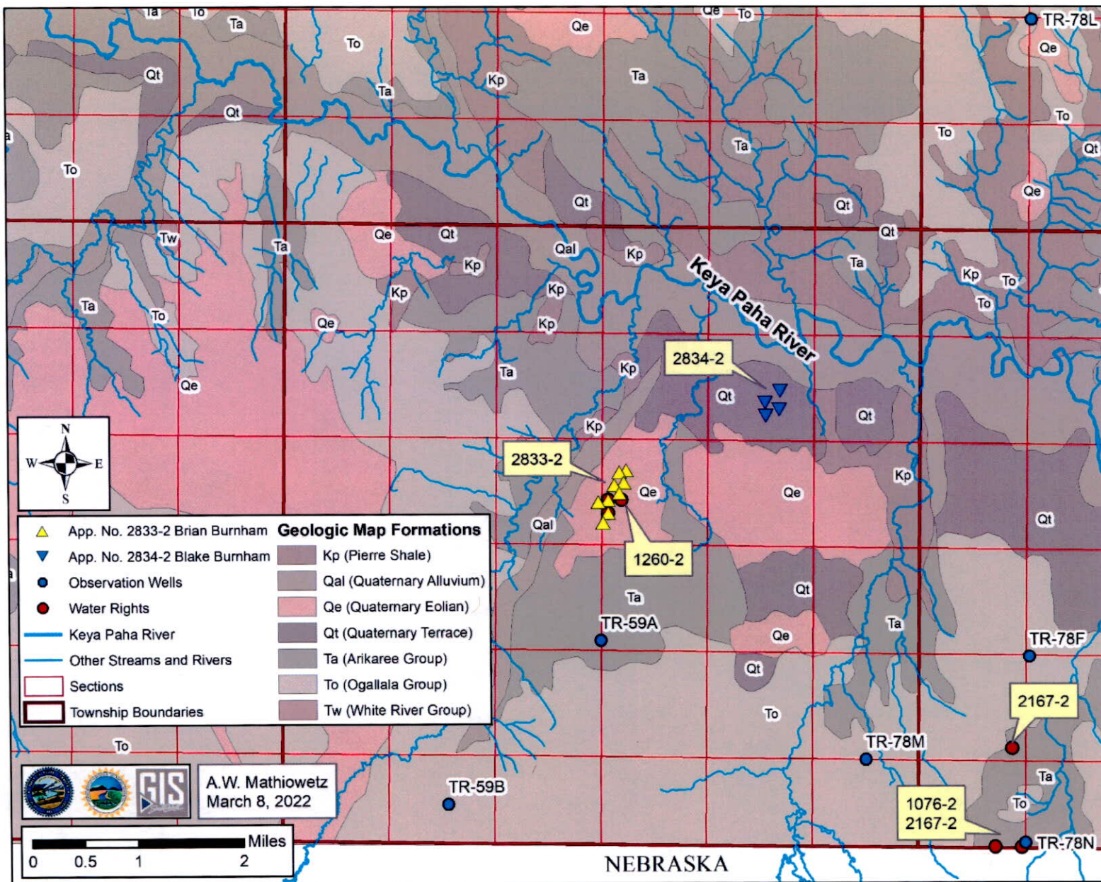
Figure 1- Geologic formations map (modified from: Martin et al, 2004) with groundwater water rights (Water Rights, 2022d), Ogallala aquifer observation wells (Water Rights, 2022c) and local streams and rivers
