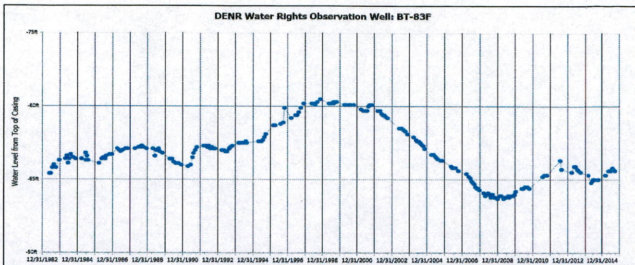
Figure 5. Hydrograph of Ogallala aquifer observation well, see Figure 1 for location.
