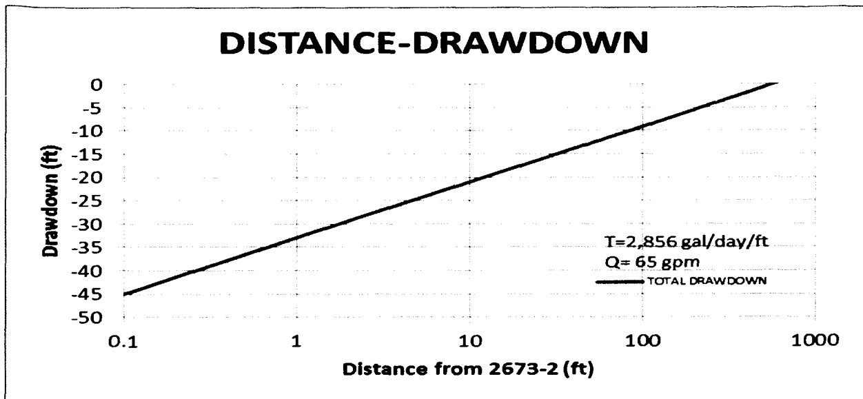
Figure 1. Distance-Drawdown plot for Water Permit Application No. 2673-3.
