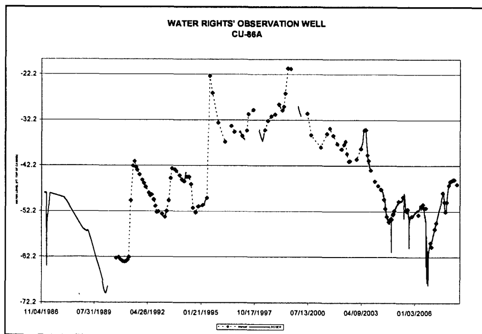
Figure 1: Monitoring well
