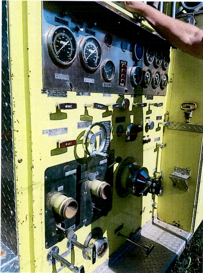
Pumper controls
