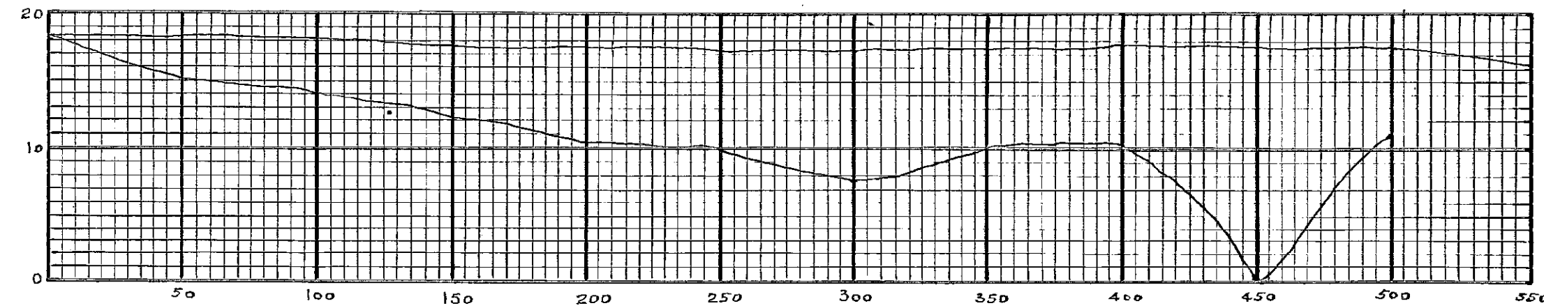
PROFILE OF DAM. SCALE VER.-1"=10FT. HOR.-1"=50FT.
