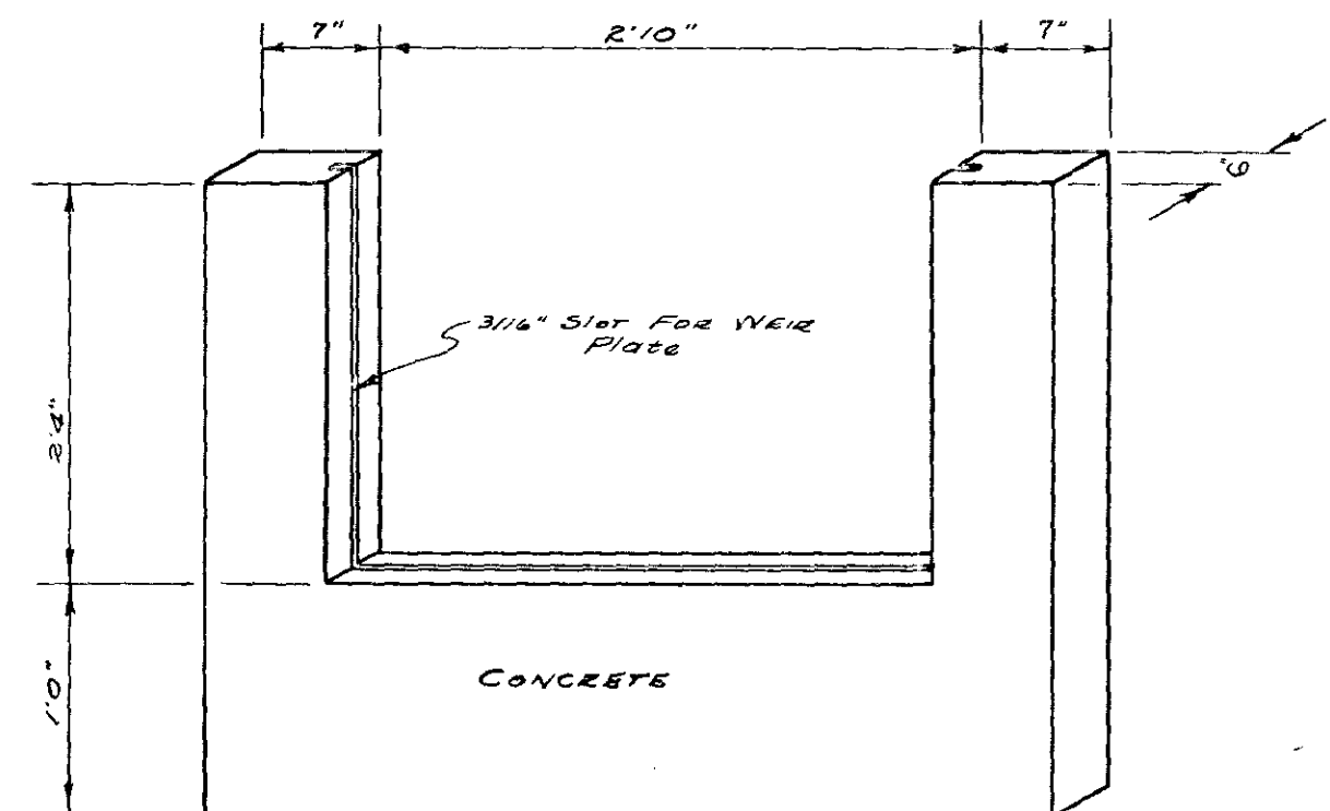
WEIR HEADWALL DETAIL (THREE TO BE BUILT)
