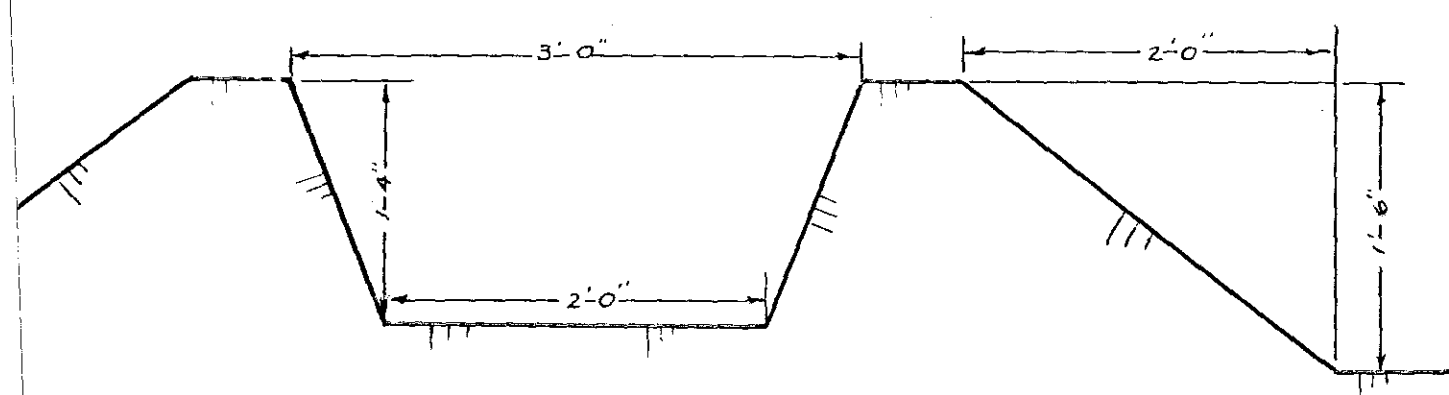
CROSS-SECTION LATERAL FIELD 4
