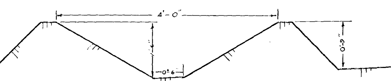
CROSS-SECTION LATERAL FIELD 1 & 2
