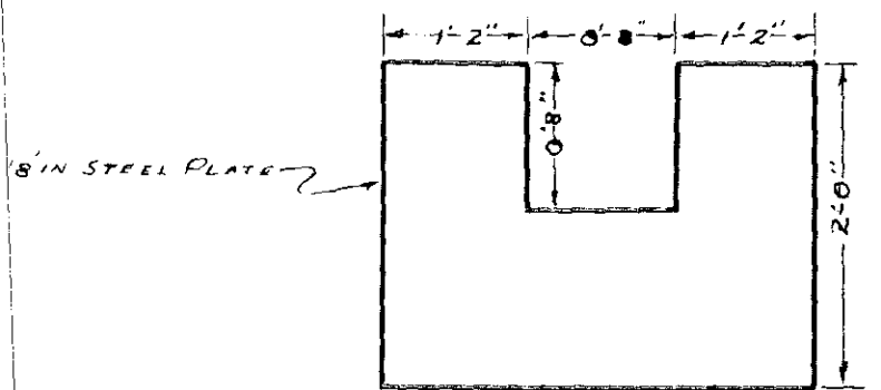
WEIR DETAIL
