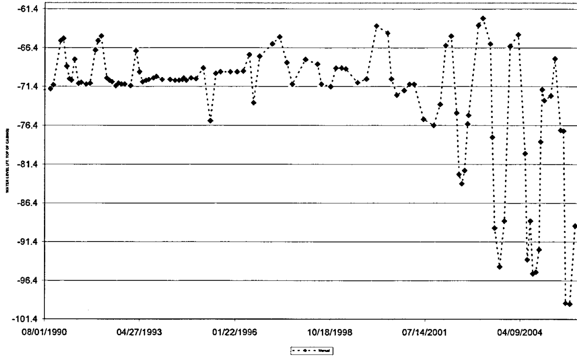
Figure 1. Hydrograph of Inyan Kara Observation Aquifer Well located approximately ten miles west of the 1857-1
