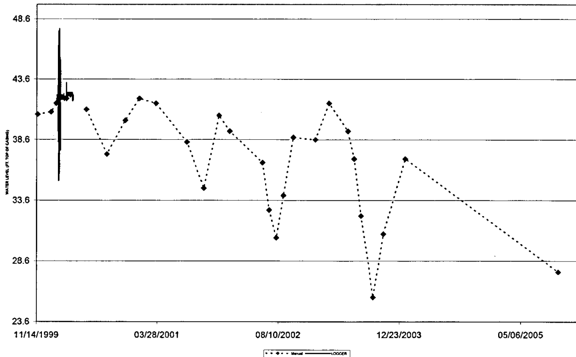
Figure 2. Hydrograph of Inyan Kara Observation Aquifer Well located approximately seventeen miles south of 1857-1
