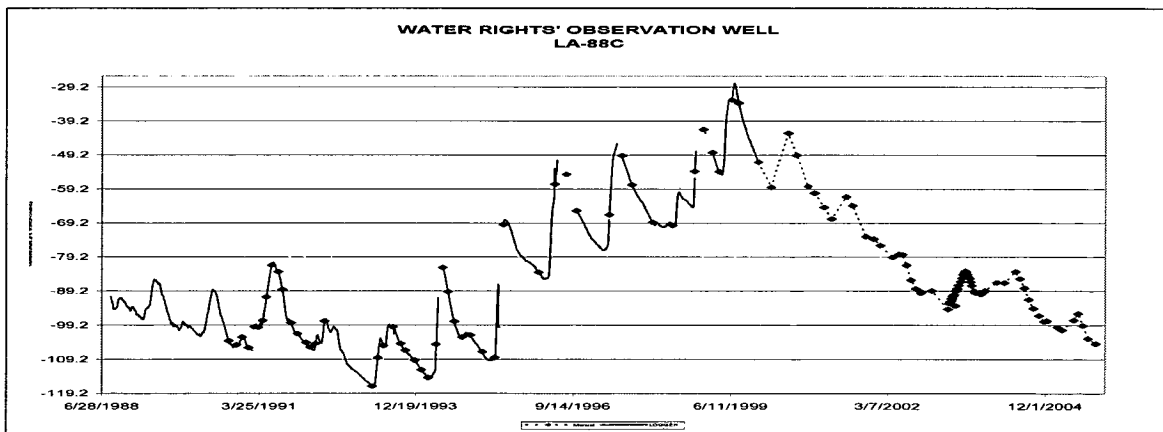
Figure 1. Hydrograph of observation well LA-88C.
