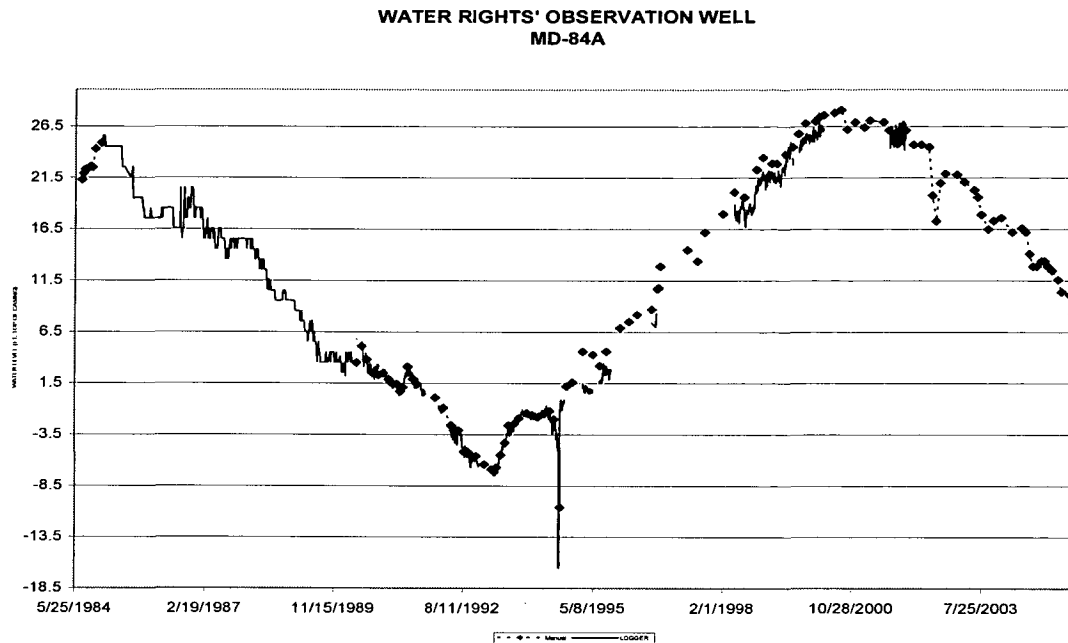
Figure 1. Hydrograph of Water Rights' Minnelusa aquifer Observation Well approximately one-half mile east of 1849-1
