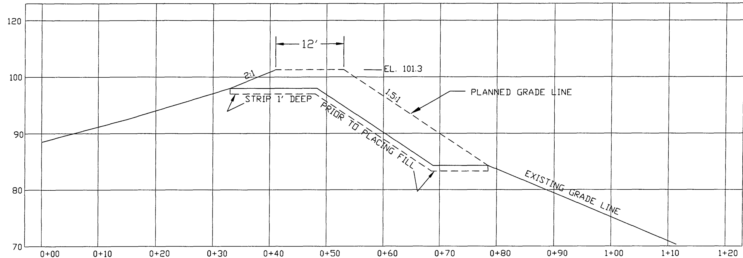
CROSS-SECTION A - A (DAM)
