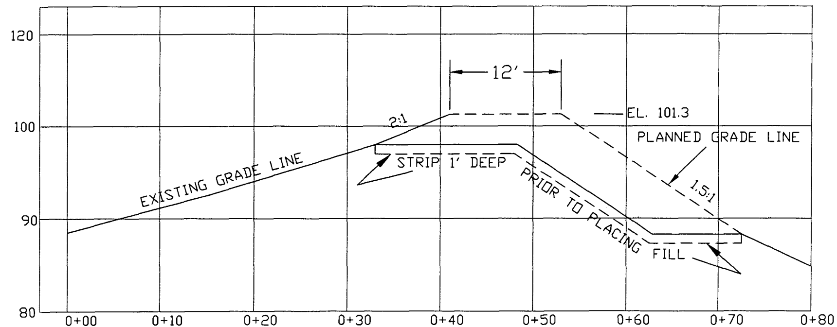
CROSS-SECTION B - B (DAM)
