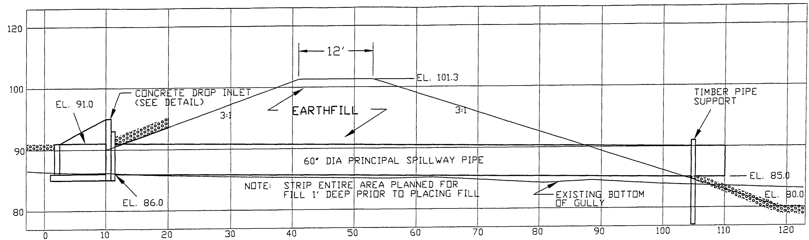
PROFILE & PRINCIPAL SPILLWAY
