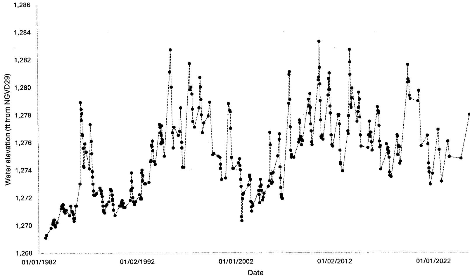
Figure 2: Hydrograph of Observation Well SP-82E [2]
