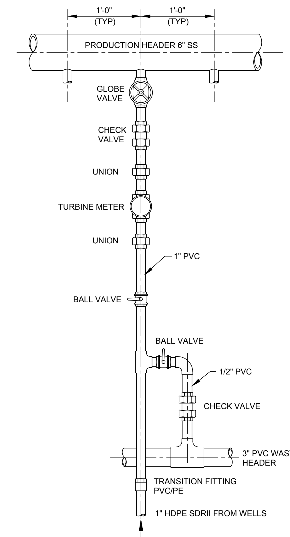
PRODUCTION HEADER DETAIL NTS
