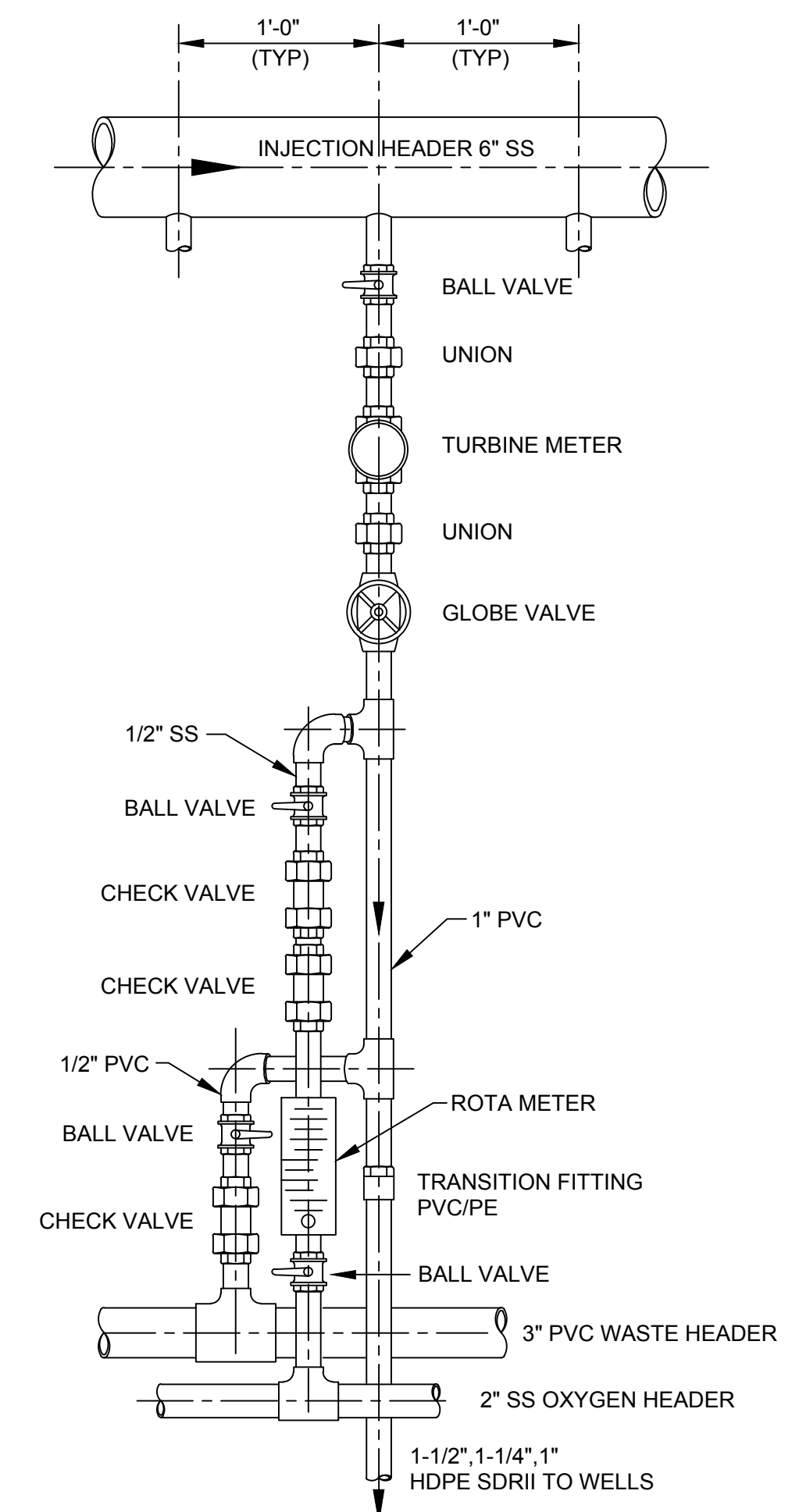
INJECTION HEADER DETAIL NTS
