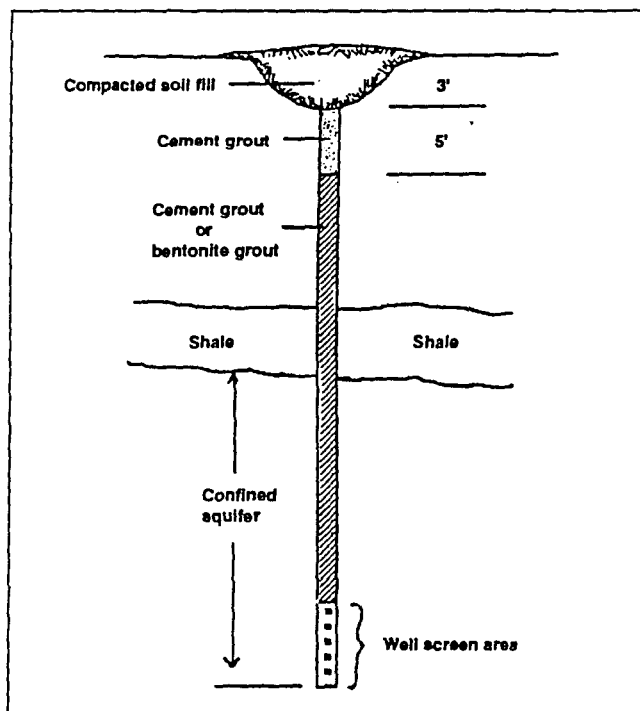
Figure 3. Plugging wells in confined aquifers.
