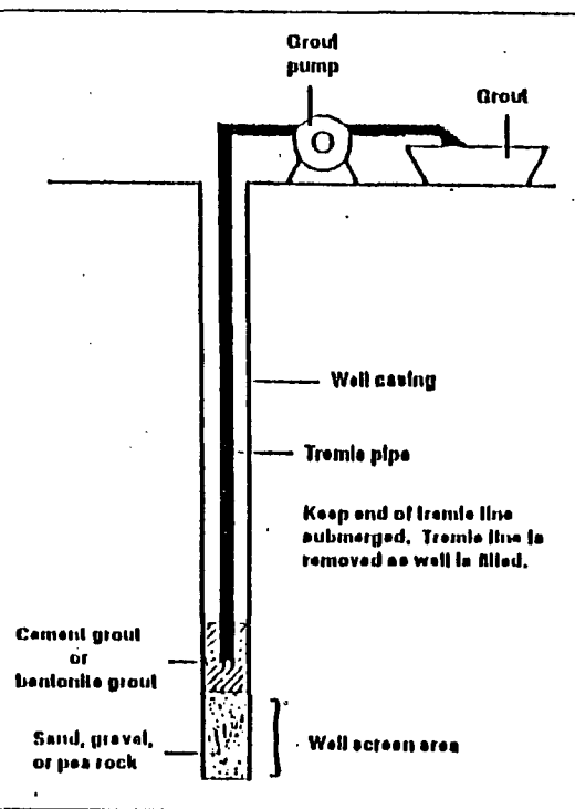
Figure 2. Pumping grout with a tremie pipe.
