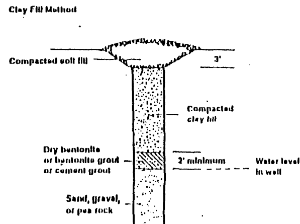
Figure 1. Plugging wells in unconfined aquifers.
