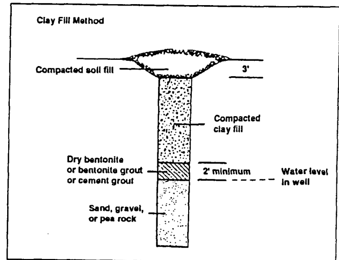
Figure 1. Plugging wells in unconfined aquifers.
