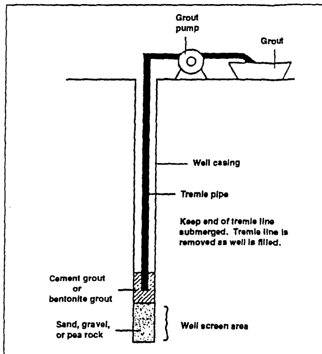
Figure 2. Pumping grout with a tremie pipe.
