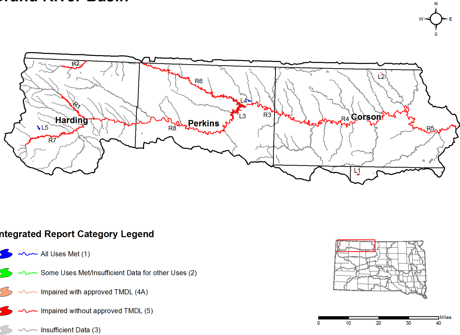
Figure 14: Grand River Basin
