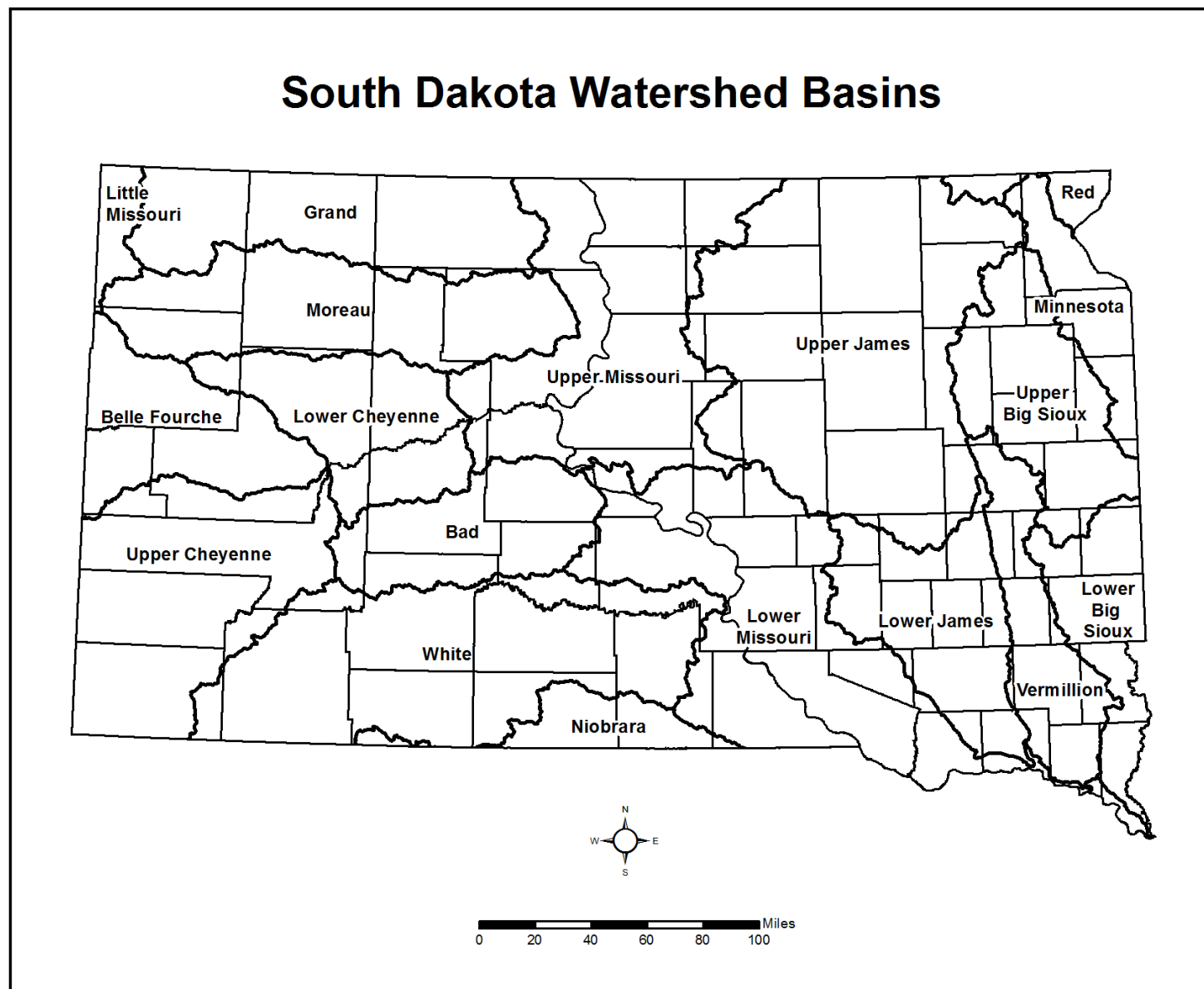
Figure 6: Major River Basins in South Dakota
