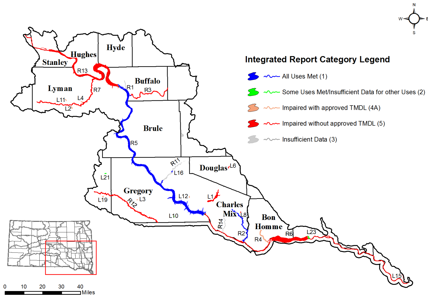
Figure 20: Lower Missouri River Basin
