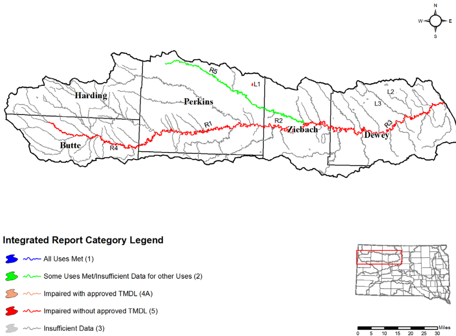
Figure 21: Moreau River Basin
