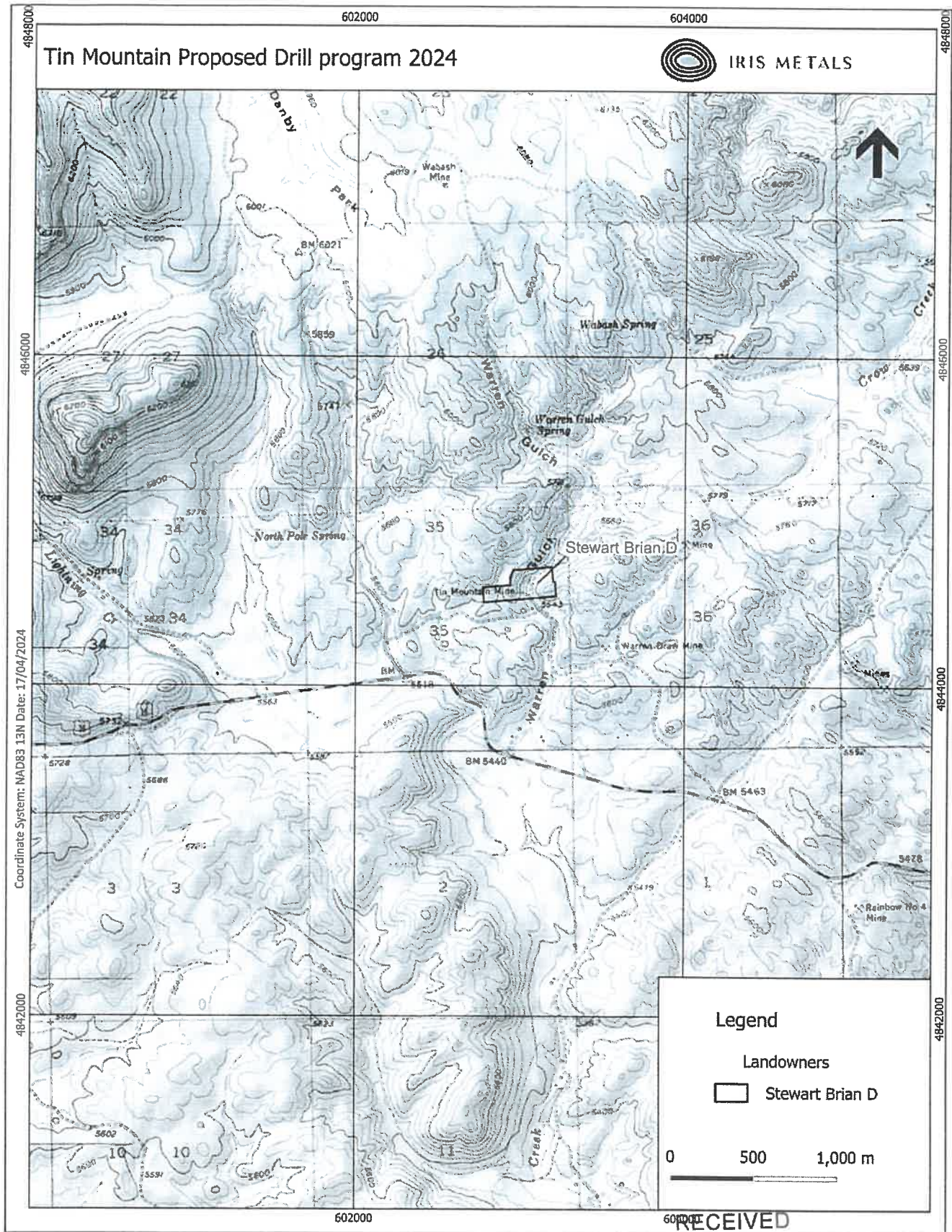
Figure 4: Proposed drilling location topographical plan. MAY 13 2024
