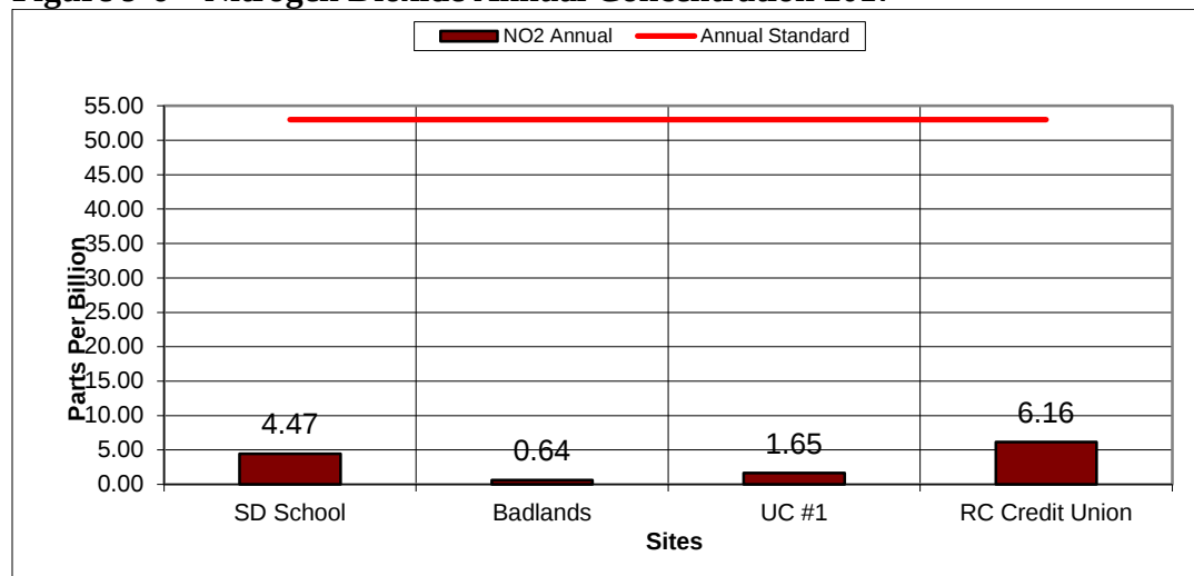
Figure 9-6 – Nitrogen Dioxide Annual Concentration 2017
