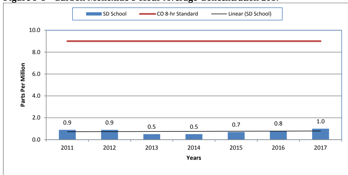
Figure 9-8 - Carbon Monoxide 8-Hour Average Concentration 2017
