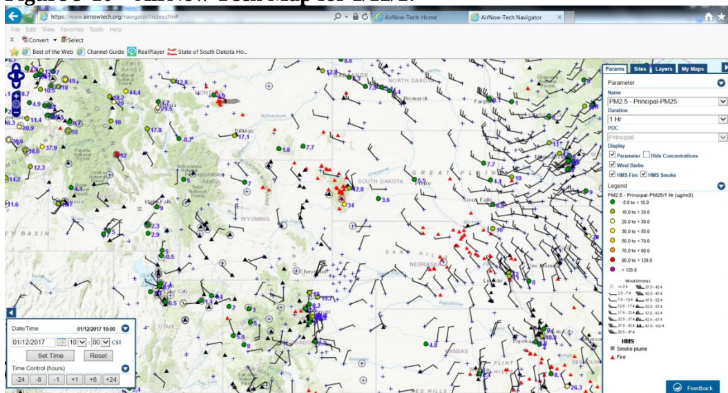
Figure 9-10 – AirNow Tech Map for 1/12/17
