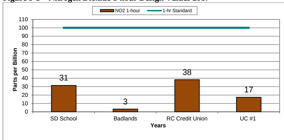
Figure 9-5 – Nitrogen Dioxide 1-hour Design Values 2017
