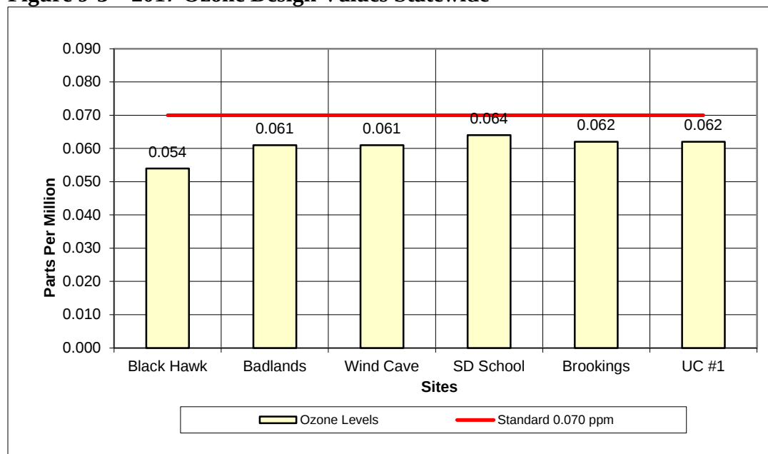
Figure 9-3 – 2017 Ozone Design Values Statewide
