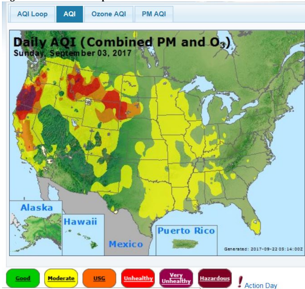
Figure 9-72 - AirNow Tech Map for 9/3/17
