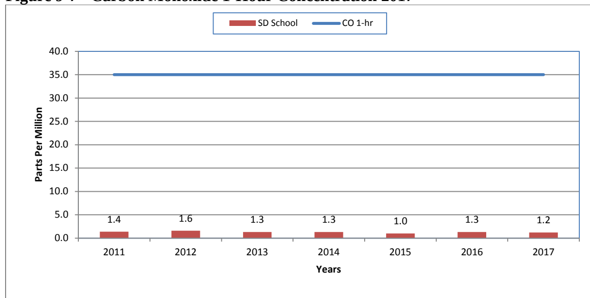
Figure 9-7 - Carbon Monoxide 1-Hour Concentration 2017
