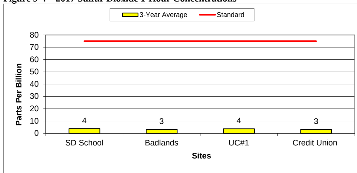
Figure 9-4 – 2017 Sulfur Dioxide 1-Hour Concentrations
