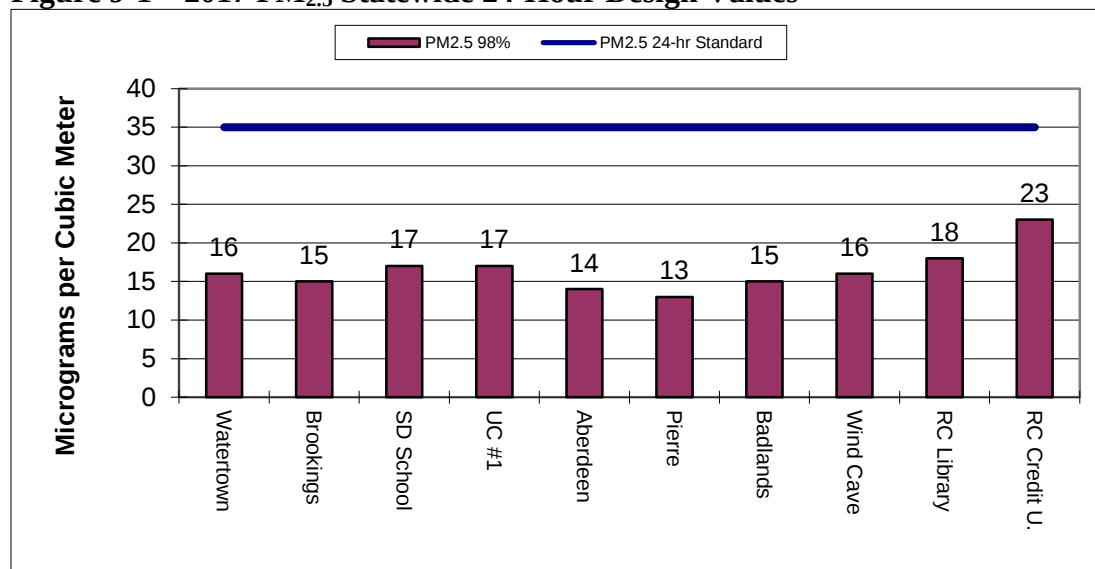
Figure 9-1 – 2017 PM 2.5 Statewide 24-Hour Design Values
