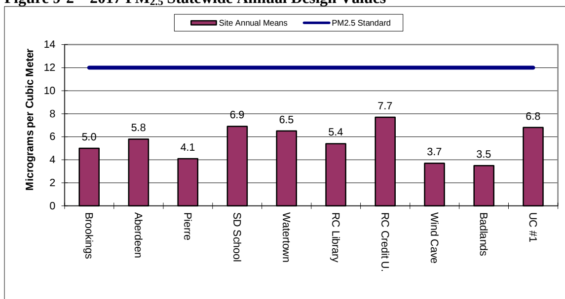
Figure 9-2 – 2017 PM 2.5 Statewide Annual Design Values
