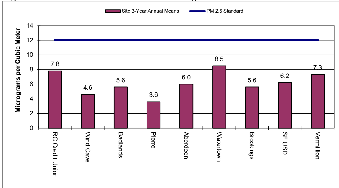
Figure 9-2 – 2023 PM 2.5 Statewide Annual Design Values
