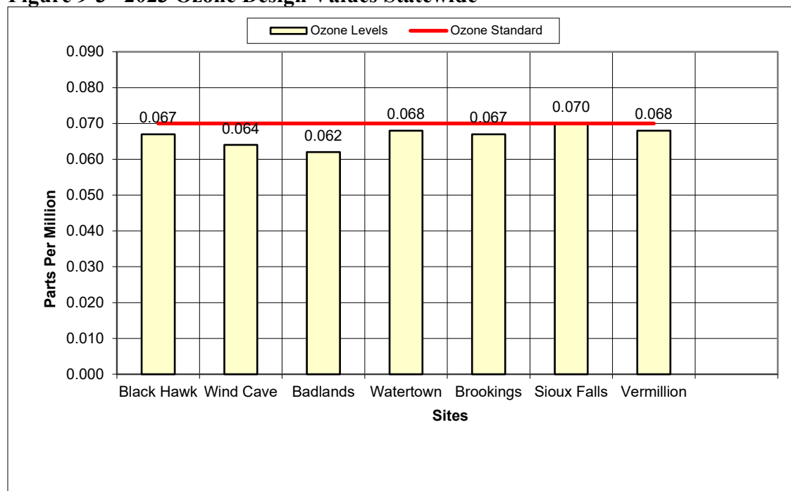
Figure 9-3– 2023 Ozone Design Values Statewide
