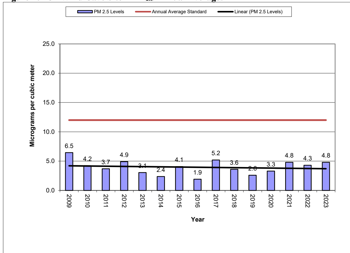
Figure 10-15 - Wind Cave Site – PM 2.5 Annual Averages
