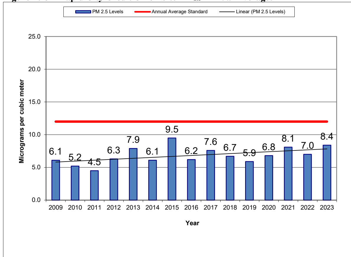
Figure 10-3 – Rapid City Credit Union Site PM 2.5 Annual Averages
