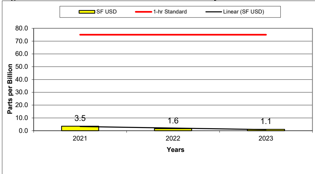
Figure 10-21 – SF USD Site – Sulfur Dioxide Yearly 1-hour 99th Percentile
