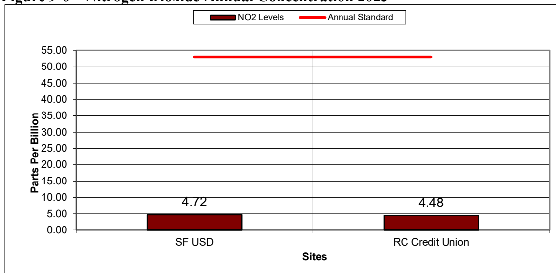
Figure 9-6 – Nitrogen Dioxide Annual Concentration 2023
