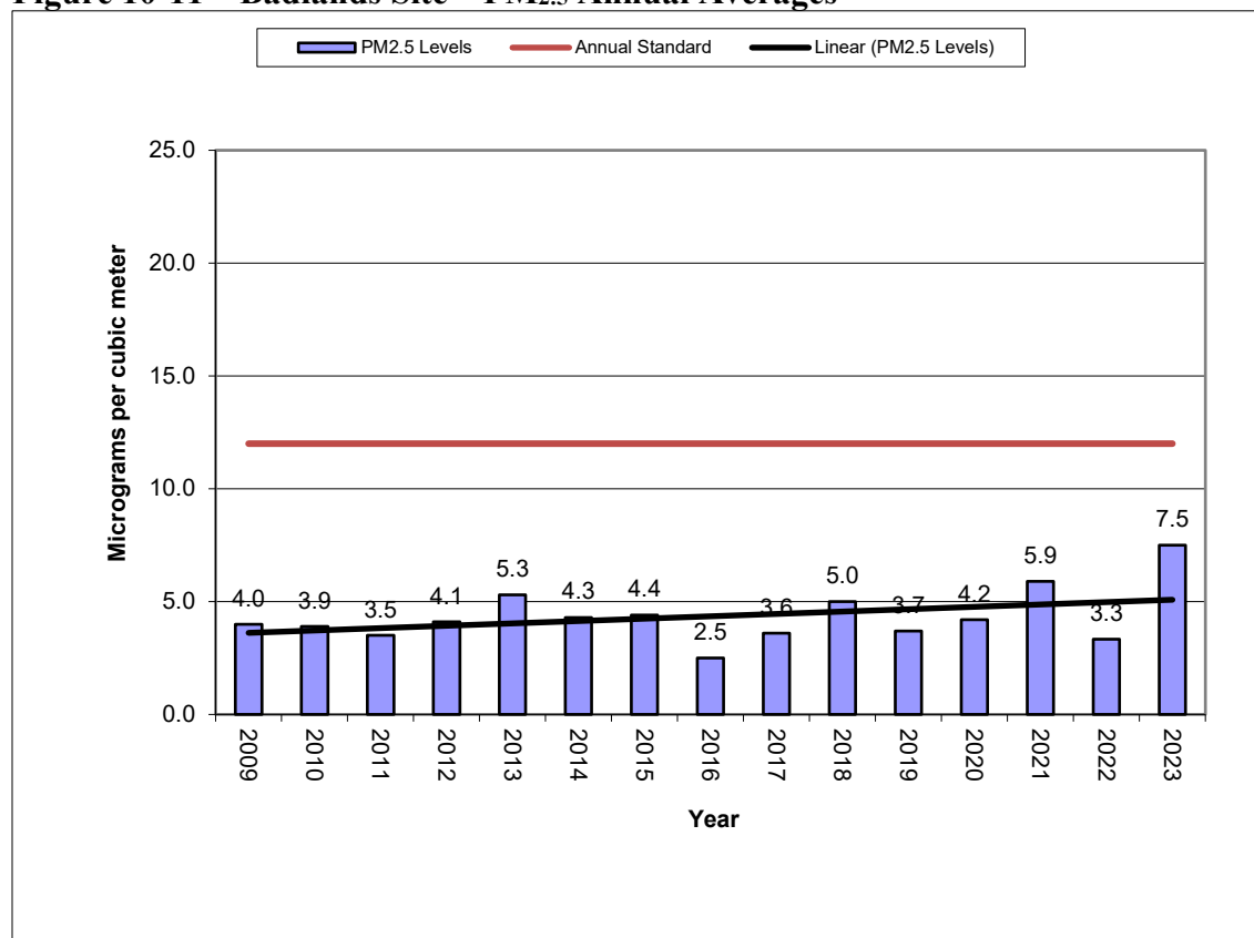
Figure 10-11 – Badlands Site – PM 2.5 Annual Averages
