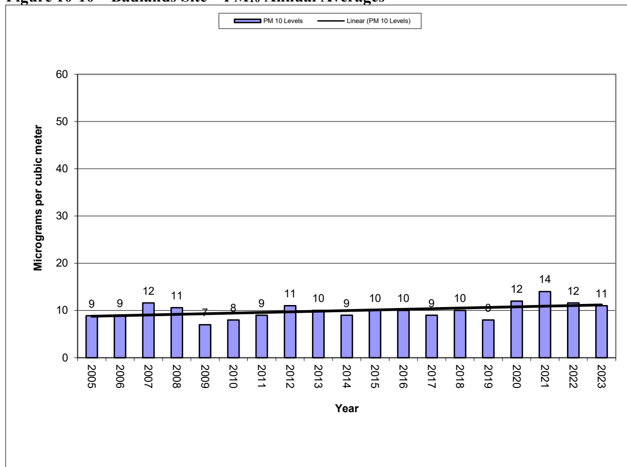
Figure 10-10 – Badlands Site – PM 10 Annual Averages
