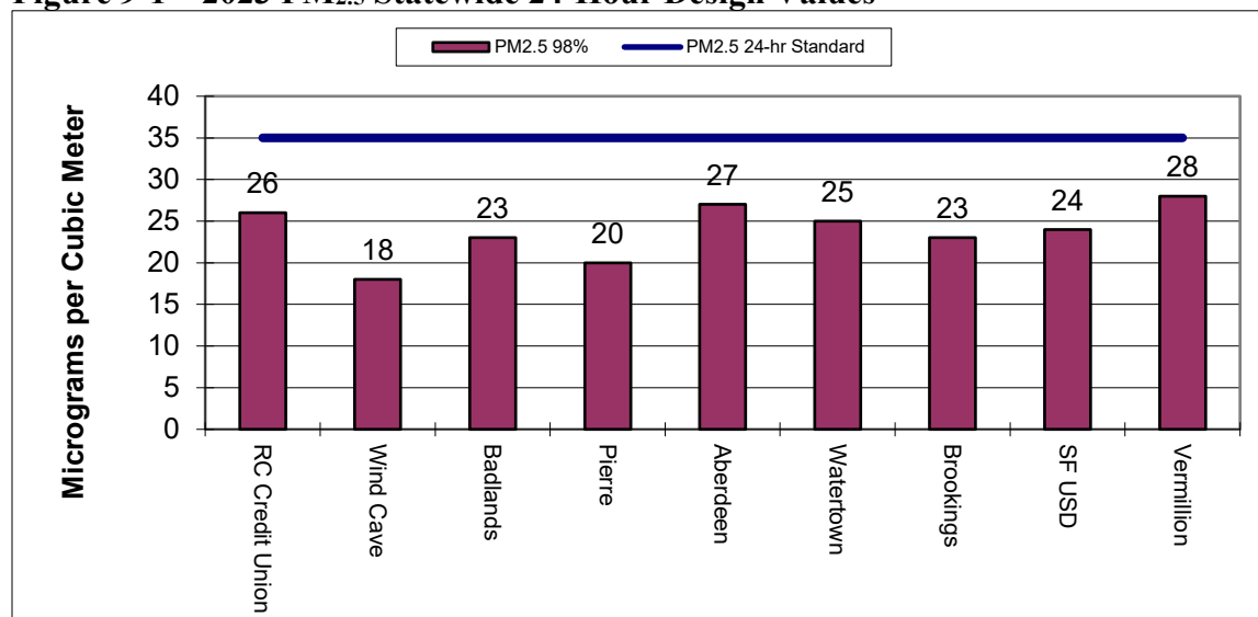
Figure 9-1 – 2023 PM 2.5 Statewide 24-Hour Design Values
