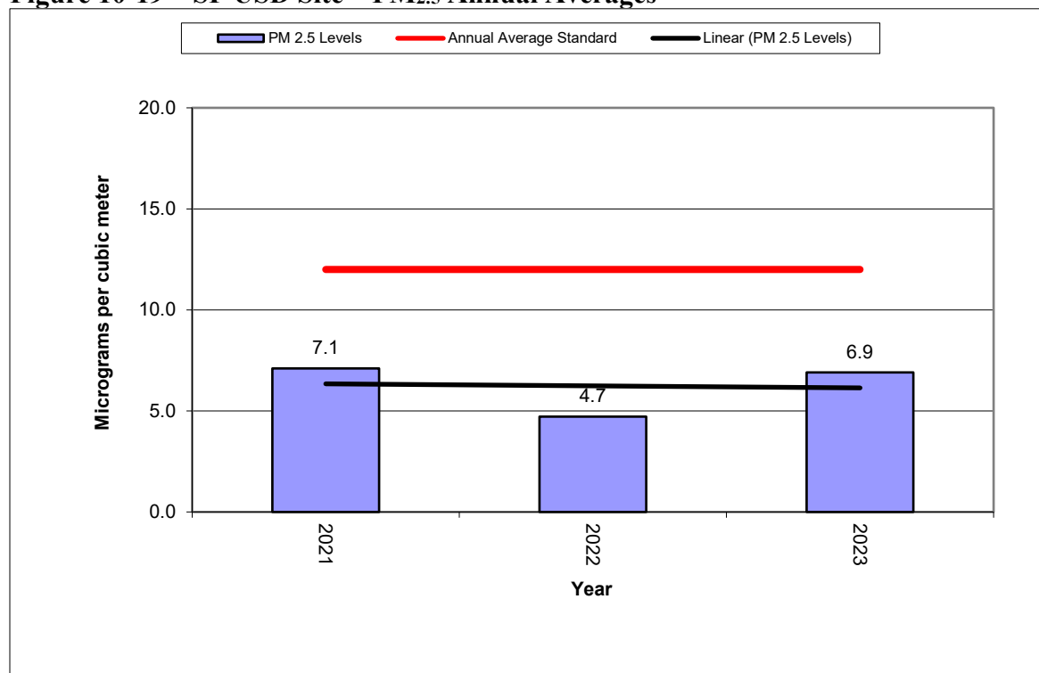
Figure 10-19 – SF USD Site – PM 2.5 Annual Averages
