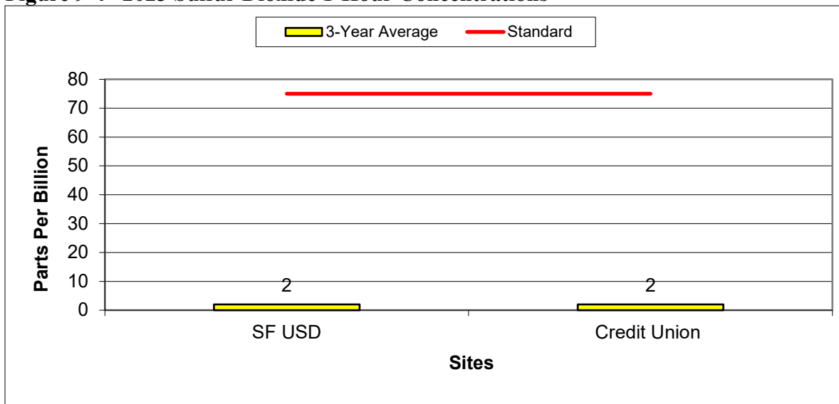
Figure 9-4– 2023 Sulfur Dioxide 1-Hour Concentrations
