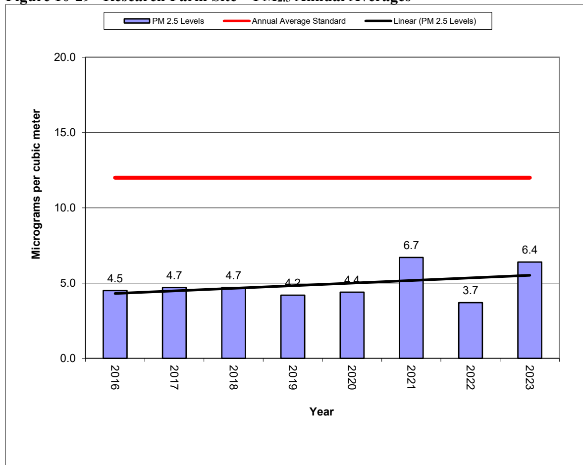
Figure 10-29 –Research Farm Site – PM 2.5 Annual Averages
