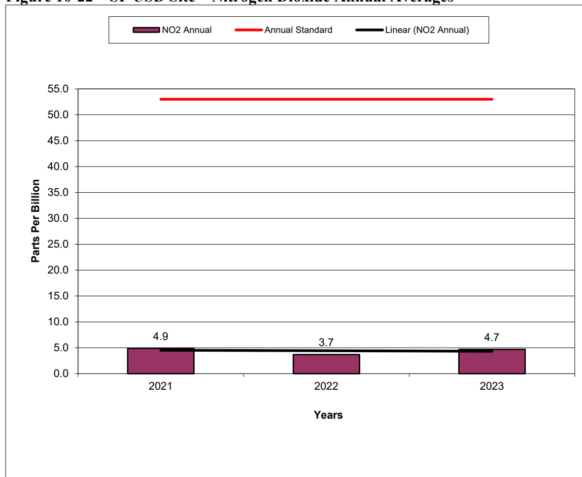
Figure 10-22 – SF USD Site – Nitrogen Dioxide Annual Averages
