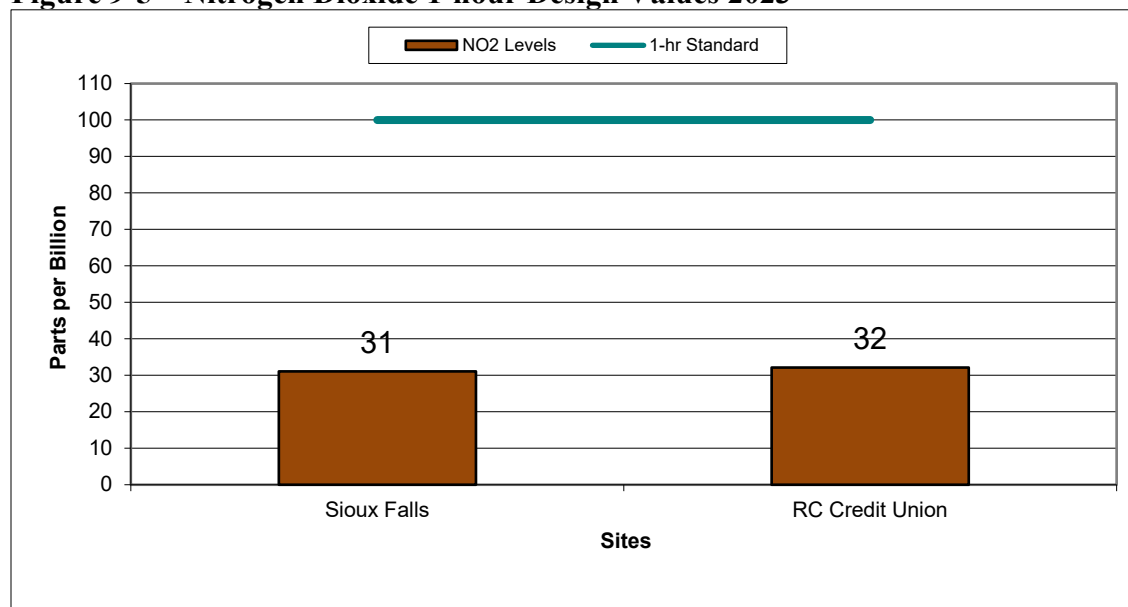
Figure 9-5 – Nitrogen Dioxide 1-hour Design Values 2023
