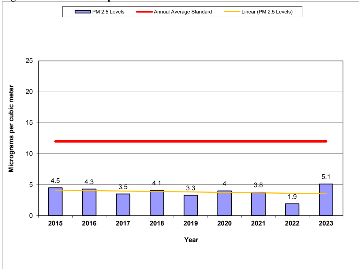
Figure 10-37 – Pierre Airport Site – Annual PM 2.5 Concentrations
