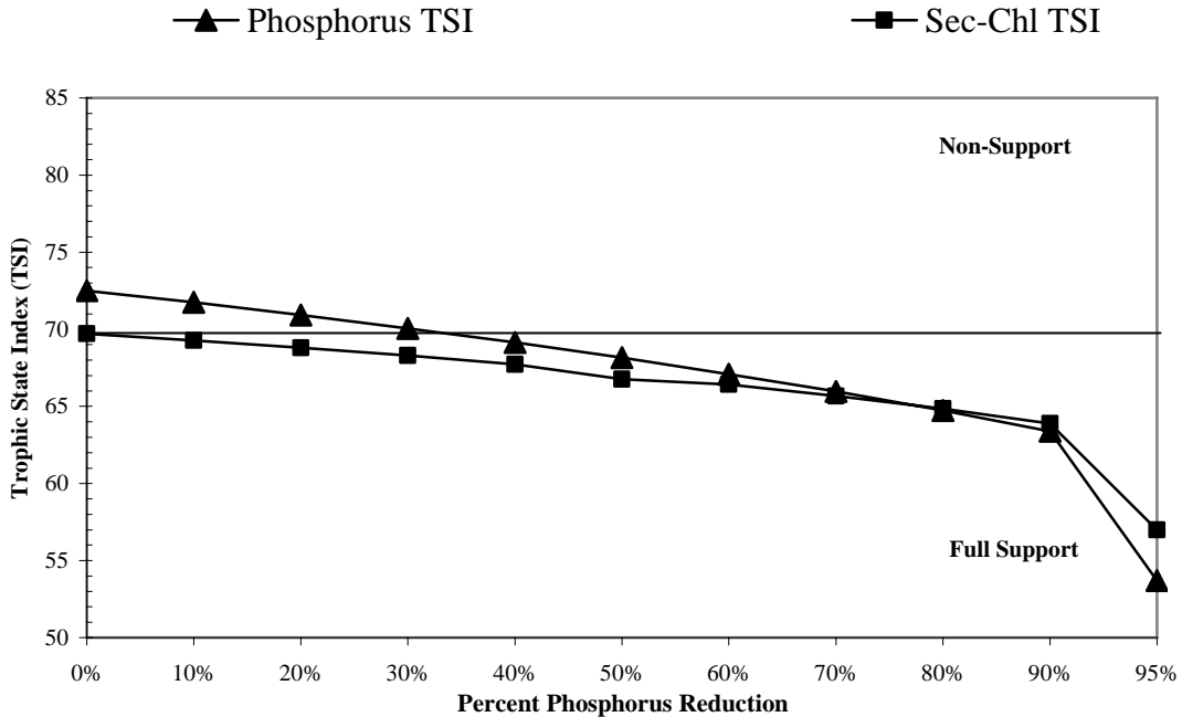
Figure 15. Graphical presentation of trophic state values in response to incremental percent reductions in total phosphorus loadings from sites WL02 and WL07 and alternative TSI target level.
