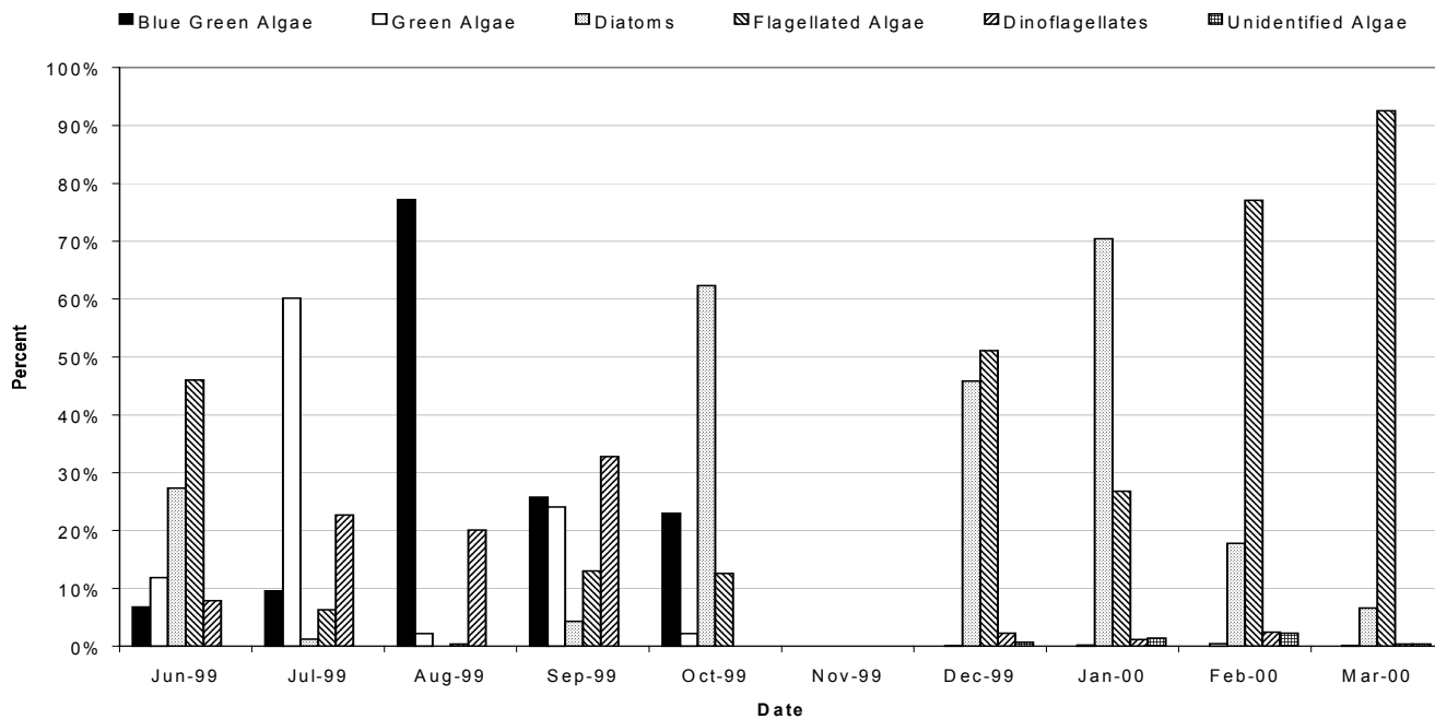
Figure 24. Average Biovolume by Date and Type for Lake Louise
