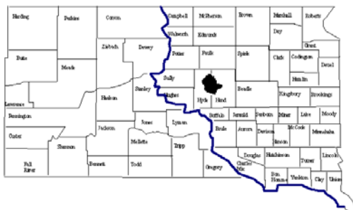
Figure 30. Watershed Location in South Dakota The north of Ree Heights created the lake, which has an average depth of 9 feet (3
