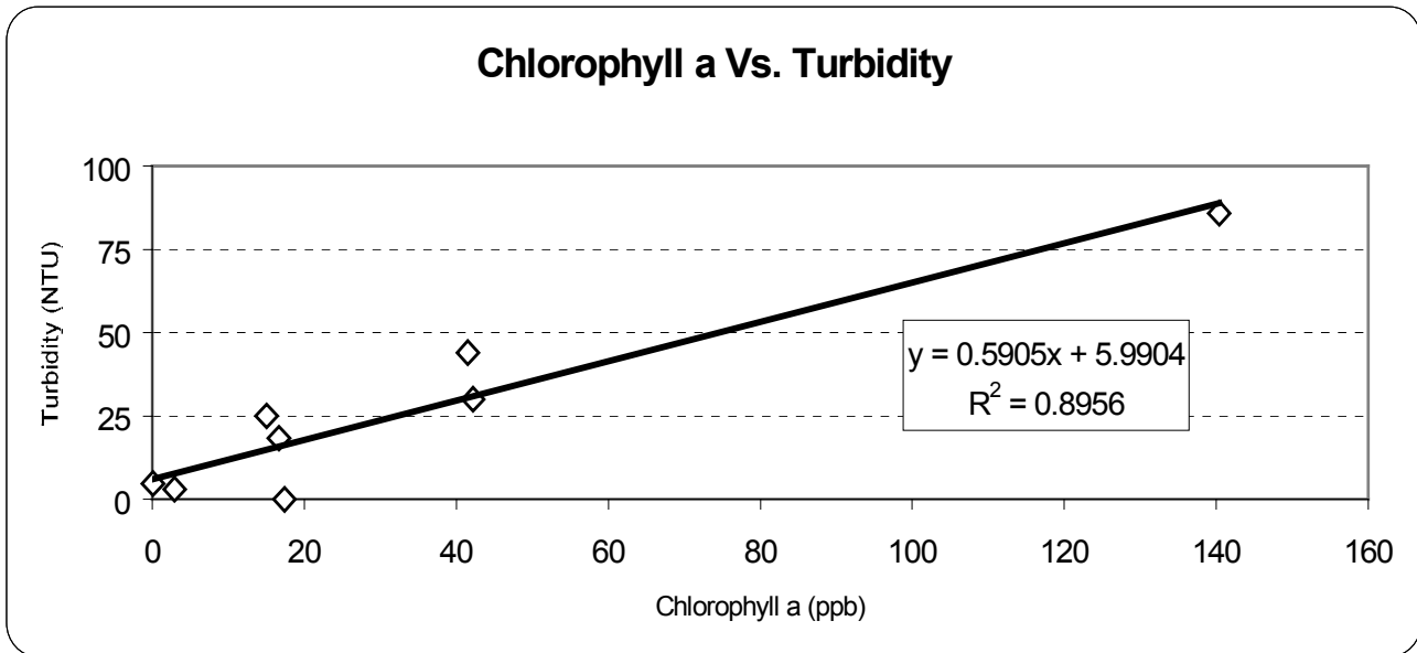
Figure 11. Chlorophyll a and Turbidity Correlation’s for Lake Louise
