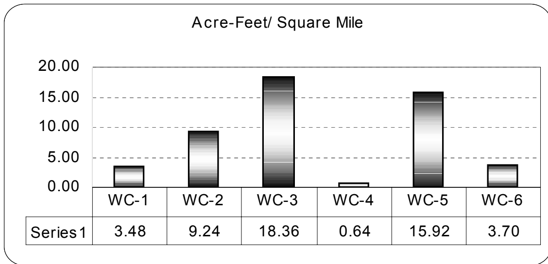
Figure 3. Subwatershed Discharge per Square Mile for the Wolf Creek Watershed
