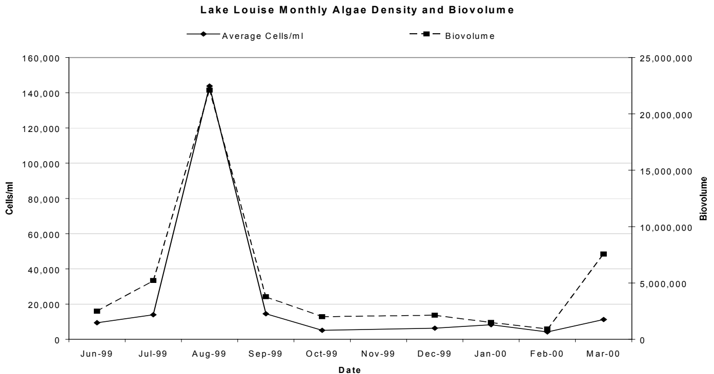
Figure 22. Monthly Algae Density and Biovolume for Lake Louise
