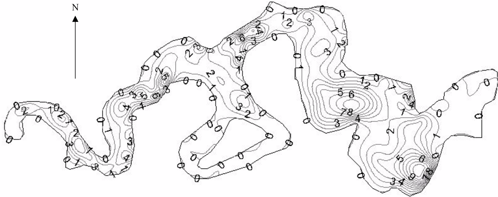
Figure 29. Lake Louise Sediment Map (Contours Expressed as Feet)
