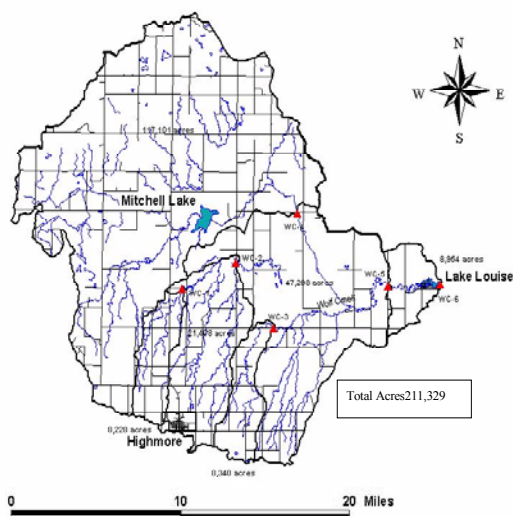
Figure 31. Lake Louise and Wolf Creek
