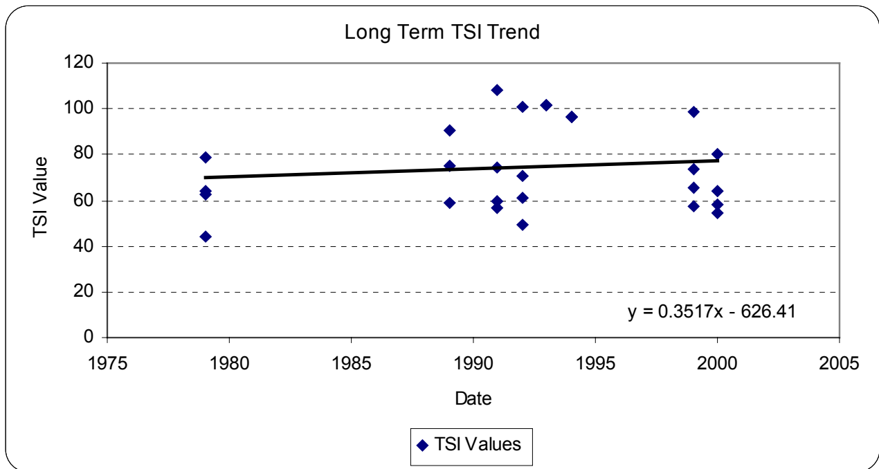
Figure 21. Long Term TSI Trends for Lake Louise
