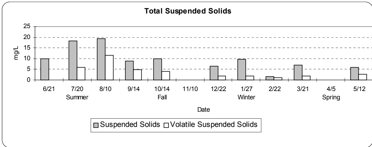
Figure 14. Total Suspended and Volatile Solids Concentrations for Lake Louise
