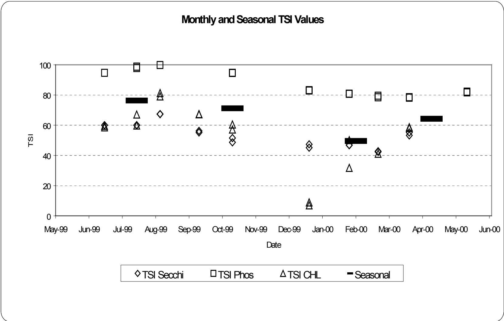
Figure 20. Monthly and Seasonal TSI Values for Lake Louise
