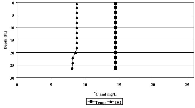
Lake Cochrane Dissolved Oxygen/Temperature Profile 7/21/99 LCL-3
