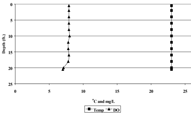
Lake Cochrane Dissolved Oxygen/Temperature Profile 10/20/99 LCL-2
