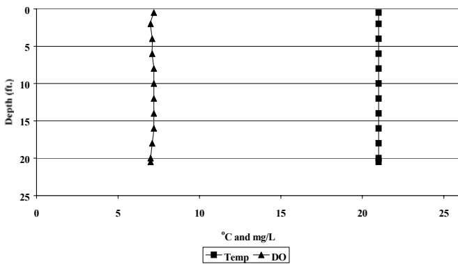
Lake Cochrane Dissolved Oxygen/Temperature Profile 8/23/99 LCL-2
