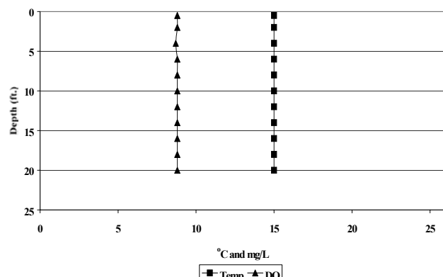
Lake Cochrane Dissolved Oxygen/Temperature Profile 11/22/99 LCL-2
