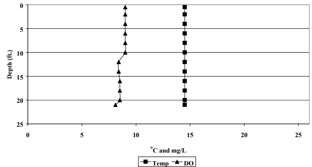
Lake Cochrane Dissolved Oxygen/Temperature Profile 7/21/99 LCL-2
