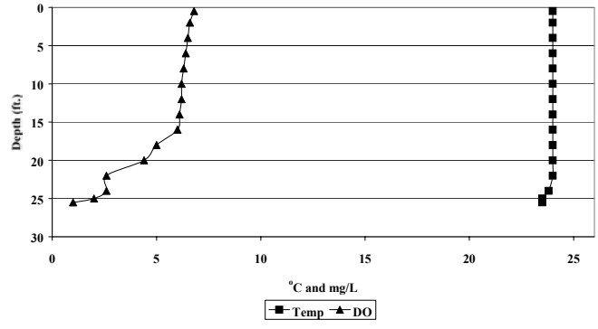
Lake Cochrane Dissolved Oxygen/Temperature Profile 9/22/99 LCL-3
