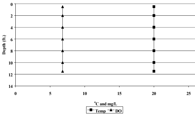
Lake Oliver Dissolved Oxygen/Temperature Profile 6/16/99 LOL-2
