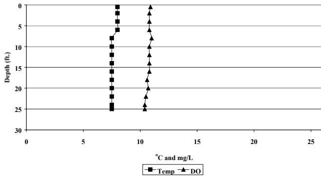
Lake Cochrane Dissolved Oxygen/Temperature Profile 6/16/99 LCL-3
