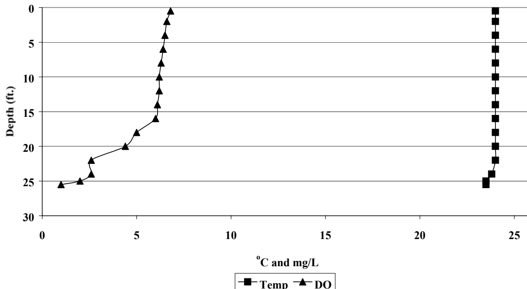
Figure 46. Lake Cochrane Diss. Oxygen/Temperature Profile 7/21/99 LCL-3.
