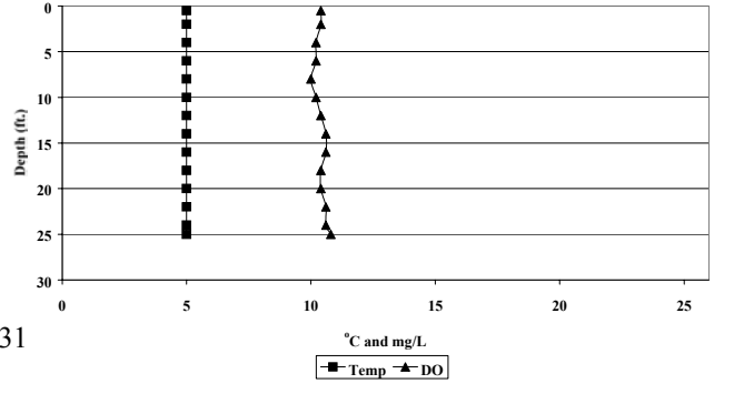
Lake Cochrane Dissolved Oxygen/Temperature Profile 11/22/99 LCL-3
