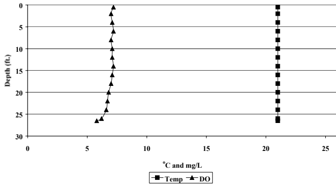
Lake Cochrane Dissolved Oxygen/Temperature Profile 8/23/99 LCL-3
