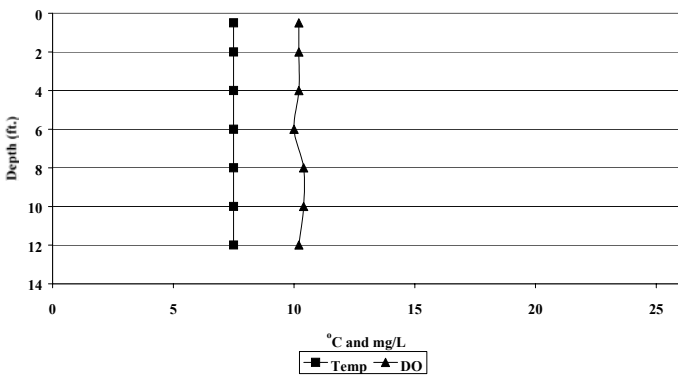
Lake Oliver Dissolved Oxygen/Temperature Profile 10/20/99 LOL-2
