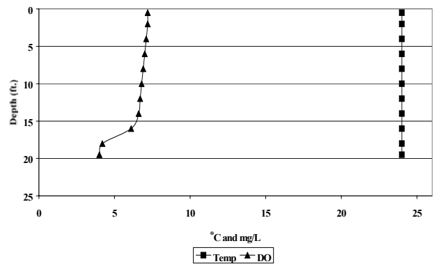
Lake Cochrane Dissolved Oxygen/Temperature Profile 9/22/99 LCL-2
