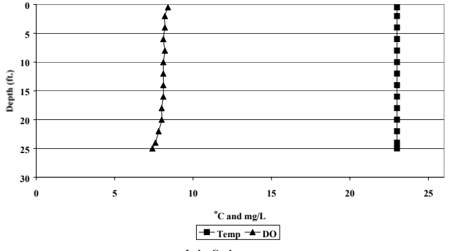
Lake Cochrane Dissolved Oxygen/Temperature Profile 10/20/99 LCL-3
