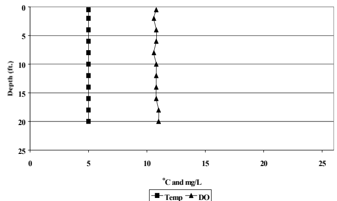
Lake Cochrane Dissolved Oxygen/Temperature Profile 11/22/99 LCL-2
