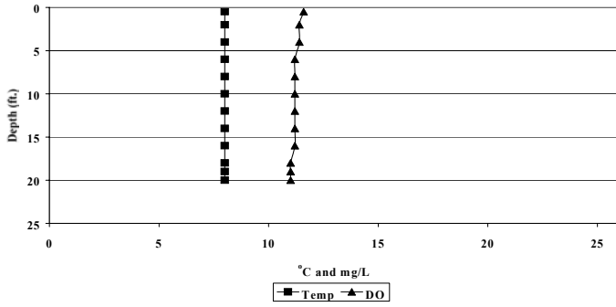
Lake Cochrane Dissolved Oxygen/Temperature Profile 6/16/99 LCL-2
