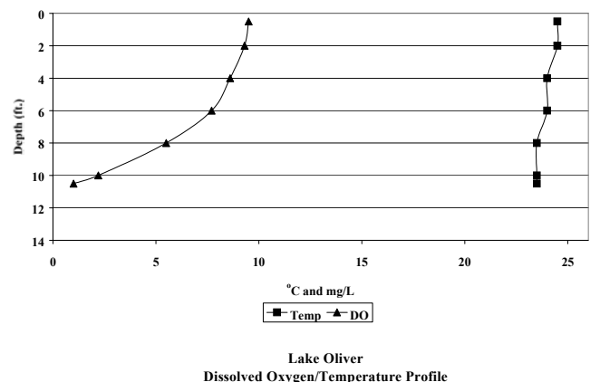
Lake Oliver Dissolved Oxygen/Temperature Profile 7/21/99 LOL-1
