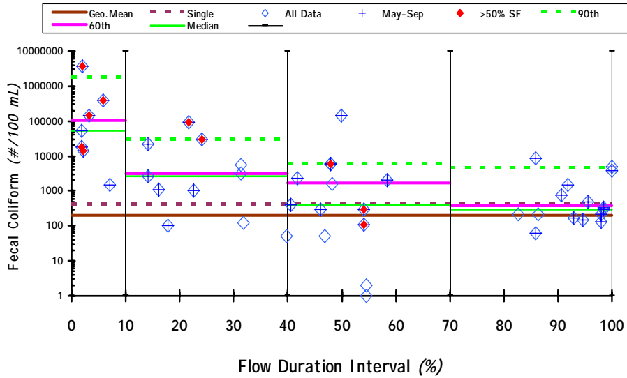
Figure 20. Comparison of Fecal Coliform Concentrations with WQS for LBST18
