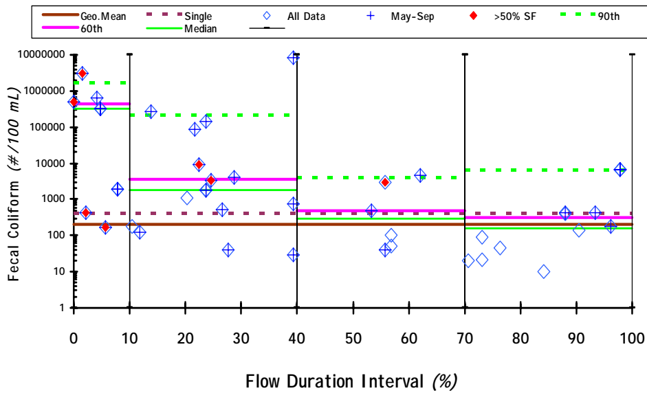
Figure 13. Comparison of Fecal Coliform Concentrations with WQS for LBST11
