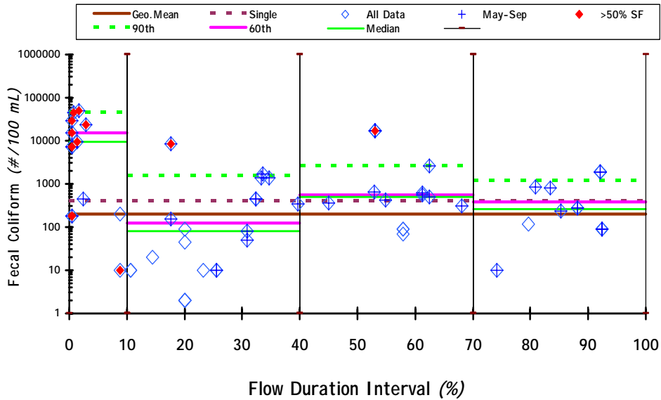
Figure 12. Comparison of Fecal Coliform Concentrations with WQS for LBST10
