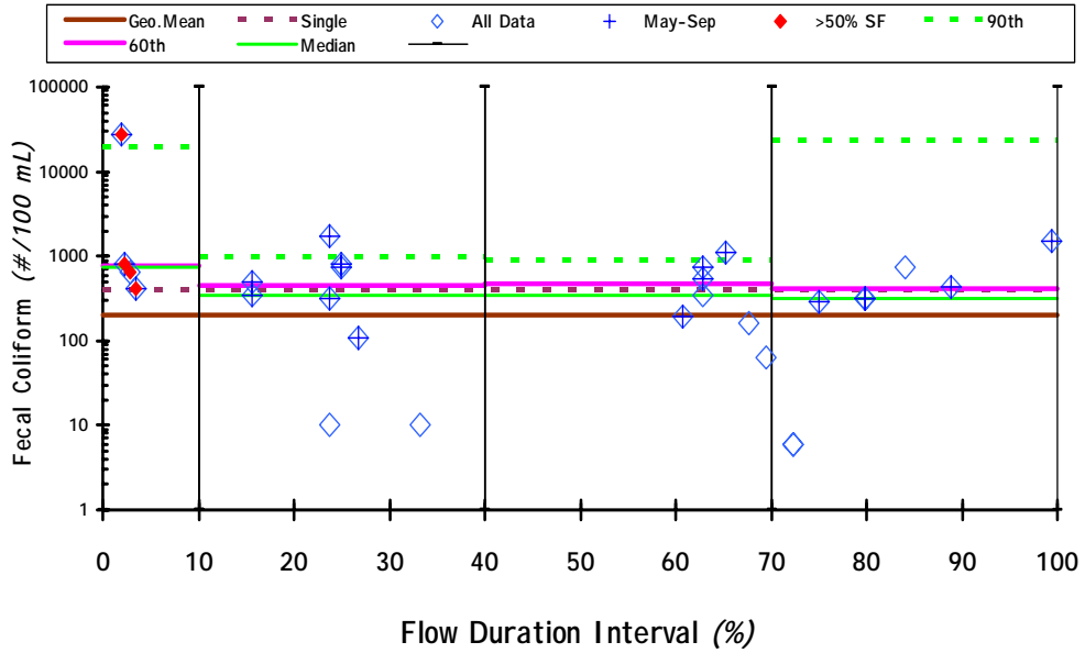
Figure 6. Comparison of Fecal Coliform Concentrations with WQS for LBST04
