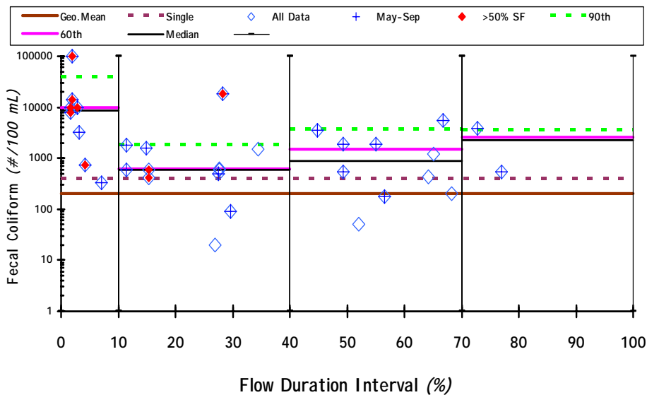
Figure 17. Comparison of Fecal Coliform Concentrations with WQS for LBST15
