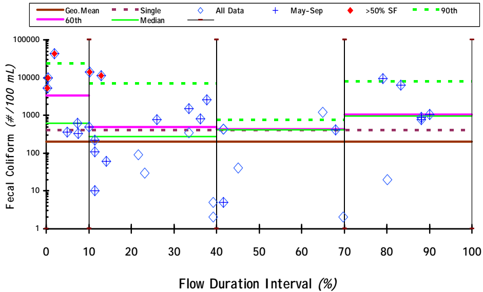
Figure 16. Comparison of Fecal Coliform Concentrations with WQS for LBST14
