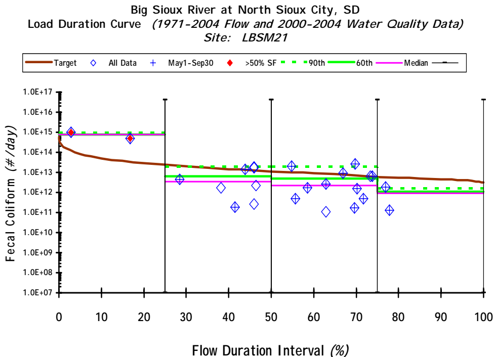
SDDENR WQData and Gage Duration Interval 7461 square miles Figure 36. BSRTMDL-5 Load Duration Curve for LBSM21
