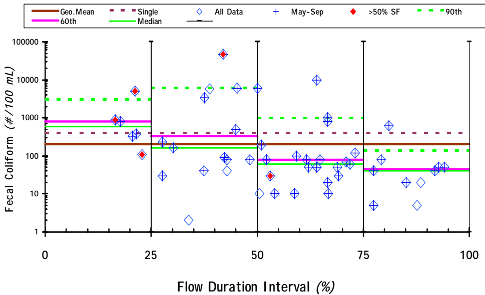
Figure 7. Comparison of Fecal Coliform Concentrations with WQS for BSM05
