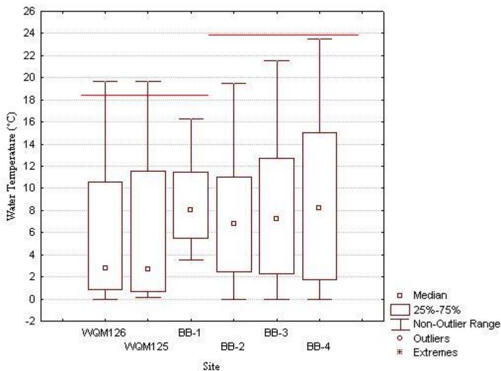
Figure 28. Water temperature values during the study period by site for Bear Butte Creek watershed mainstem sites. Horizontal lines are water temperature criteria for the coldwater permanent fish propagation (18.3 °C) and coldwater marginal fish propagation (23.9 °C) beneficial uses.
