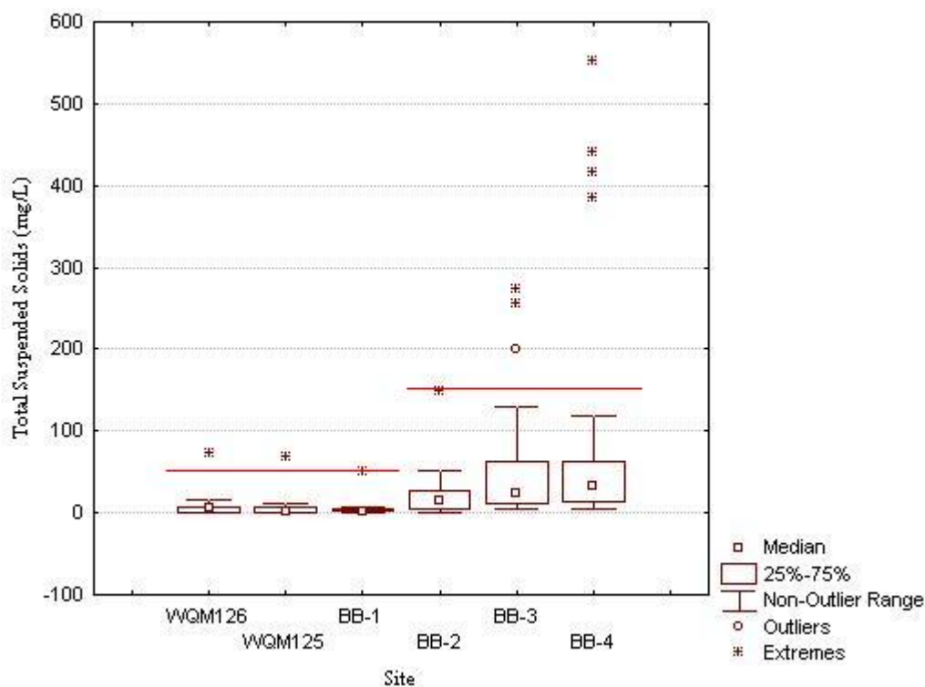
Figure 22. Box plot of total suspended solids concentrations by site for Bear Butte Creek mainstem sites. Horizontal lines are TSS criteria for the coldwater permanent fish propagation (53 mg/L) and coldwater marginal fish propagation (158 mg/L) beneficial uses.
