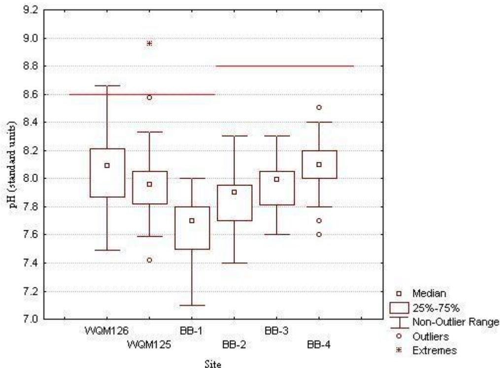
Figure 6. Box plot of field pH values by site for Bear Butte Creek mainstem sites. Horizontal lines are the upper pH criteria for the coldwater permanent fish propagation (8.6 standard units) and coldwater marginal fish propagation (8.8 standard units) beneficial uses.
