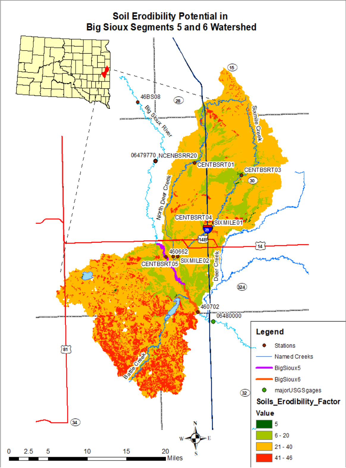
Figure 3 - Soil Erodibility Potential in Big Sioux Segment 5 and 6 Watershed
