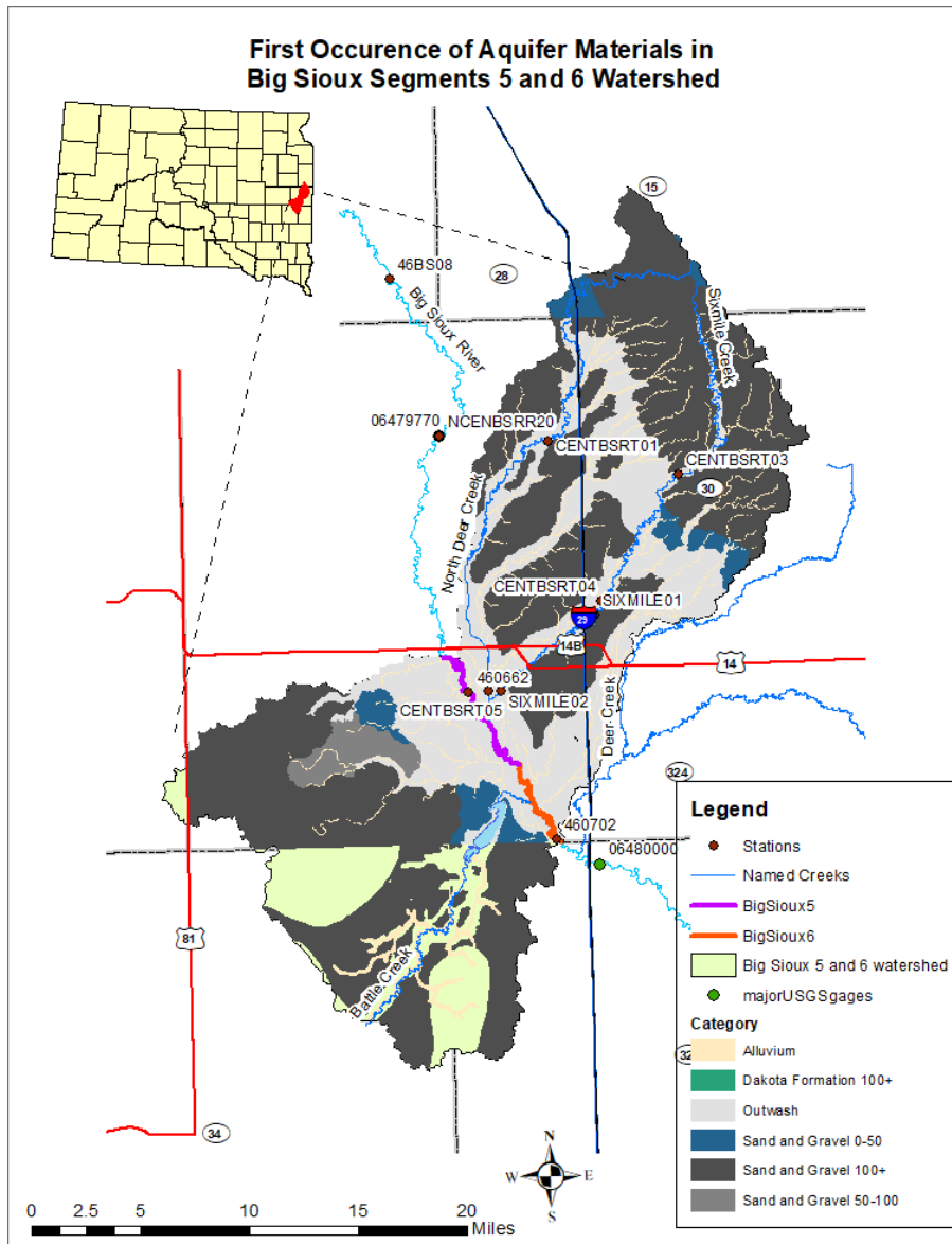
Figure 2 - Occurrence of Aquifer Material in Big Sioux Segments 5 and 6 Watershed
