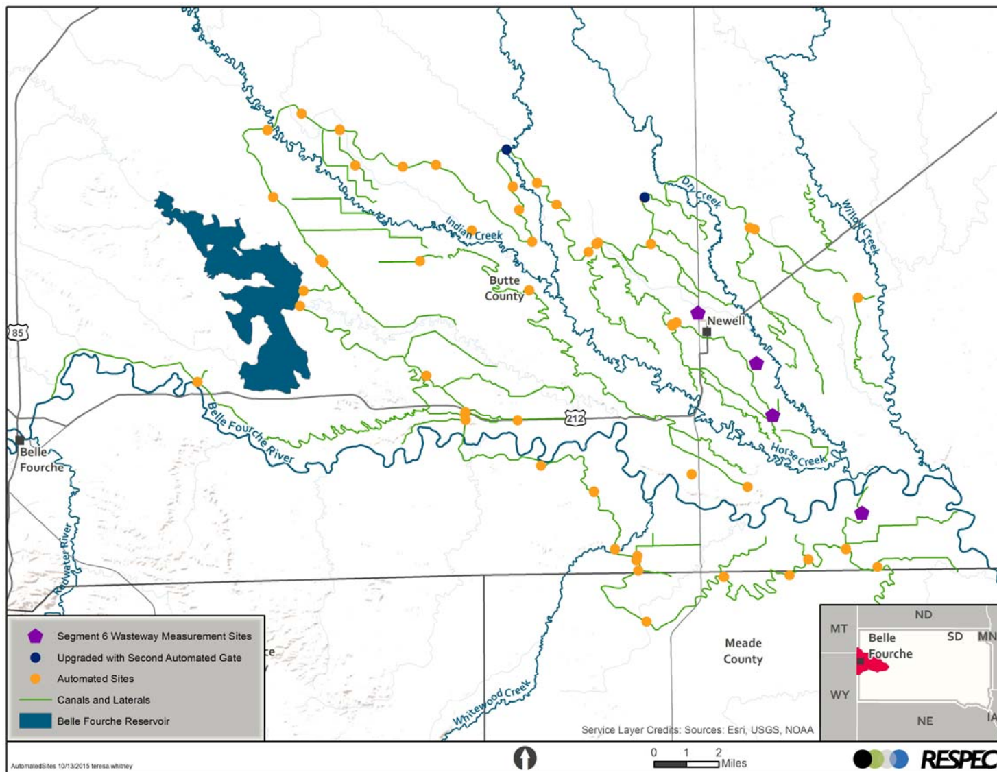
Figure 3-1. Location of the Automated Sites in the Belle Fourche Irrigation District Installed During Segment 6.
