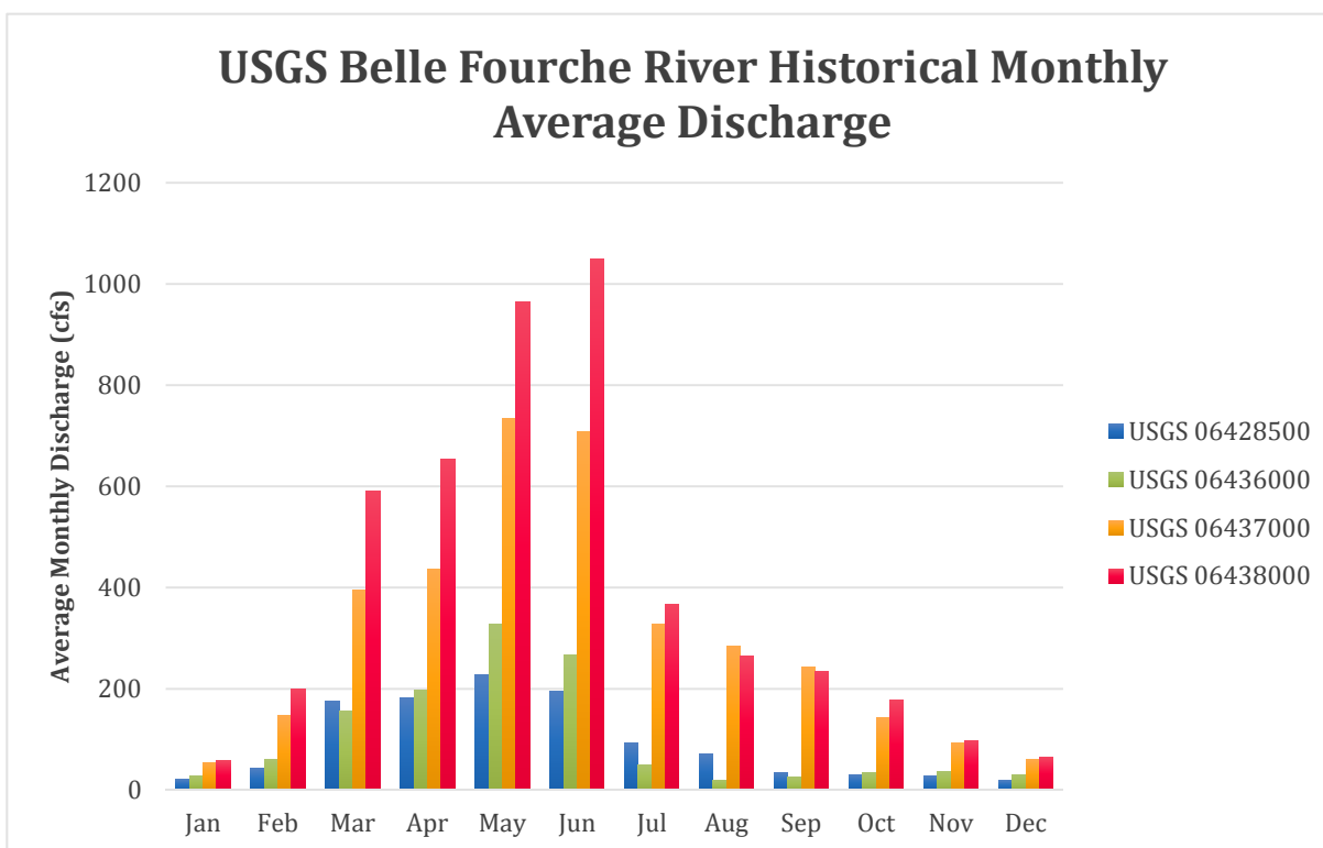
Figure 5-3. Average Historical Monthly Flows on the Belle Fourche River at U.S. Geological Survey Gaging Locations Within the Belle Fourche River Watershed in South Dakota.
