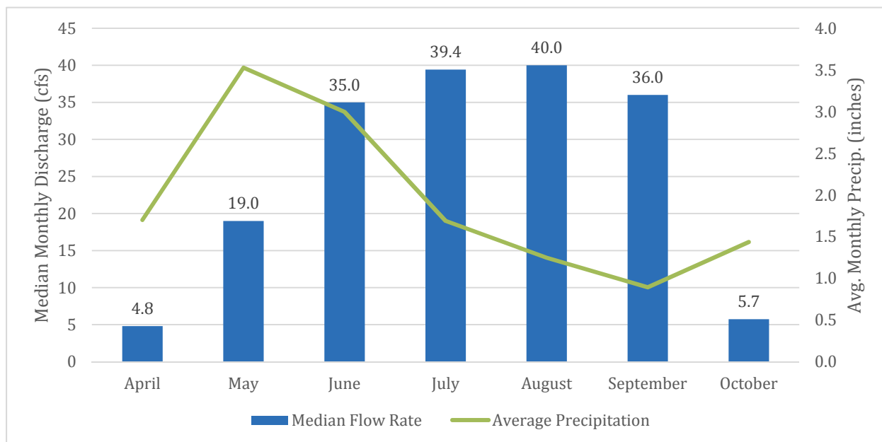
Figure 5-6. Historical Median Discharge on Horse Creek and Average Precipitation at Newell, South Dakota.
