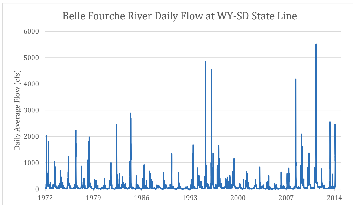
Figure 5-4. Daily Average Flow for the Belle Fourche River at the State Line (USGS 06428500).
