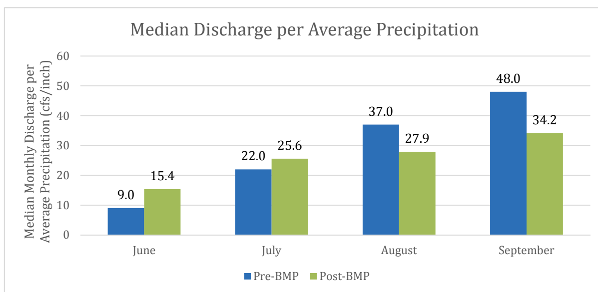
Figure 5-7. Comparison of the Median Flow Rate per Average Precipitation by Month for the Pre-BMP and Post-BMP Implementation Periods.
