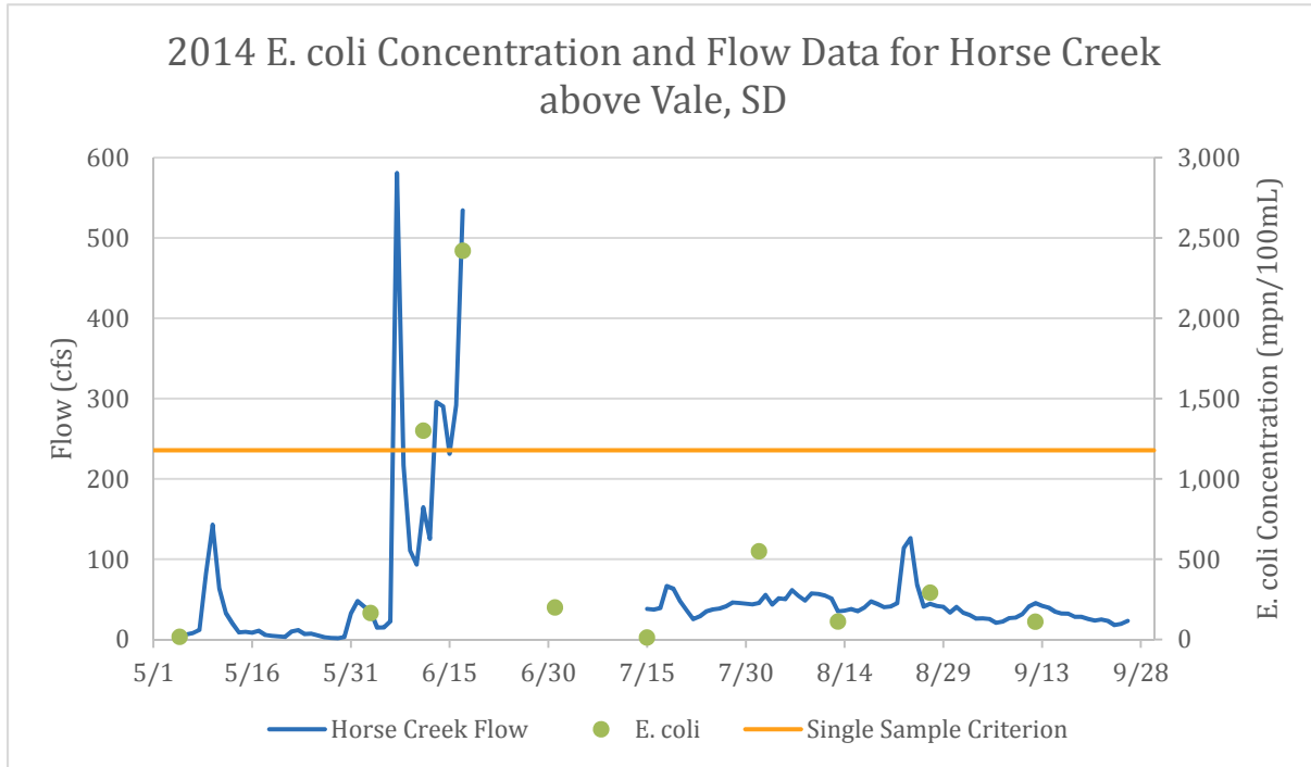
Figure 5-9. 2014 E. Coli Concentrations and Flow for Horse Creek Within the Belle Fourche River Watershed in South Dakota.
