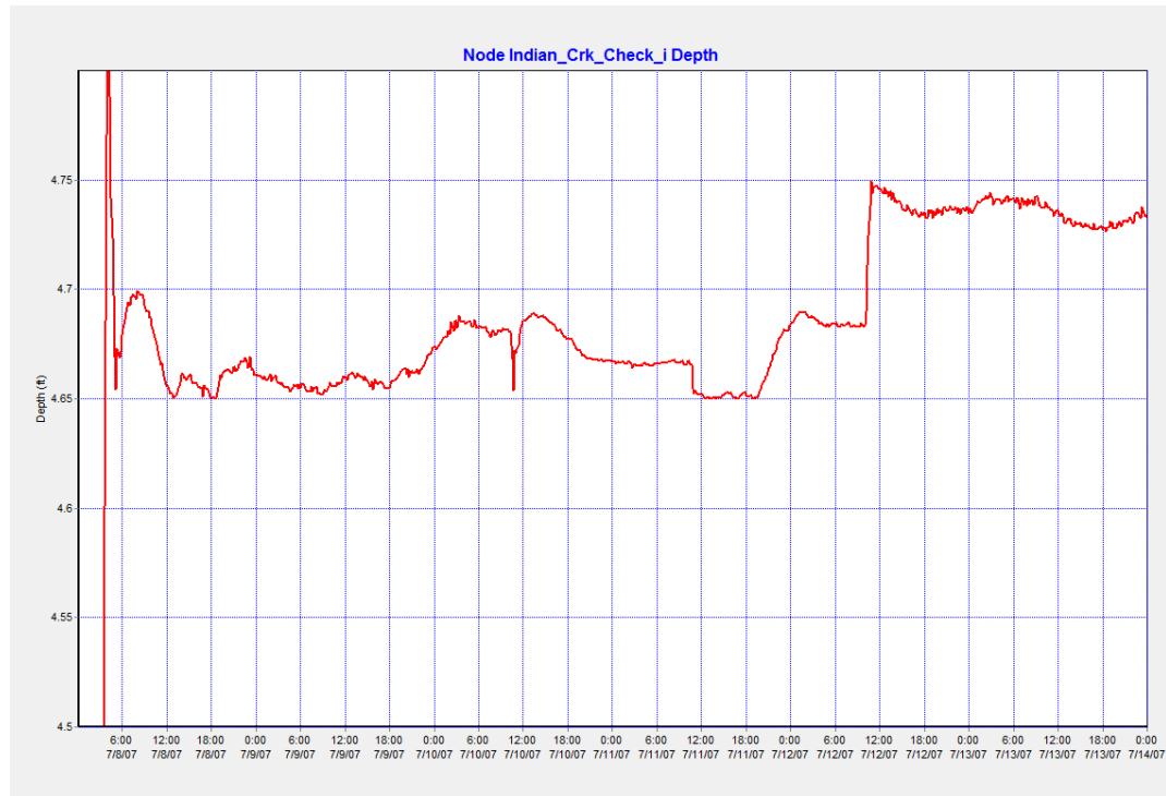
Figure 40. Modeled upstream water depth as a result of the PID modulated control rule with a time to open/close the automated gate equal to 1.0 hours and a K_p value of -70.0 TTOC = 1.0 hrs, K_p = -70.0
