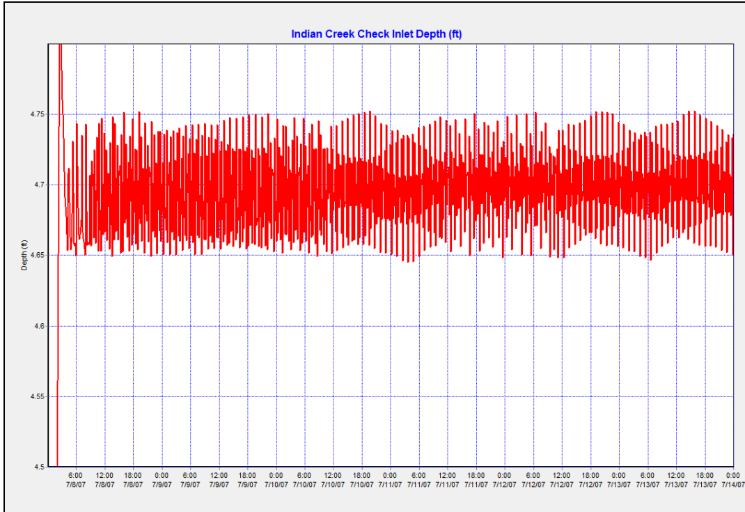
Figure 28. Figure 20. Upstream stage at the Indian Creek check using the control rules recommended by Schoenfelder (2006) and a time to open/close of 1.0 hrs.
