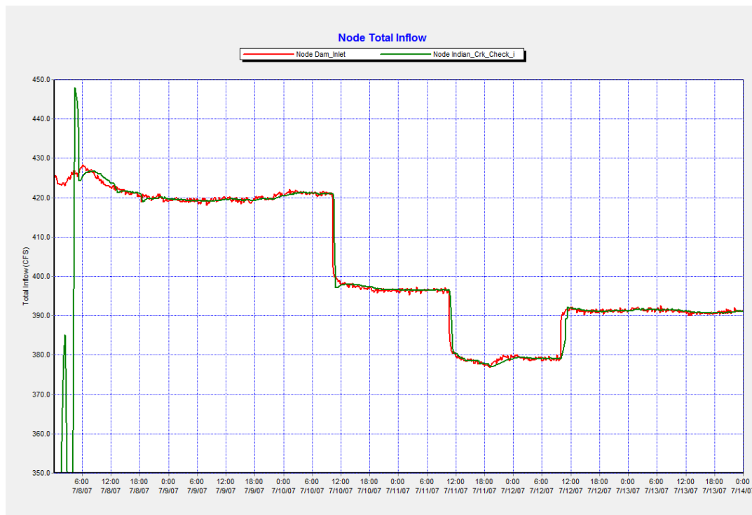
Figure 41. Modeled flow as a result of the PID modulated control rule with a time to open/close the automated gate equal to 1.0 hours and a K_p value of -70.0 .
