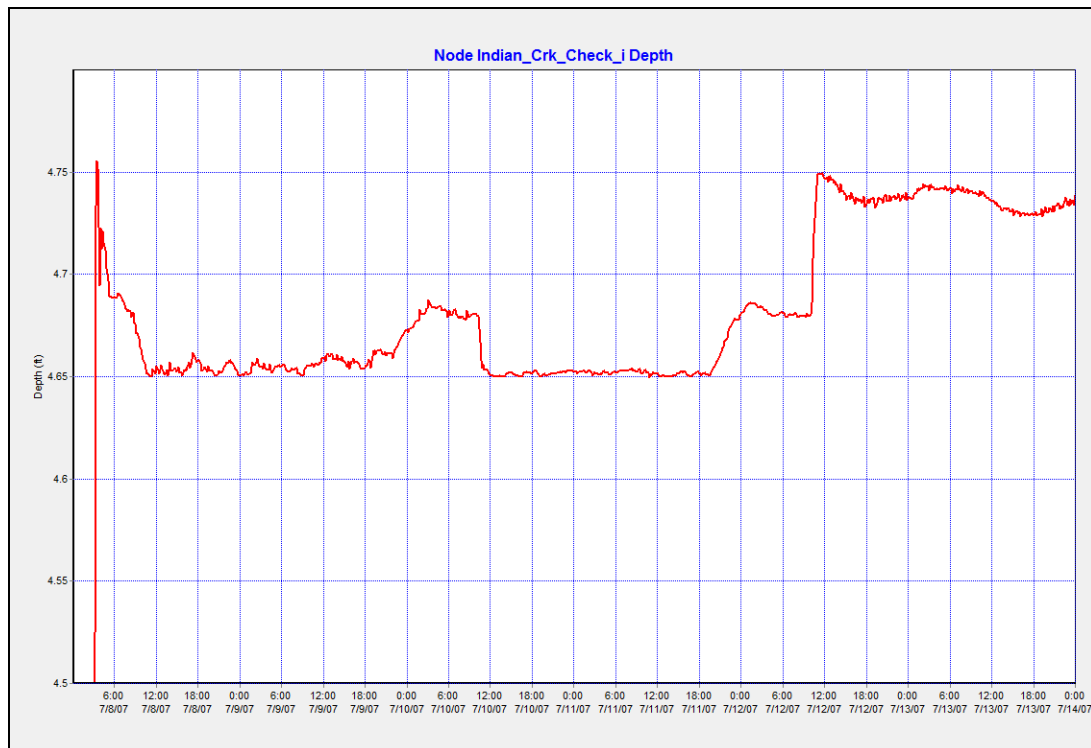
Figure 42. Modeled upstream water depth as a result of the PID modulated control rule with a time to open/close the automated gate equal to 0.25 hours and a Kp value of -70.0
