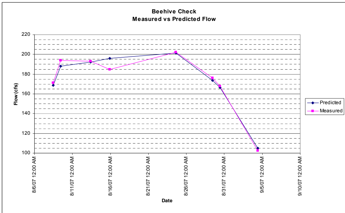
Figure 10. Comparison of measured flow to the predicted flow estimated by the model for the Beehive check.
