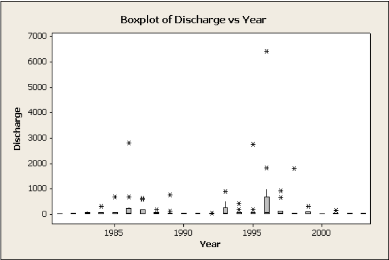
Figure G-4. Box Plot of TDS, SC, and Discharge Versus Year for USGS Site 6436760.
