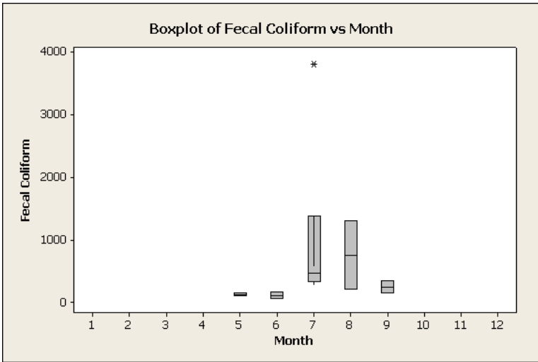
Figure B-1. Box Plot of SSC, TSS, Turbidity, and Fecal Coliform Versus Month for Storet ID 460130.
