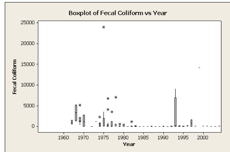
Figure H-3. Box Plot of SSC, TSS, Turbidity, and Fecal Coliform Versus Year for USGS Site 6437000.
