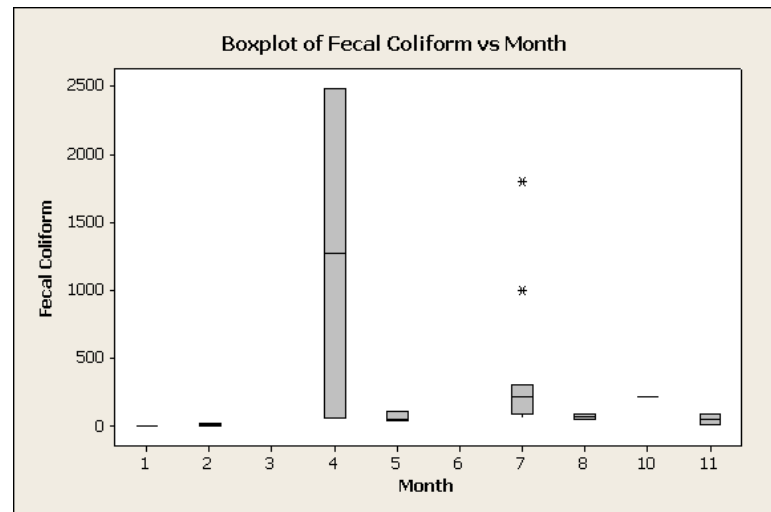
Figure C-1. Box Plot of SSC, TSS, Turbidity, and Fecal Coliform Versus Month for Storet ID 460681.
