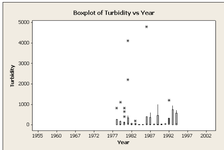
Figure A-5. Box Plot of SSC, TSS, Turbidity, and Fecal Coliform Versus Year for All Sites.
