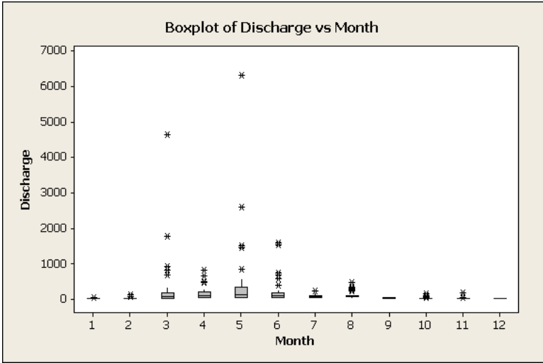
Figure E-2. Box Plot of TDS, SC, and Discharge Versus Month for USGS Site 6428500.
