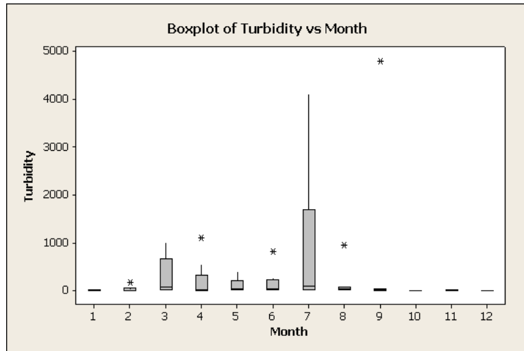
Figure I-1. Box Plot of SSC, TSS, Turbidity, and Fecal Coliform Versus Month for USGS Site 6438000.
