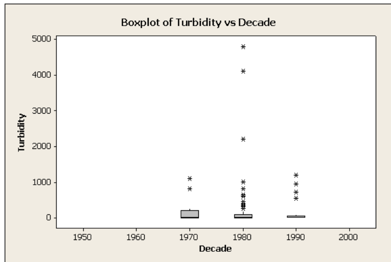
Figure A-7. Box Plot of SSC, TSS, Turbidity, and Fecal Coliform Versus Decade for All Sites.
