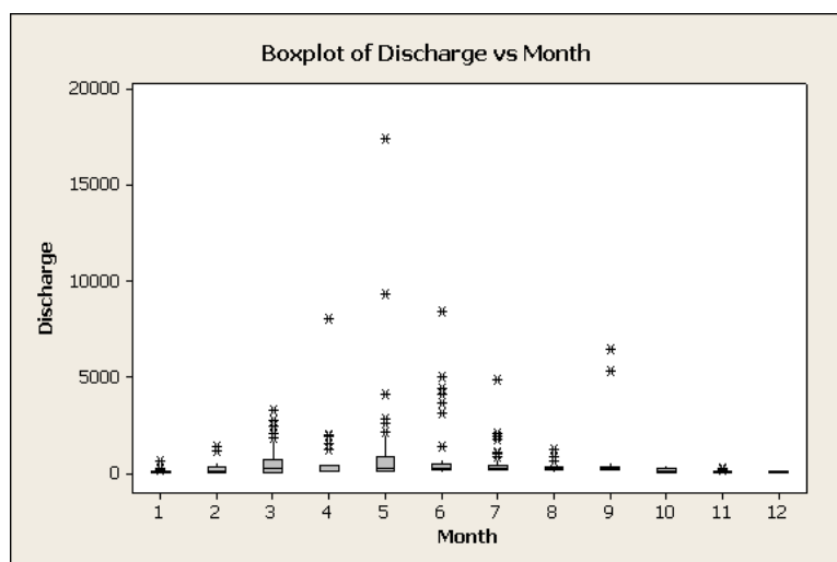
Figure H-2. Box Plot of TDS, SC, and Discharge Versus Month for USGS Site 6437000.
