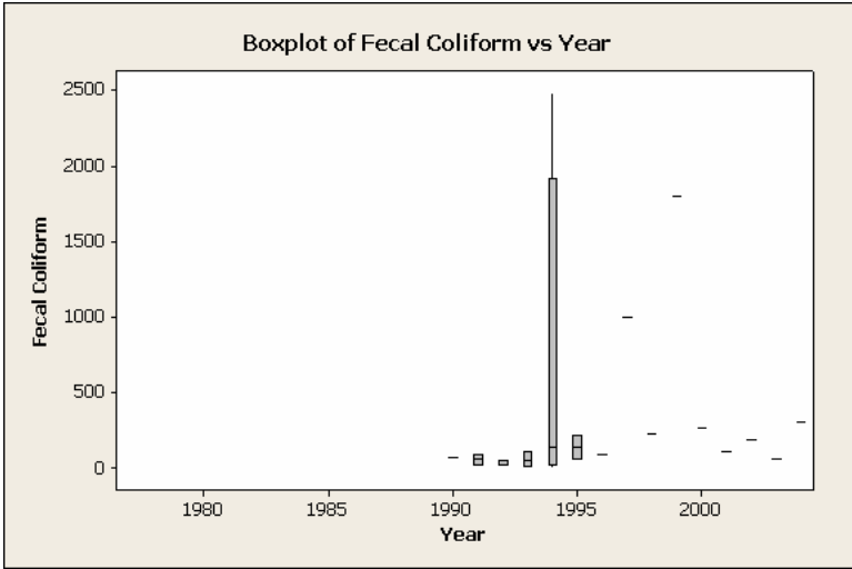
Figure C-3. Box Plot of SSC, TSS, Turbidity, and Fecal Coliform Versus Year for Storet ID 460681.
