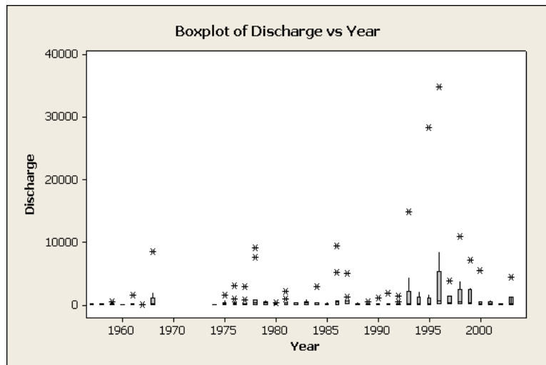
Figure I-4. Box Plot of TDS, SC, and Discharge Versus Year for USGS Site 6438000.
