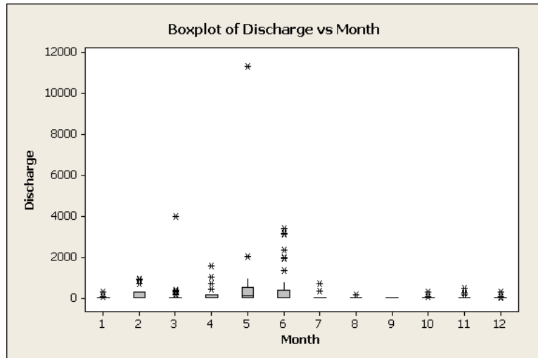
Figure F-2. Box Plot of TDS, SC, and Discharge Versus Month for USGS Site 6436000.
