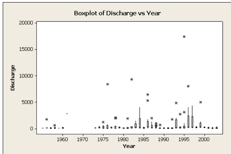
Figure H-4. Box Plot of TDS, SC, and Discharge Versus Year for USGS Site 6437000.
