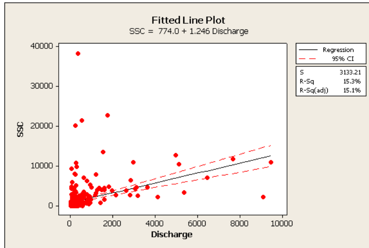
Figure A-9. Fitted Line for TDS Versus SC, SSC Versus Turbidity, SSC Versus Discharge, and Turbidity Versus Discharge for All Sites.
