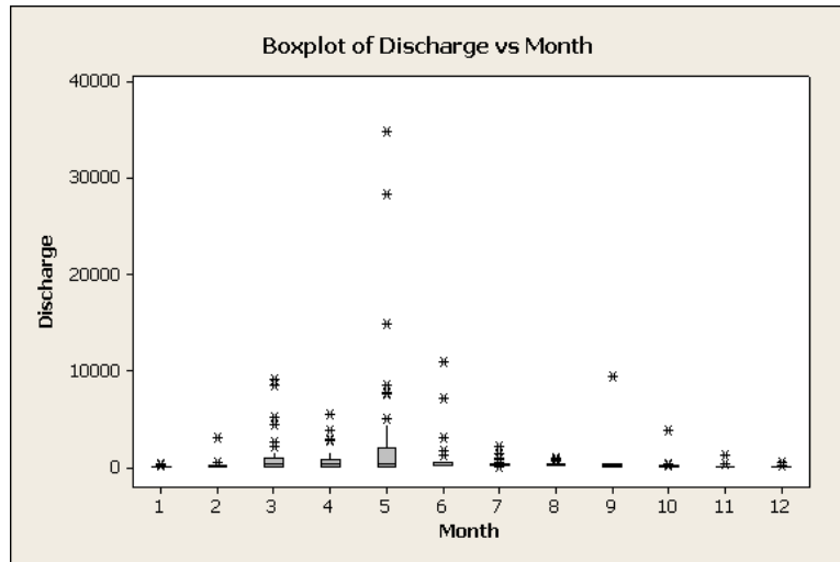
Figure I-2. Box Plot of TDS, SC, and Discharge Versus Month for USGS Site 6438000.
