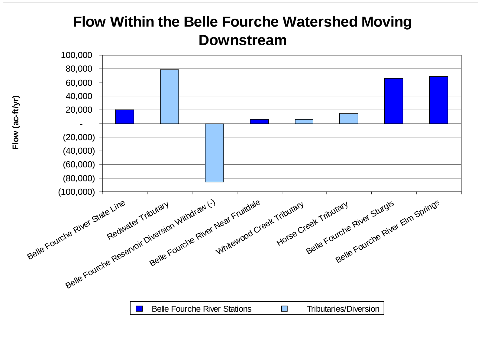
Figure A-2. Belle Fourche River Watershed Water Budget.
