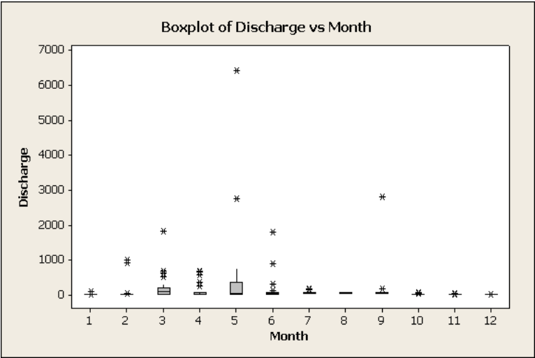
Figure G-2. Box Plot of TDS, SC, and Discharge Versus Month for USGS Site 6436760.
