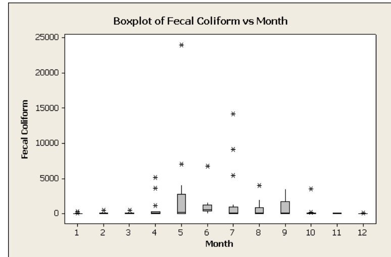
Figure H-1. Box Plot of SSC, TSS, Turbidity, and Fecal Coliform Versus Month for USGS Site 6437000.
