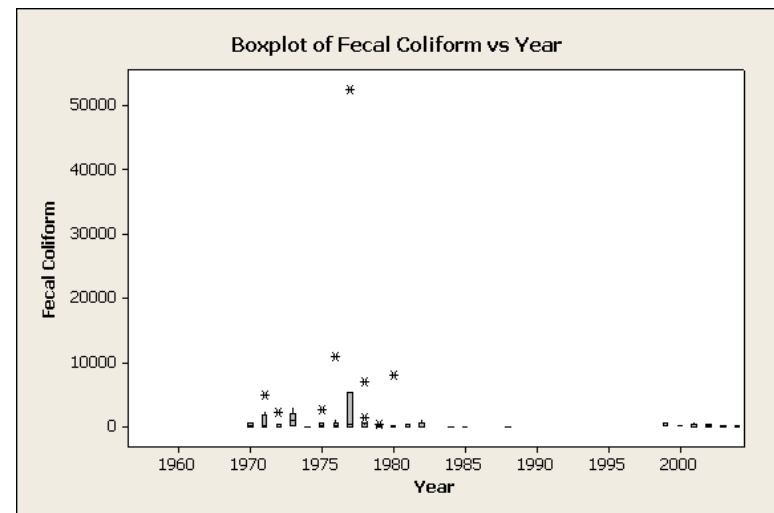
Figure I-3. Box Plot of SSC, TSS, Turbidity, and Fecal Coliform Versus Year for USGS Site 6438000.
