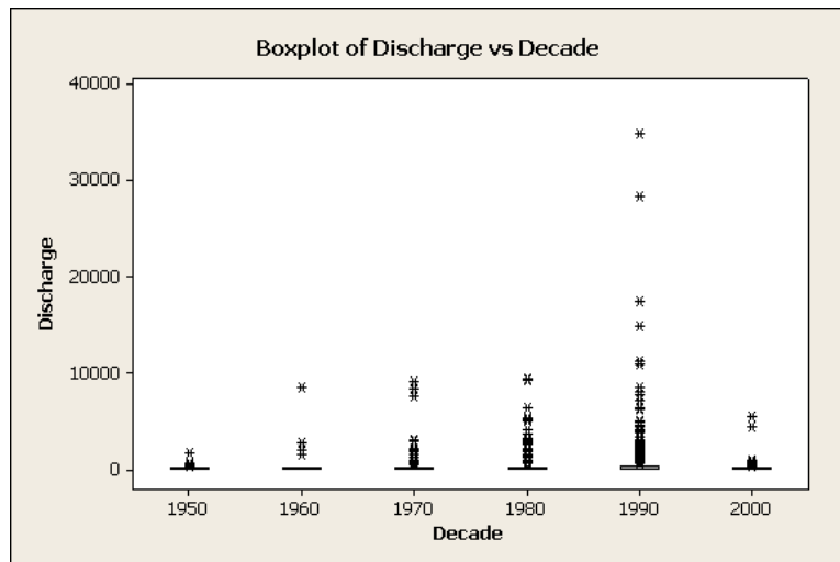
Figure A-8. Box Plot of TDS, SC, and Discharge Versus Decade for All Sites.
