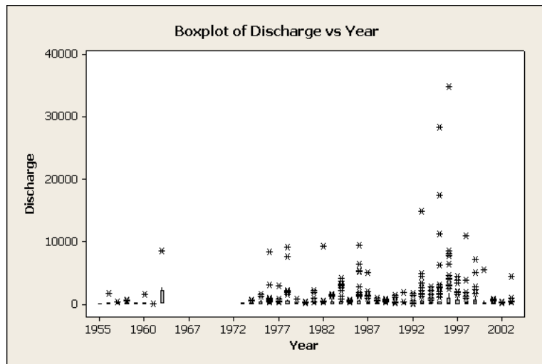
Figure A-6. Box Plot of TDS, SC, and Discharge Versus Year for All Sites.
