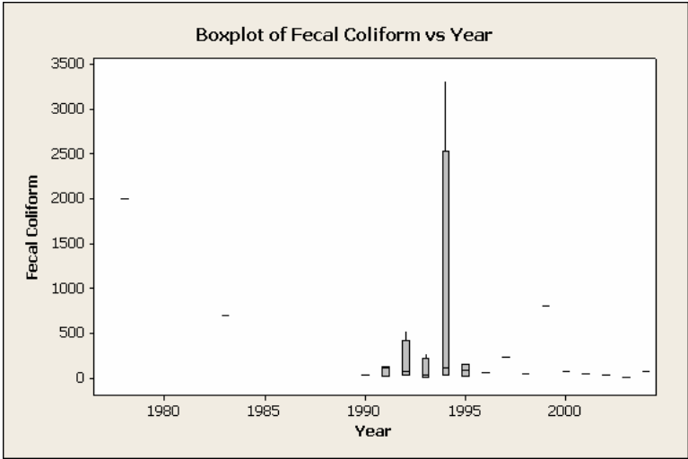
Figure D-3. Box Plot of SSC, TSS, Turbidity, and Fecal Coliform Versus Year for Storet ID 460683.
