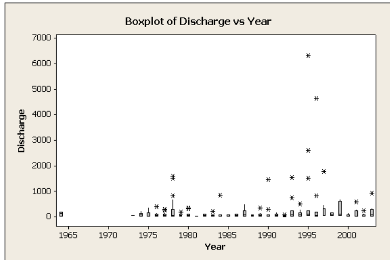
Figure E-4. Box Plot of TDS, SC, and Discharge Versus Year for USGS Site 6428500.
