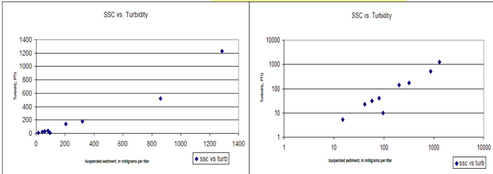
Figure G-6. Horse Creek Water Quality Regression Analysis.
