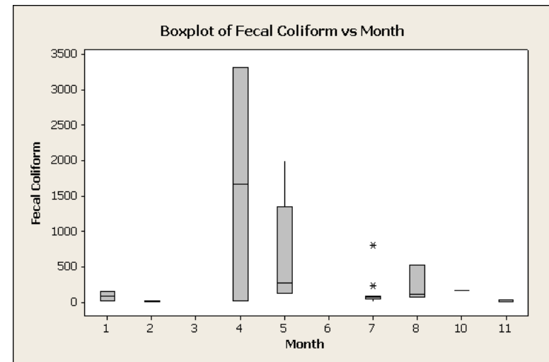
Figure D-1. Box Plot of SSC, TSS, Turbidity, and Fecal Coliform Versus Month for Storet ID 460683.
