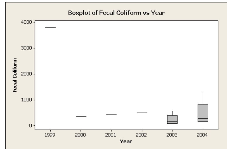
Figure B-3. Box Plot of SSC, TSS, Turbidity, and Fecal Coliform Versus Year for Storet ID 460130.
