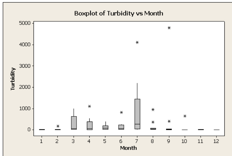
Figure A-3. Box Plot of SSC, TSS, Turbidity, and Fecal Coliform Versus Month for All Sites.
