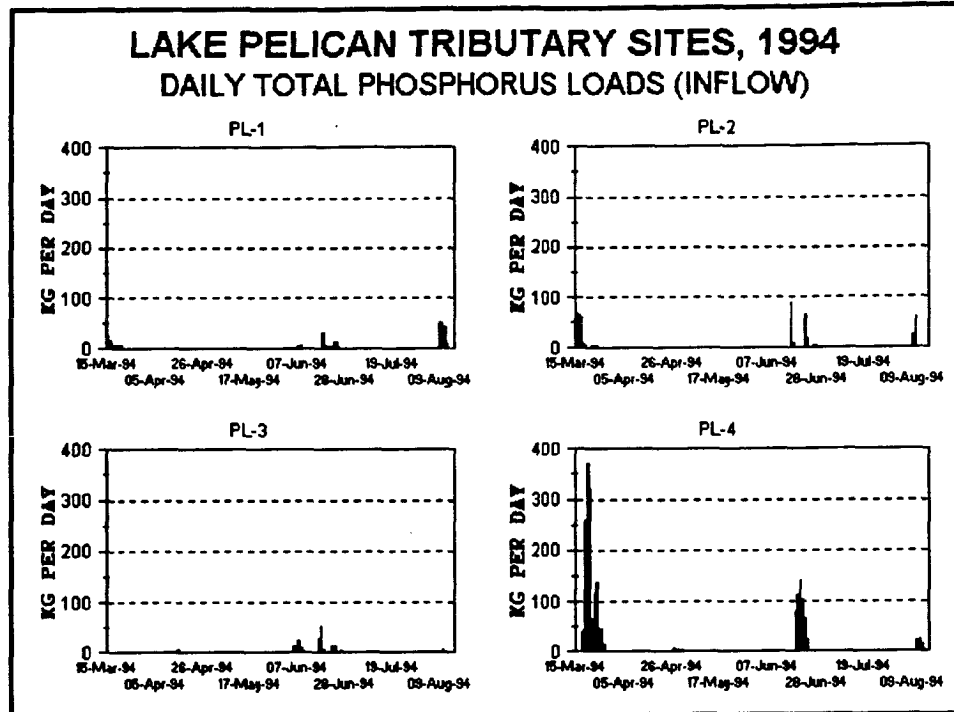
Figure 64. Daily Total Phosphorus Loads (Inflow)
