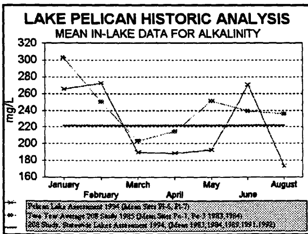
Figure 13. Historic In-Lake Alkalinity
