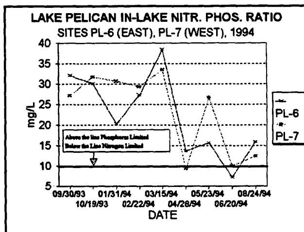
Figure 5. In-Lake N/P Ratio
