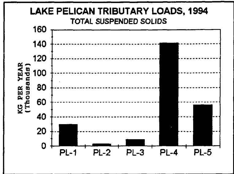
Figure 49. Total Suspended Solids
