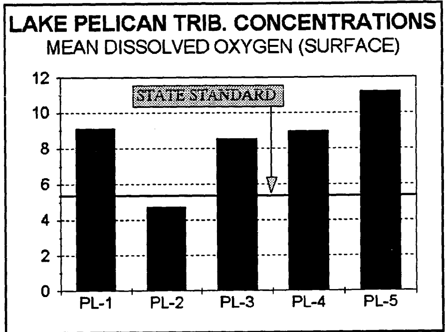
Figure 42. Mean Dissolved Oxygen (Surface)
