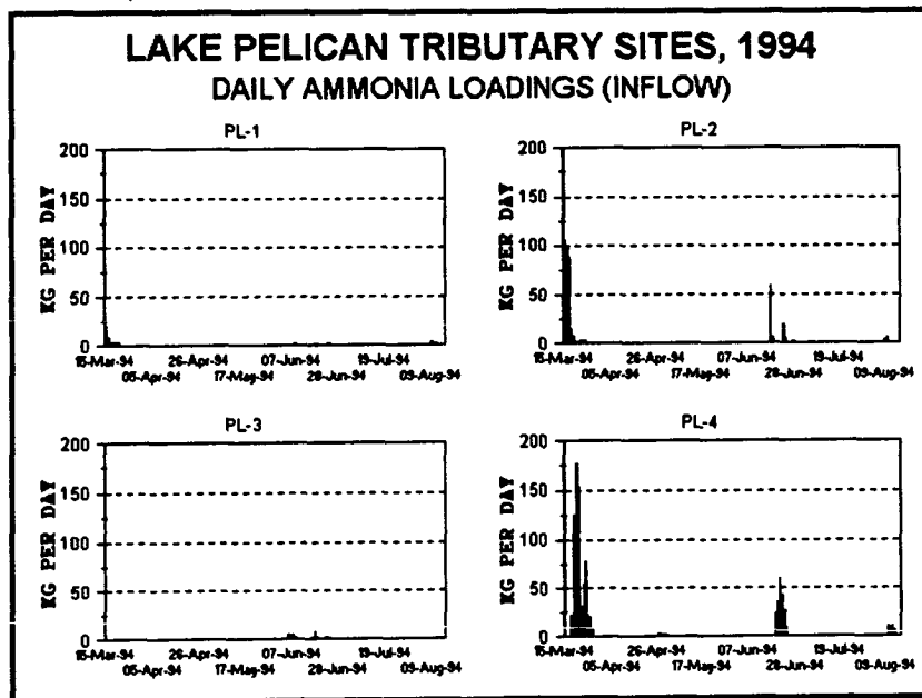
Figure 55. Daily Ammonia Loadings (Inflow)
