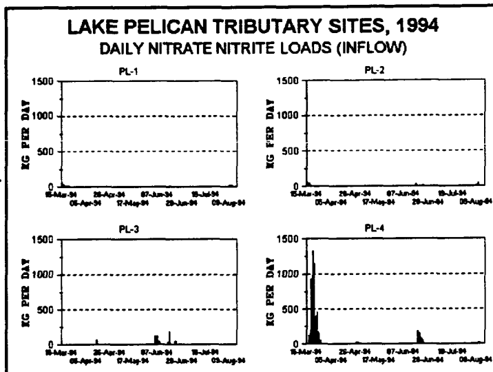
Figure 60. Daily Nitrate Nitrite Loads (Inflow)
