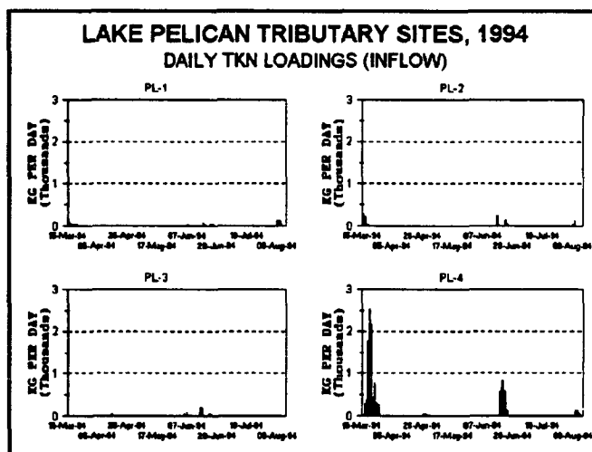
Figure 58. Daily TKN Loadings (Inflow)
