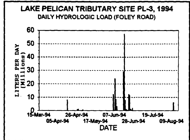
Figure 37. PL-3 Hydrologic Load
