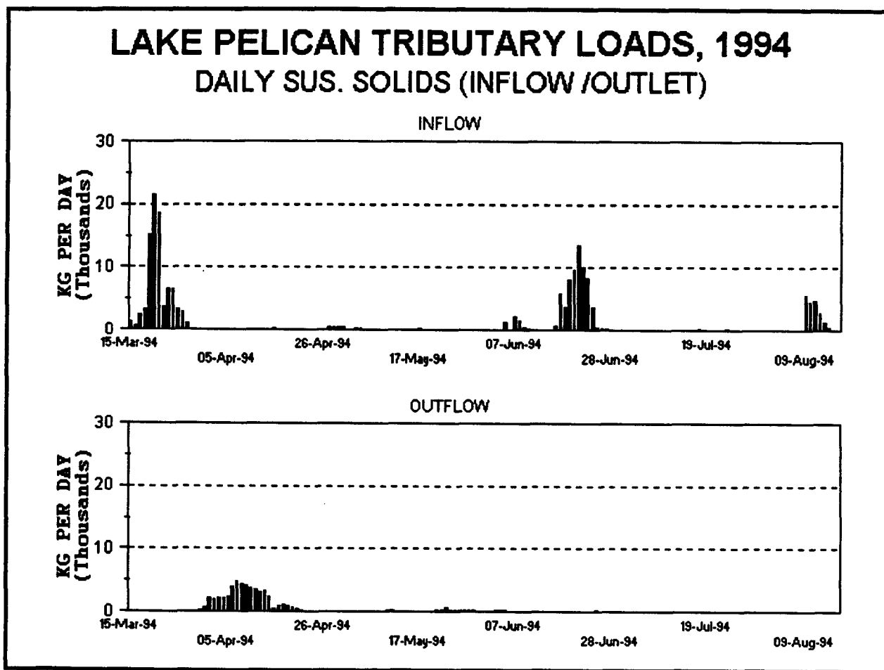
Figure 51. Daily Suspended Solids (Inflow/Outflow)
