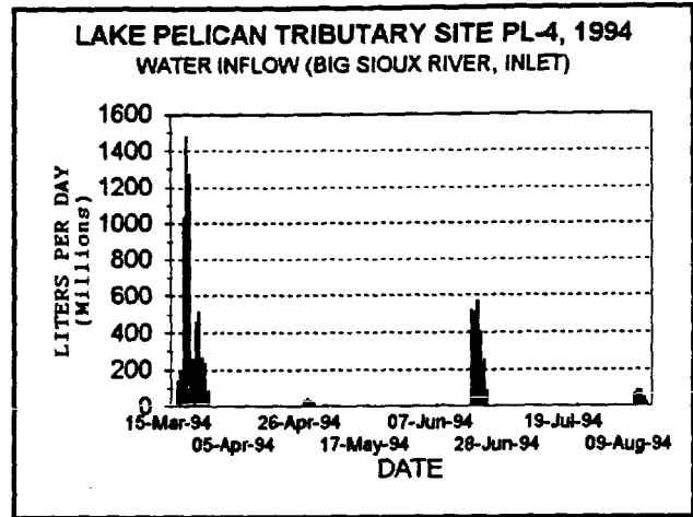
Figure 38. PL-4 Water Inflow
