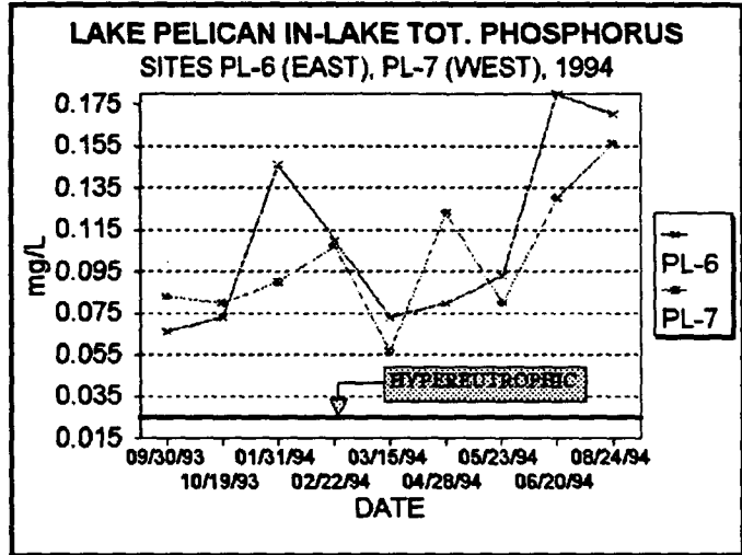
Figure 26. In-Lake Total Phosphorus
