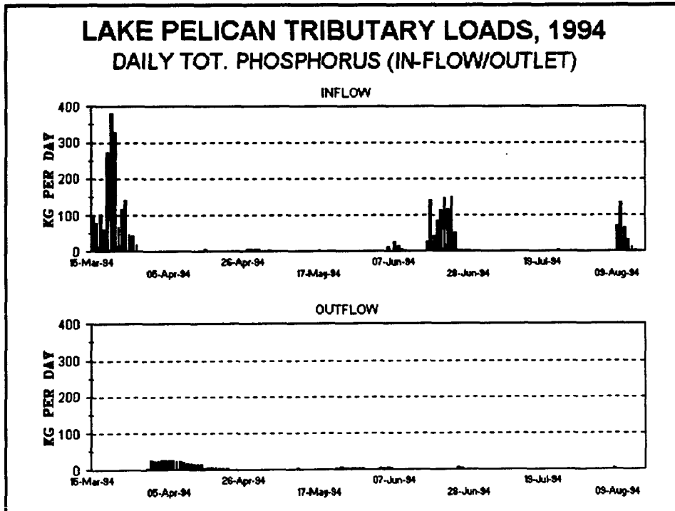
Figure 65. Daily Tot. Phosphorus (Inflow/Outflow)
