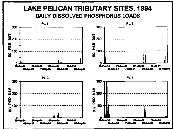
Figure 66. Daily Diss. Phosphorus Loads
