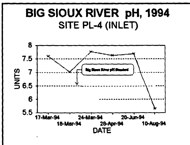
Figure 45. Site PL-4 pH
