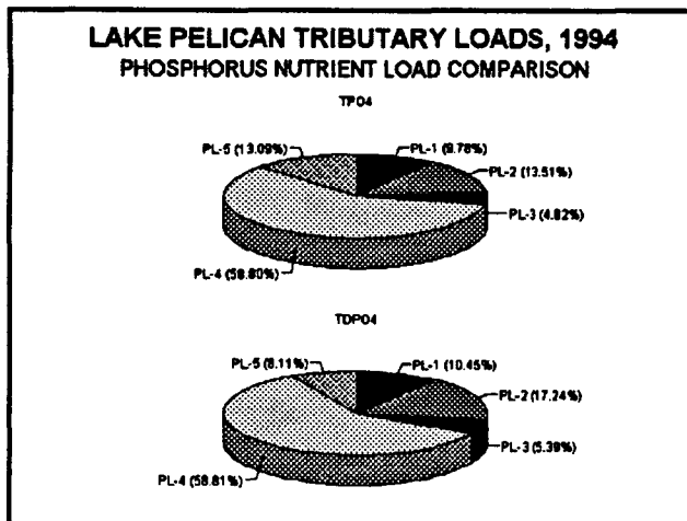
Figure 63. Phosphorus Nutrient Comparison
