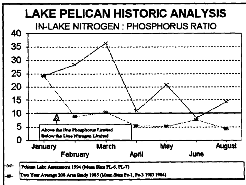
Figure 6. Historic In-Lake N & P Ratio
