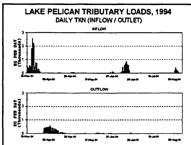
Figure 59. Daily TKN (Inflow/Outflow)
