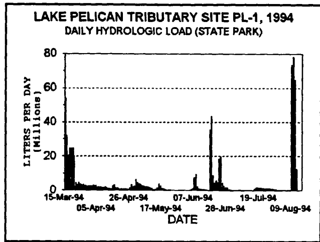
Figure 33. PL-1 Hydrologic Load
