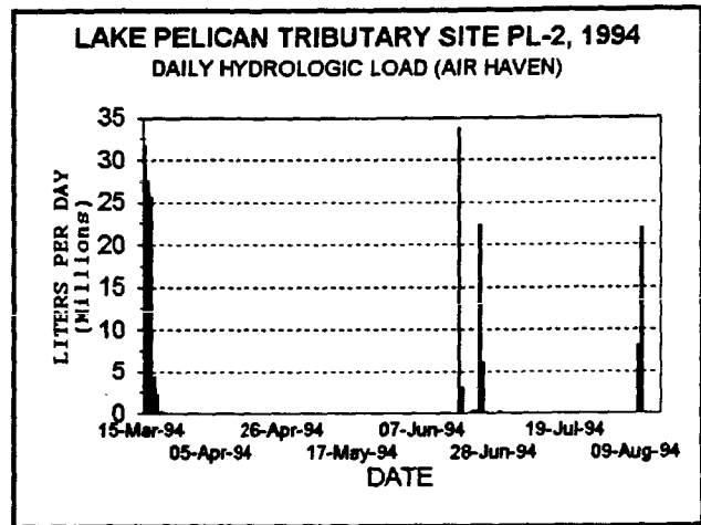
Figure 35. PL-2 Hydrologic Load
