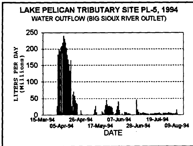
Figure 39. PL-5 Water Outflow
