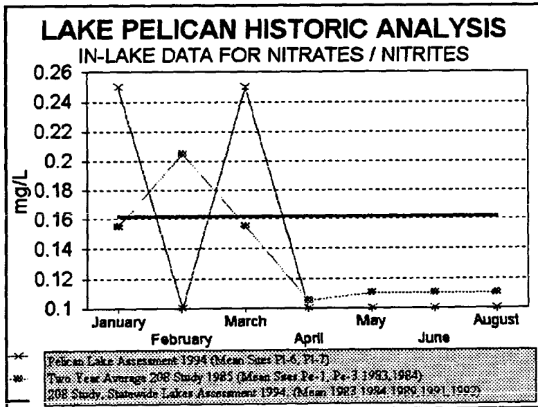
Figure 25. Historic In-Lake Nitrate + Nitrite
