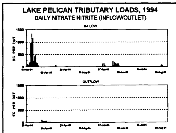
Figure 61. Daily Nitrate Nitrite (Inflow/Outflow)
