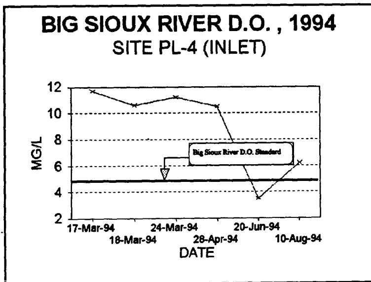
Figure 43. PL-4 (Inlet) Dissolved Oxygen
