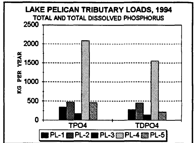
Figure 62. Total and Total Dissolved Phosphorus
