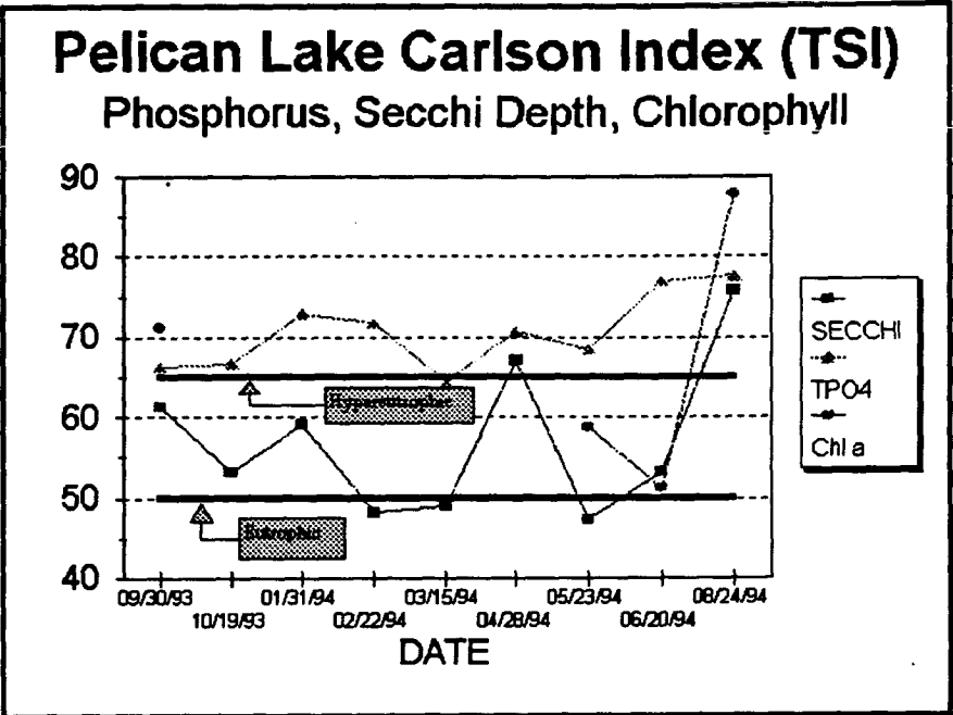
Figure 29. In-Lake Carlson Index
