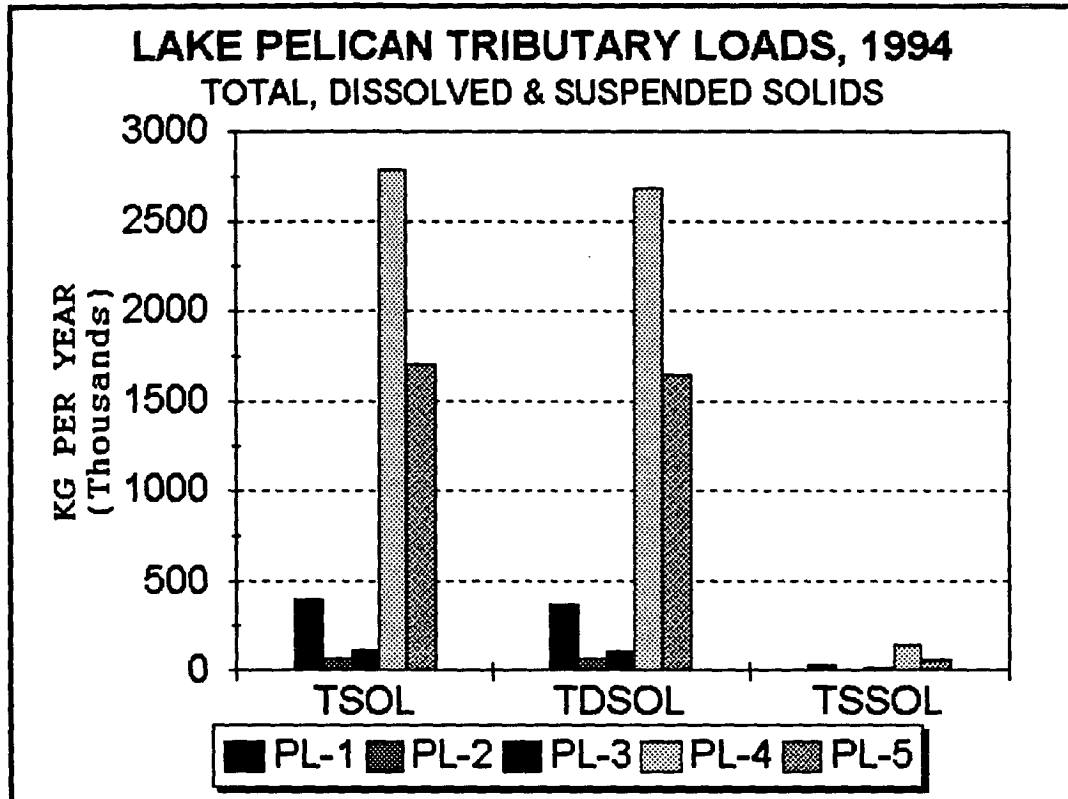
Figure 48. Total, Dissolved & Suspended Solids Loads
