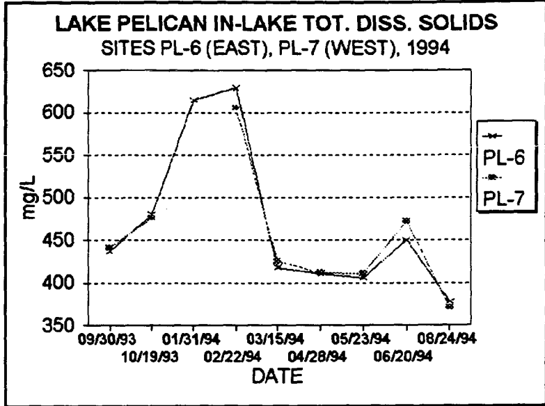
Figure 14. In-Lake Total Dissolved Solids
