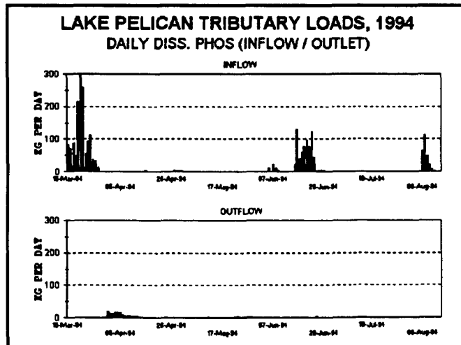
Figure 67. Daily Diss. Phosphorus (Inflow/Outflow)
