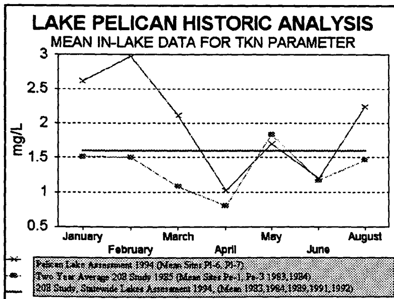
Figure 23. Historic In-Lake TKN
