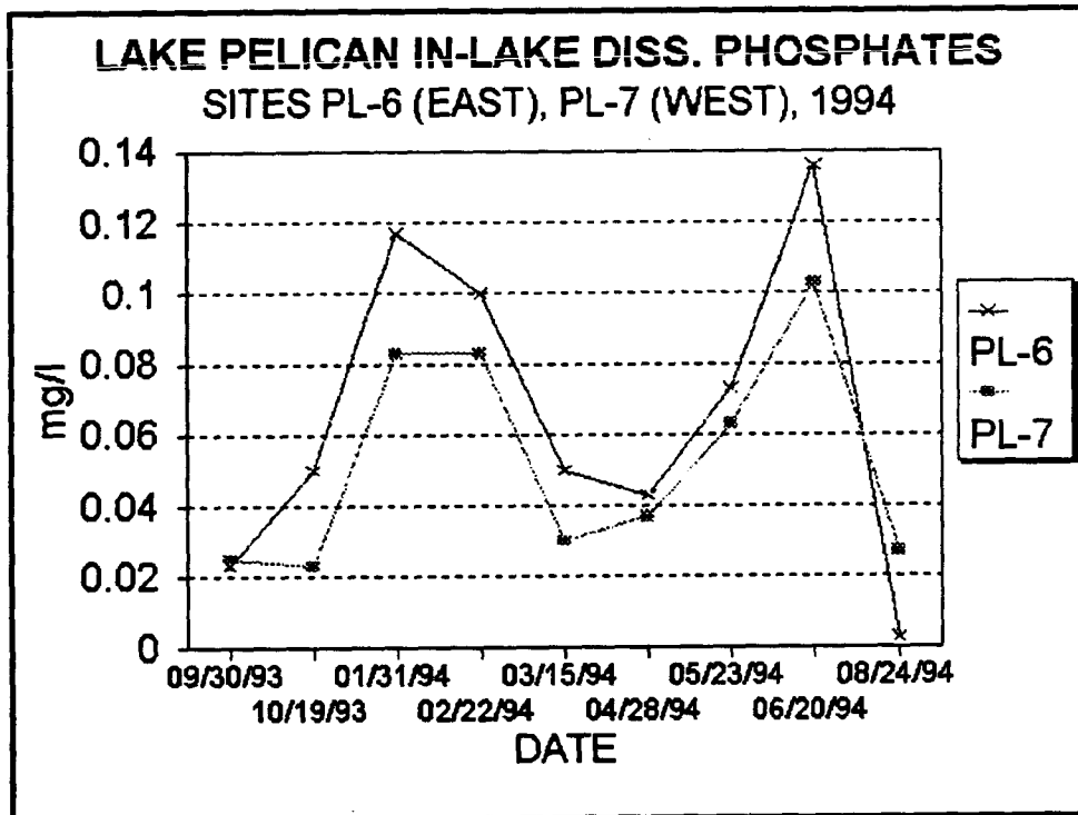
Figure 28. In-Lake Total Dissolved Phosphorus
